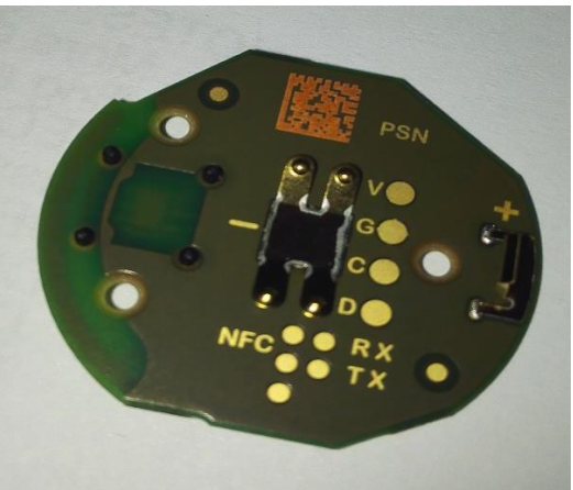
PCB bottom battery side
