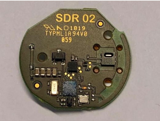
PCB top without shields
