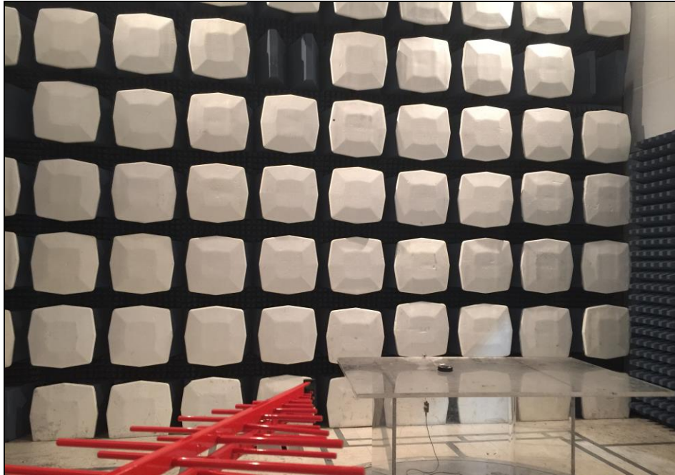
Photograph 1. Radiated Spurious Emissions, Below 1 GHz, Test Setup
