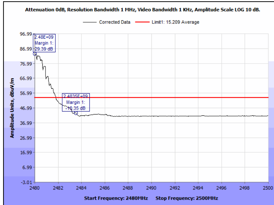
Plot 18. Radiated Restricted Band Edge, High Channel, Average
