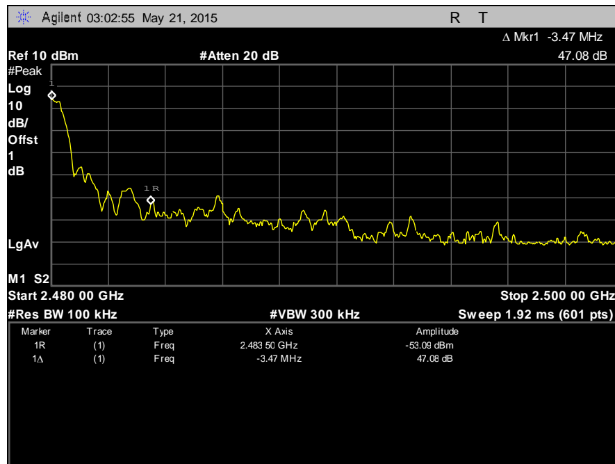
Plot 24. Conducted Band Edge, High Channel
