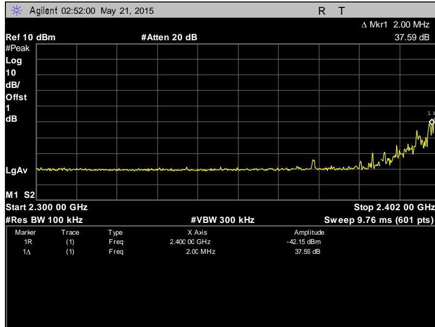
Plot 23. Conducted Band Edge, Low Channel
