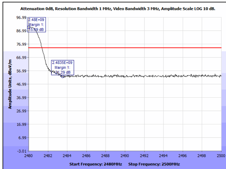
Plot 19. Radiated Restricted Band Edge, High Channel, Peak
