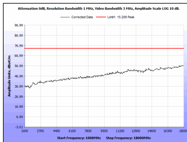
Plot 12. Radiated Spurious Emissions, Mid Channel, 1 GHz – 18 GHz, Peak
