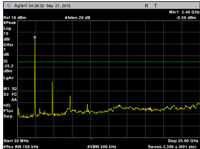
Plot 20. Conducted Spurious Emissions, Low Channel, 30 MHz – 25 GHz
