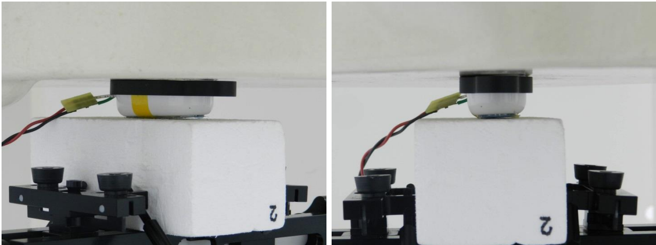
Back with Frame, Test Separation 0 mm
