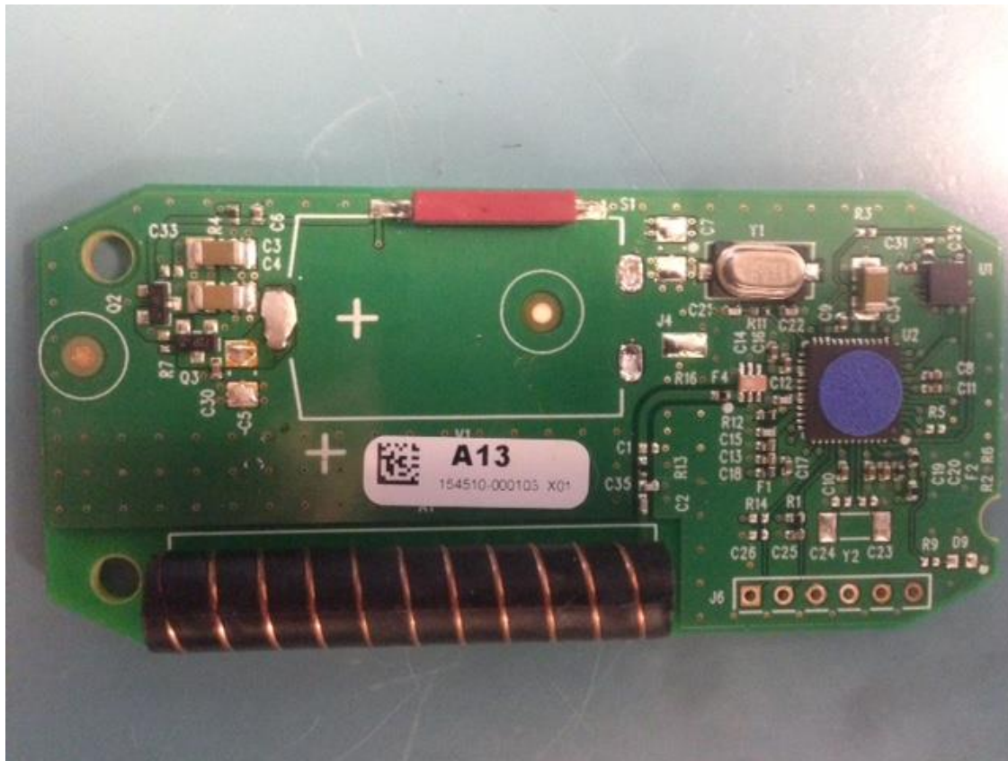
Top with battery removed
