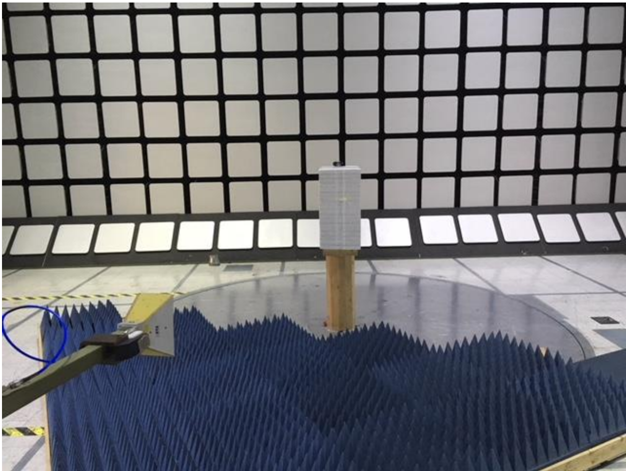
Test setup for 1 – 5 GHz
