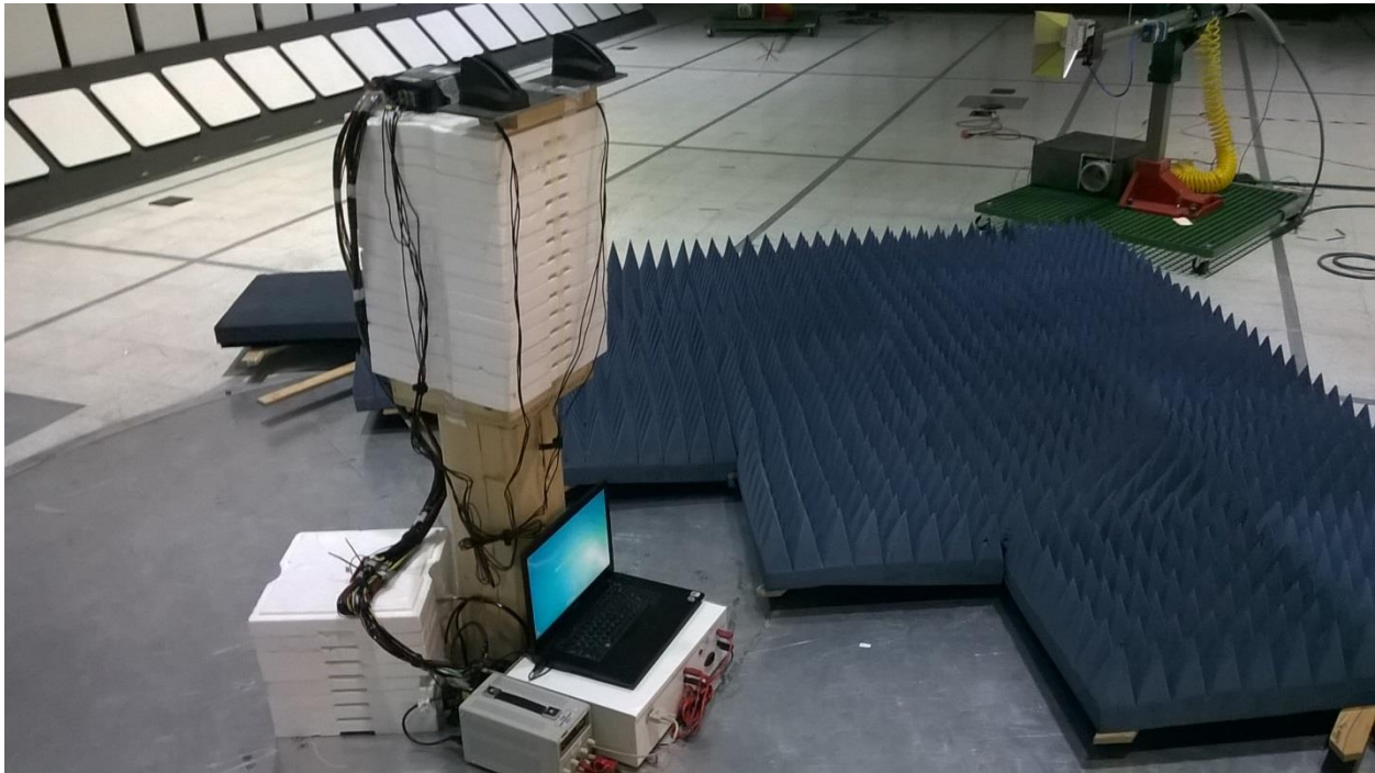
Figure 3 - Radiated emissions, 1 – 18GHz
