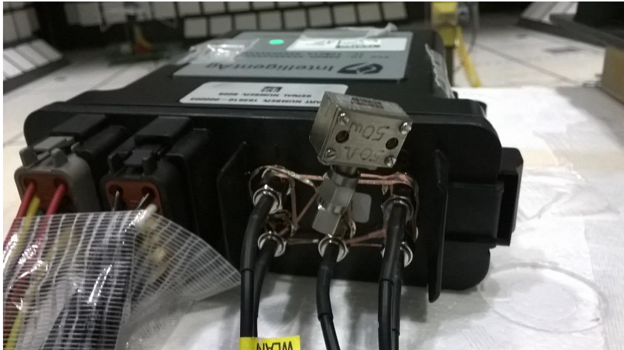
Figure 4 - 50 ohm load used for radiated spurious emissions test on the satellite communications radio
