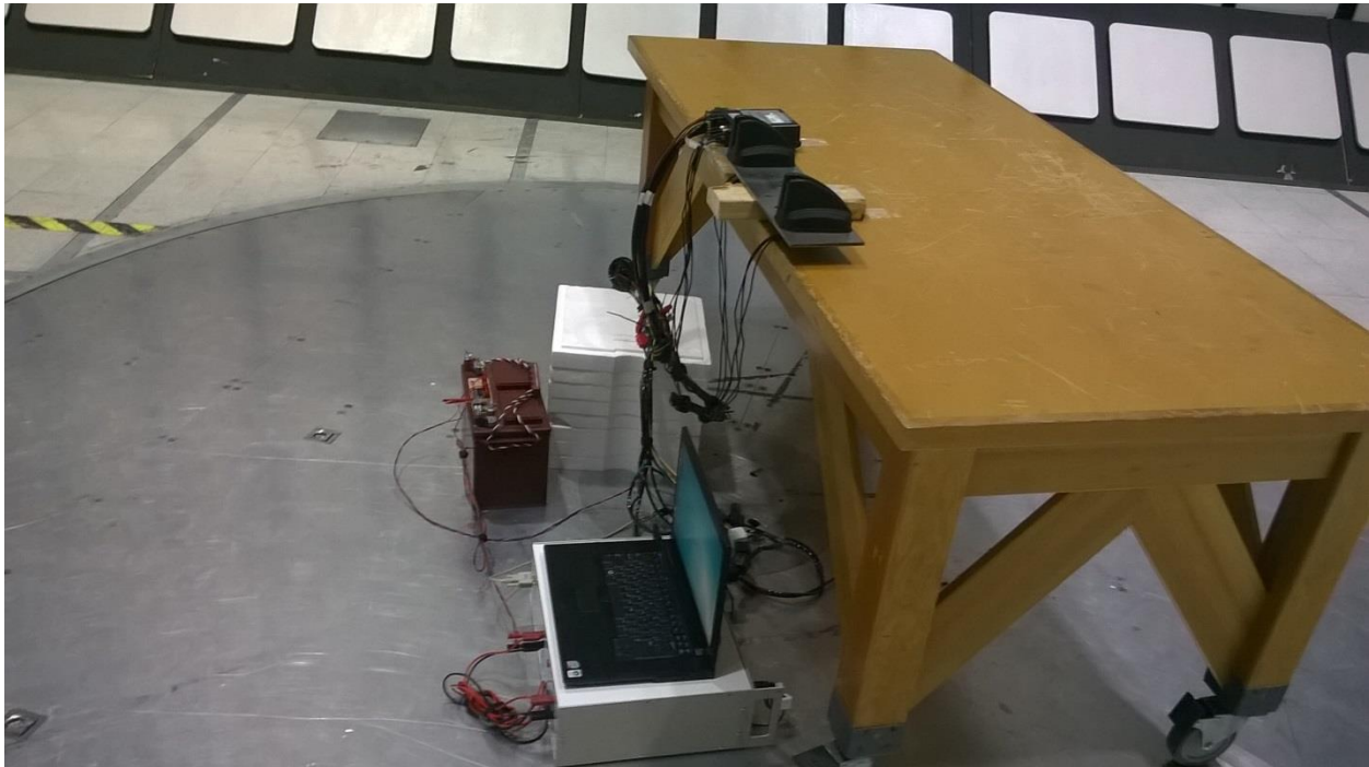
Figure 1 - Radiated emissions, 30MHz - 1GHz
