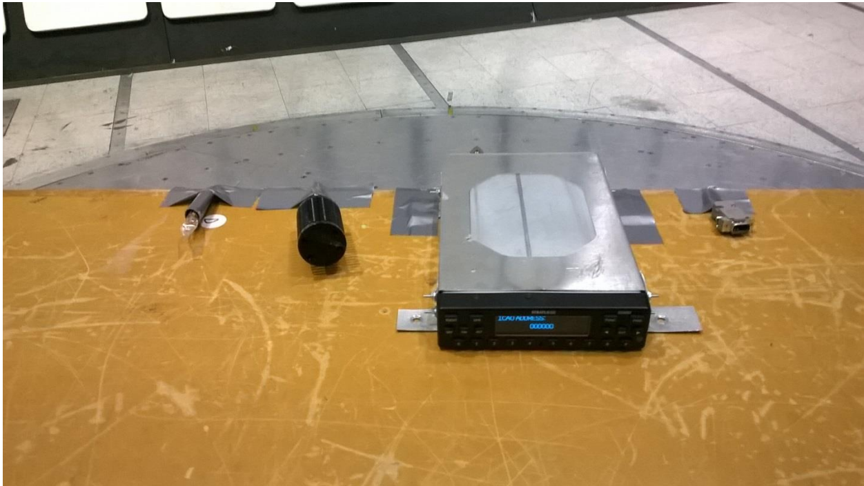
Figure 4 - Test Setup Photo, 30MHz - 1GHz
