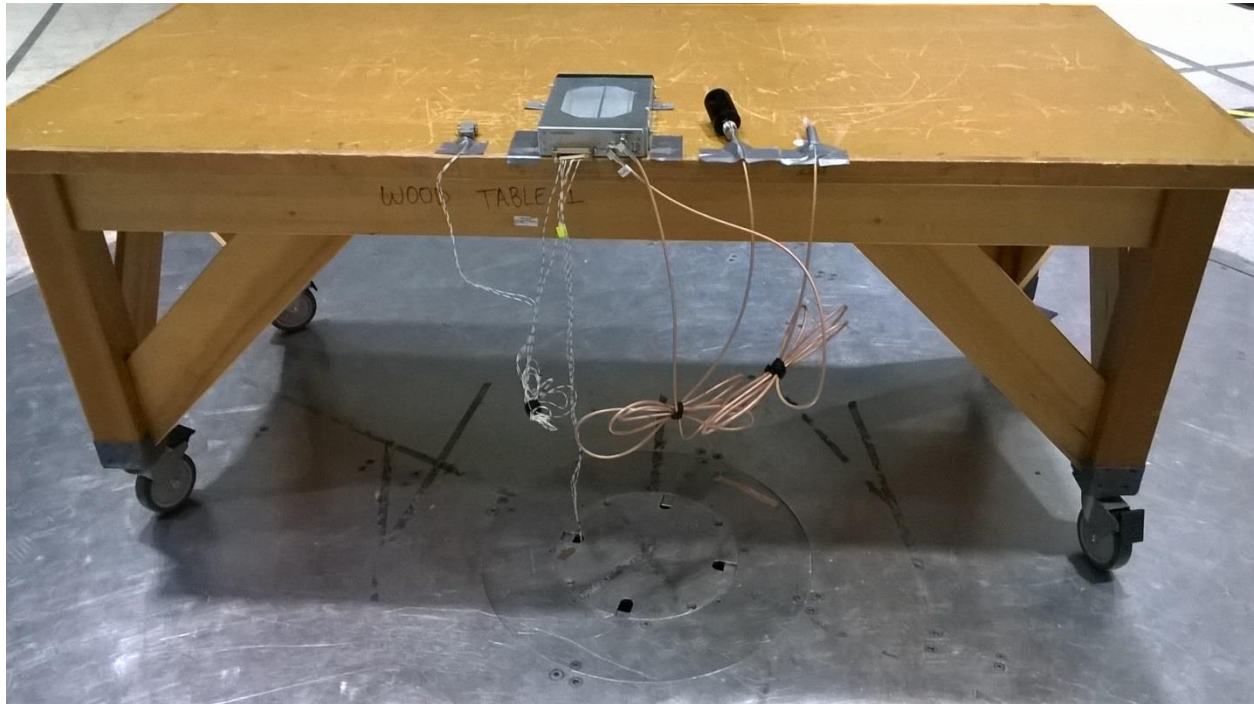
Figure 3 - Test Setup Photo, 30MHz - 1GHz
