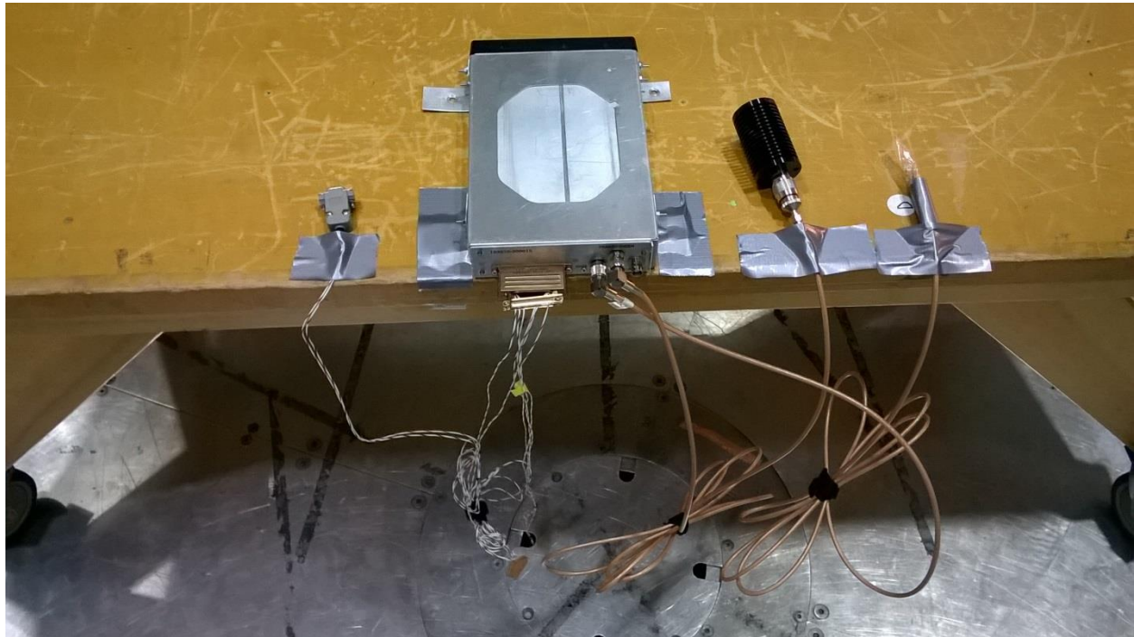
Figure 2 - Test Setup Photo, 30MHz - 1GHz
