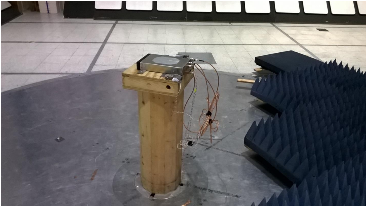
Figure 1 - Test Setup Photo - 1GHz - 12GHz
