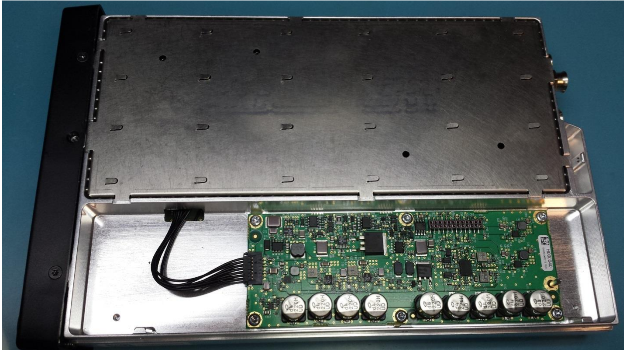
Figure 6 - Power and transmit cavity with TX cover on
