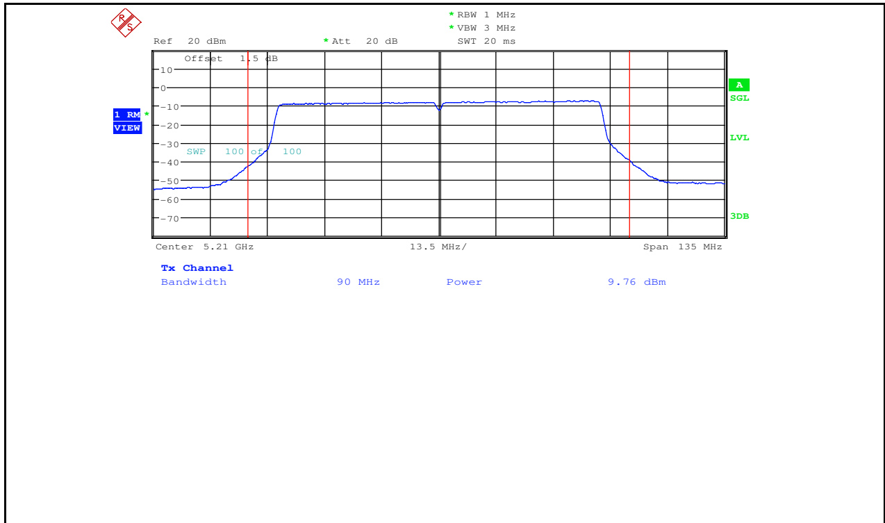
Maximum Conduct Output Power_11AC80_5210_Ant2
