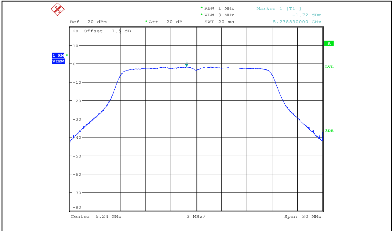
Maximum Power Spectral Density_TNVN_11N20_5240_Ant2
