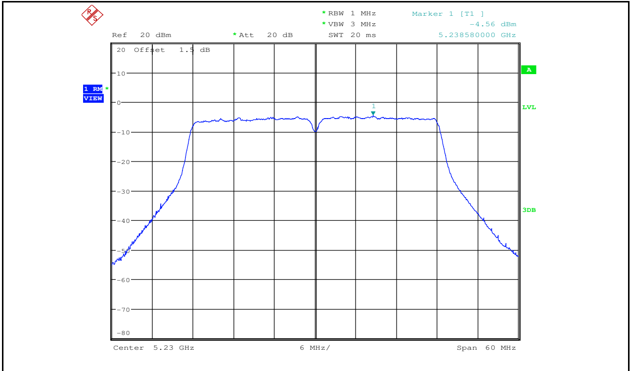
Maximum Power Spectral Density_TNVN_11AC40_5230_Ant2
