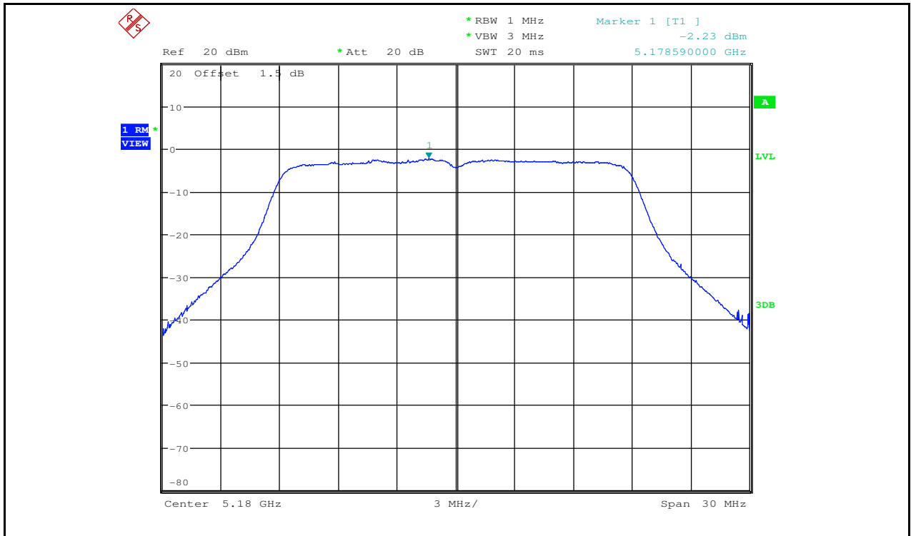
Maximum Power Spectral Density_TNVN_11AC20_5180_Ant2
