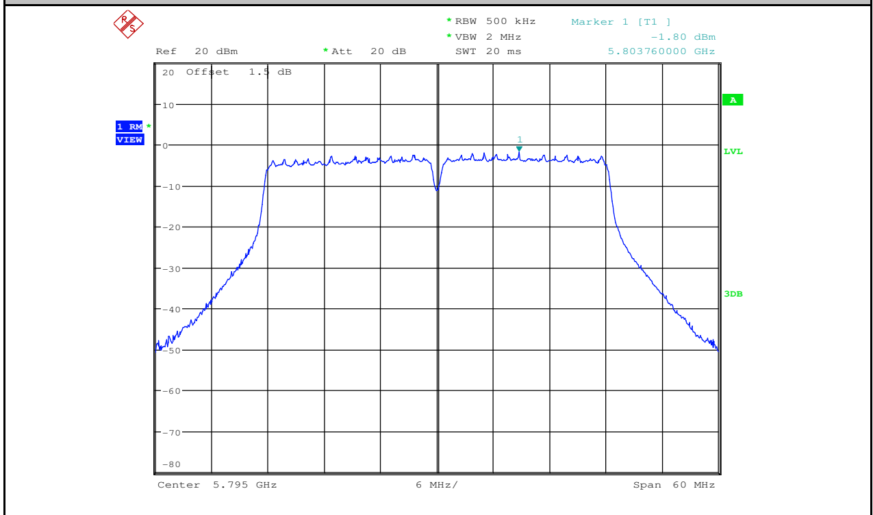
Maximum Power Spectral Density_TNVN_11AC40_5795_Ant2
