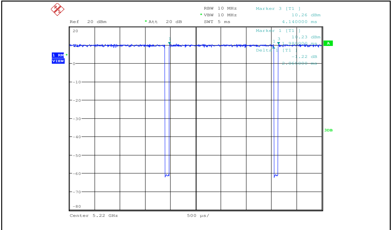
Duty Cycle_11A_5220_Ant2
