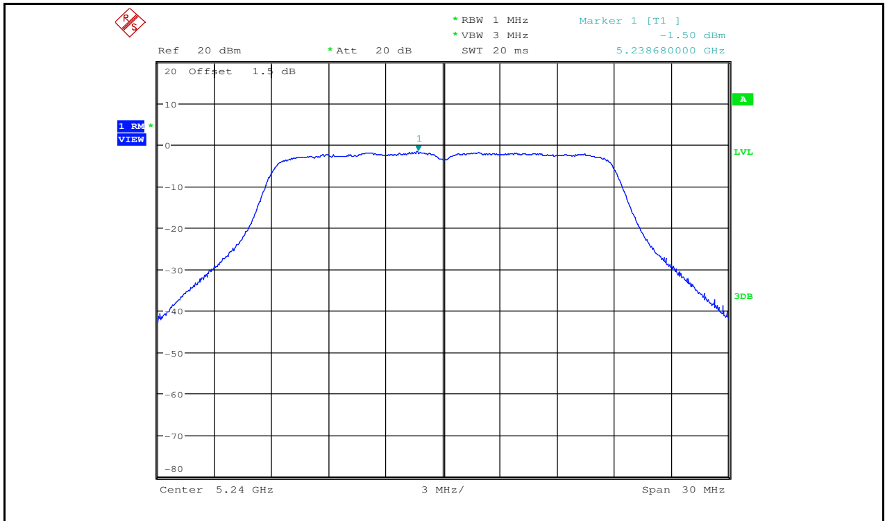
Maximum Power Spectral Density_TNVN_11AC20_5240_Ant2
