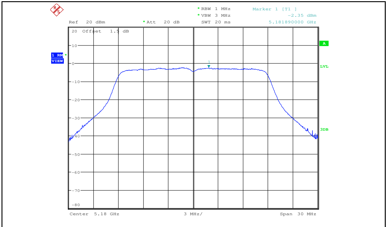
Maximum Power Spectral Density_TNVN_11N20_5180_Ant2
