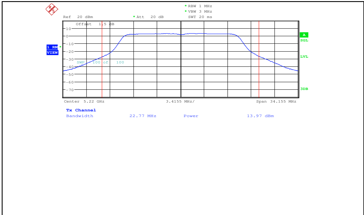
Maximum Conduct Output Power_11A_5220_Ant2
