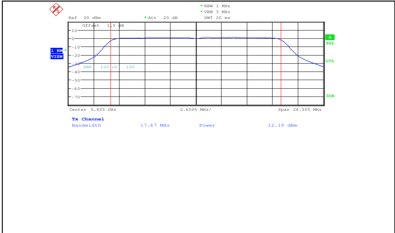
Maximum Conduct Output Power_11AC20_5825_Ant2
