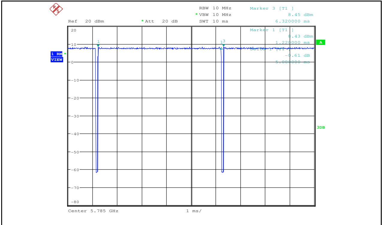
Duty Cycle_11N20_5785_Ant2
