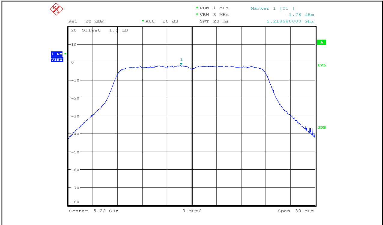
Maximum Power Spectral Density_TNVN_11N20_5220_Ant2
