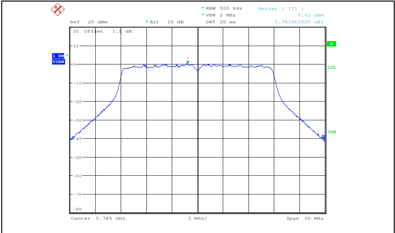
Maximum Power Spectral Density_TNVN_11N20_5785_Ant2
