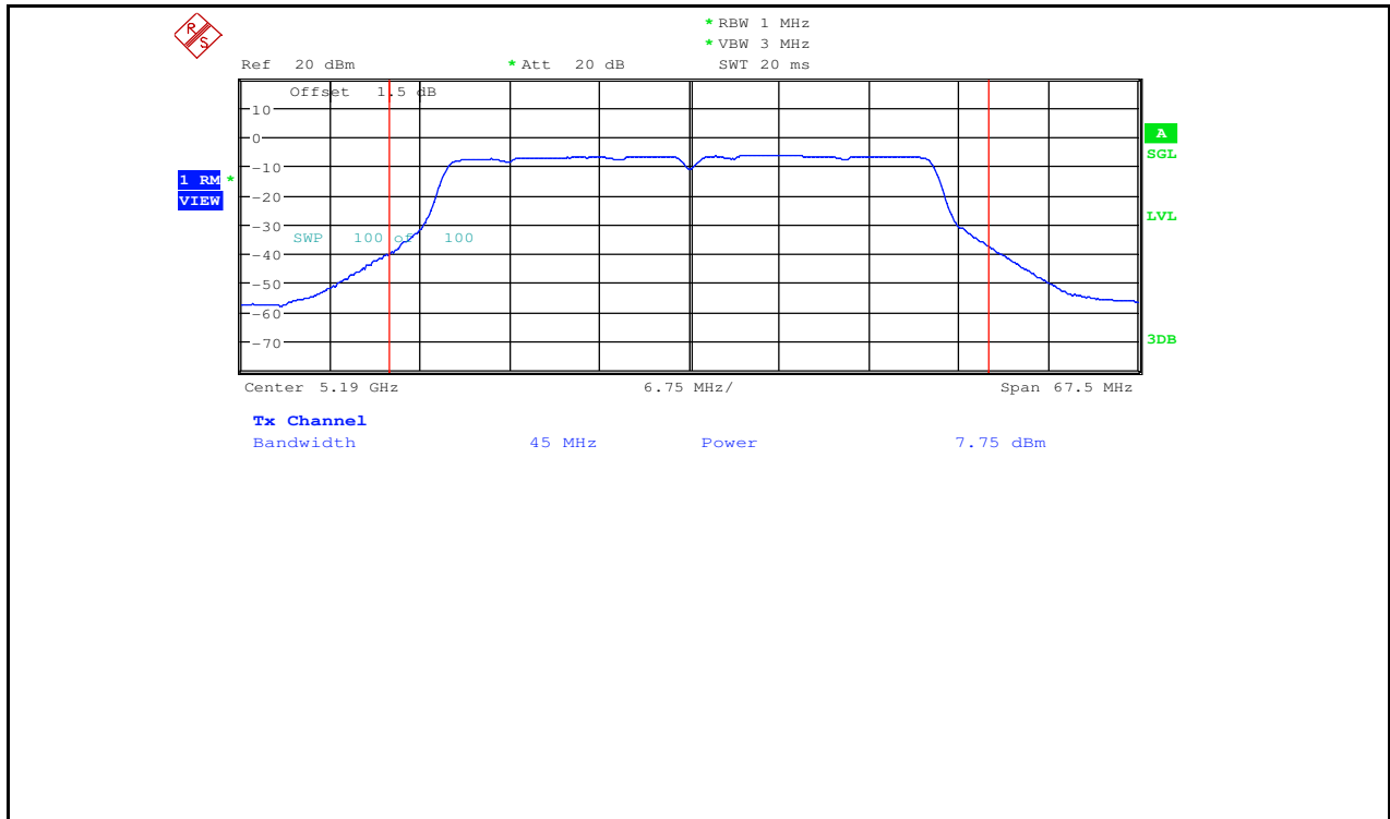
Maximum Conduct Output Power_11N40_5190_Ant2
