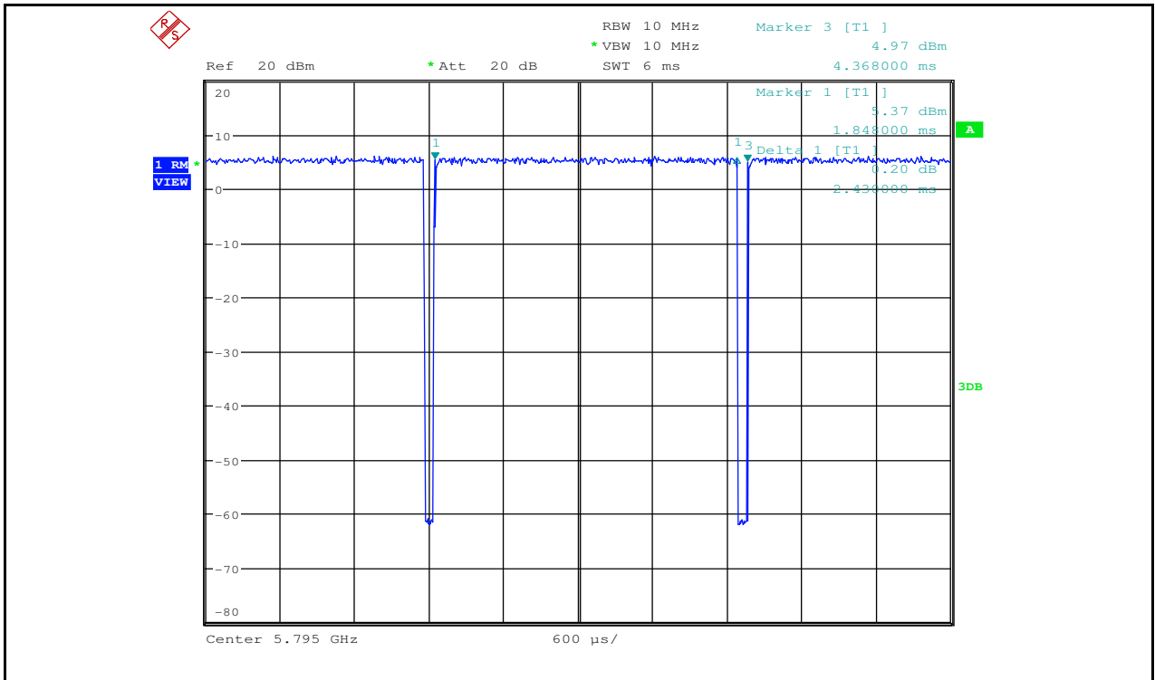
Duty Cycle_11N40_5795_Ant2
