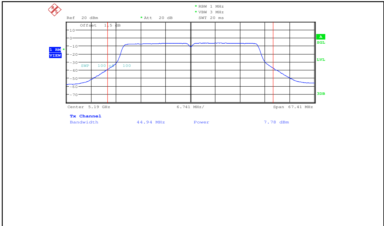
Maximum Conduct Output Power_11AC40_5190_Ant2
