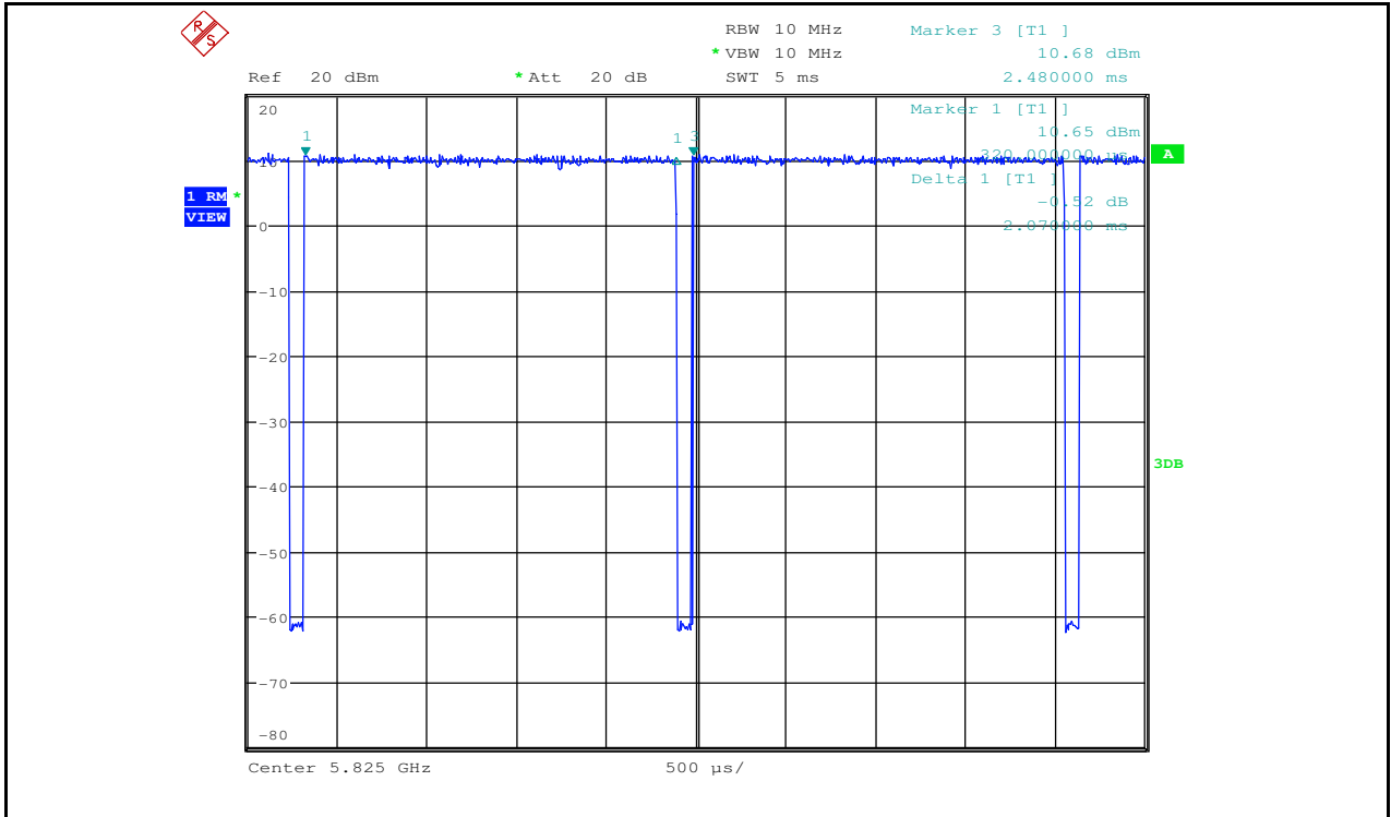
Duty Cycle_11A_5825_Ant2
