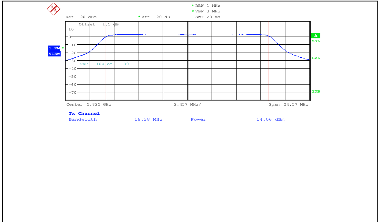
Maximum Conduct Output Power_11A_5825_Ant2
