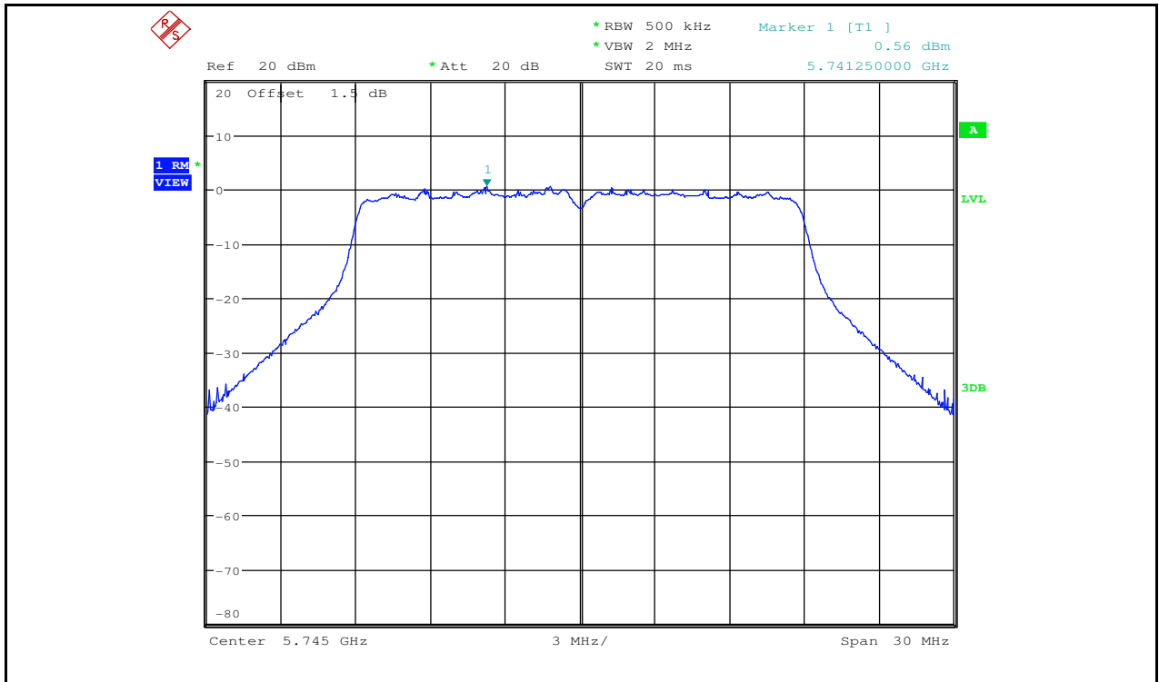
Maximum Power Spectral Density_TNVN_11N20_5745_Ant2
