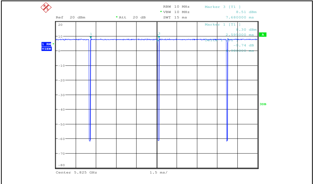
Duty Cycle_11AC20_5825_Ant2
