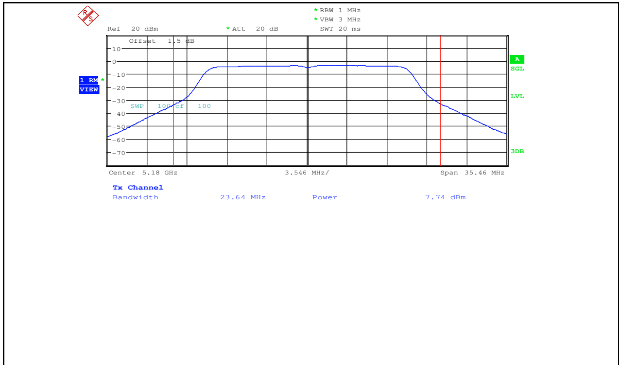
Maximum Conduct Output Power_11AC20_5180_Ant2
