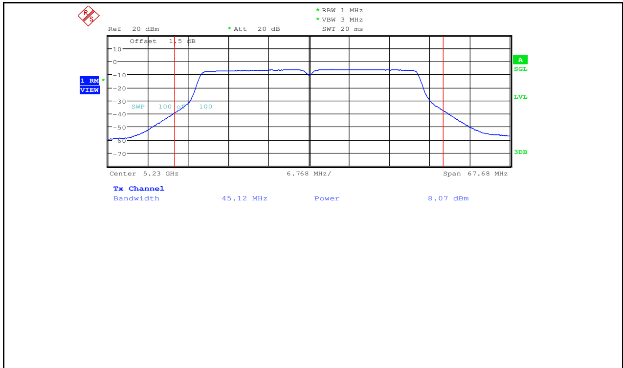
Maximum Conduct Output Power_11N40_5230_Ant2
