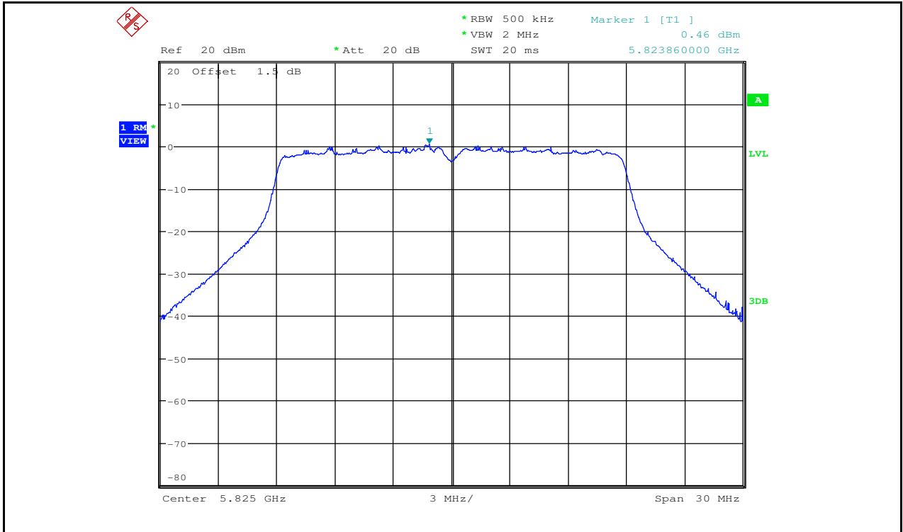
Maximum Power Spectral Density_TNVN_11N20_5825_Ant2
