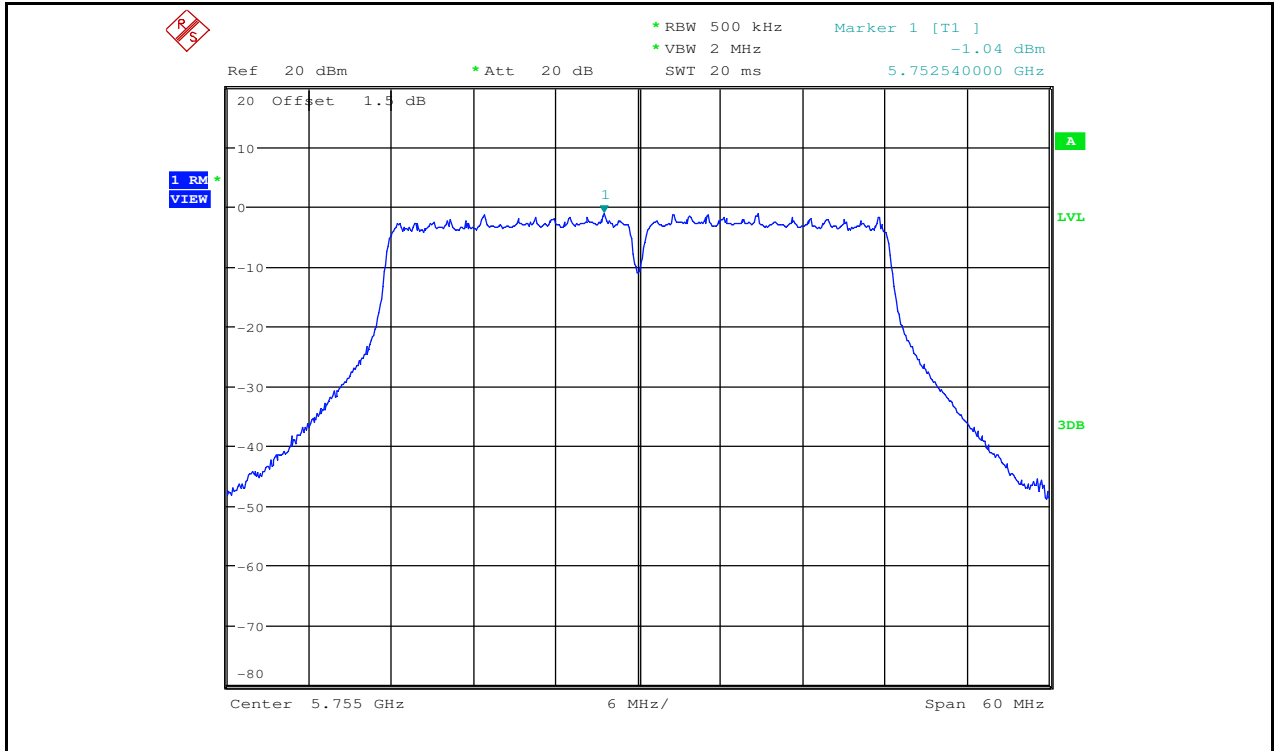
Maximum Power Spectral Density_TNVN_11AC40_5755_Ant2
