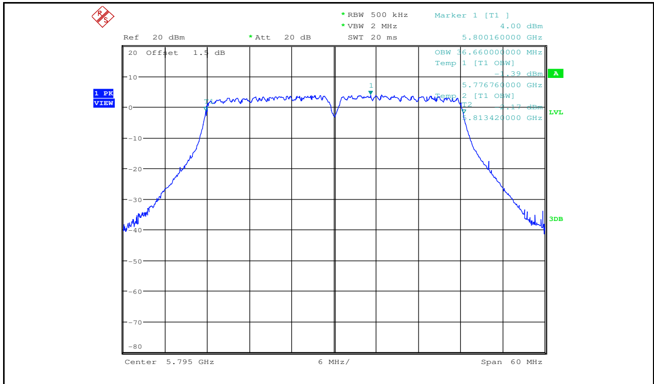
Occupied Bandwidth Measurement_11AC40_5795_Ant2
