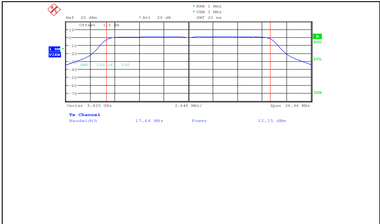
Maximum Conduct Output Power_11N20_5825_Ant2
