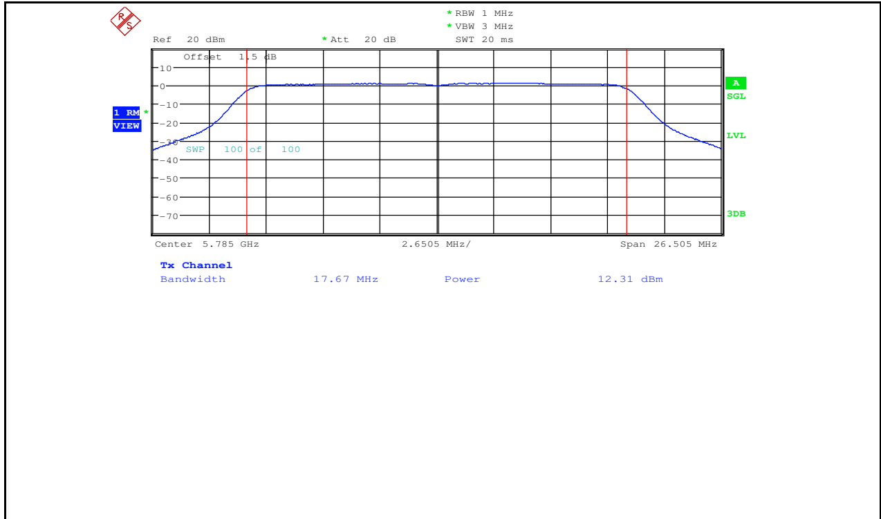
Maximum Conduct Output Power_11AC20_5785_Ant2
