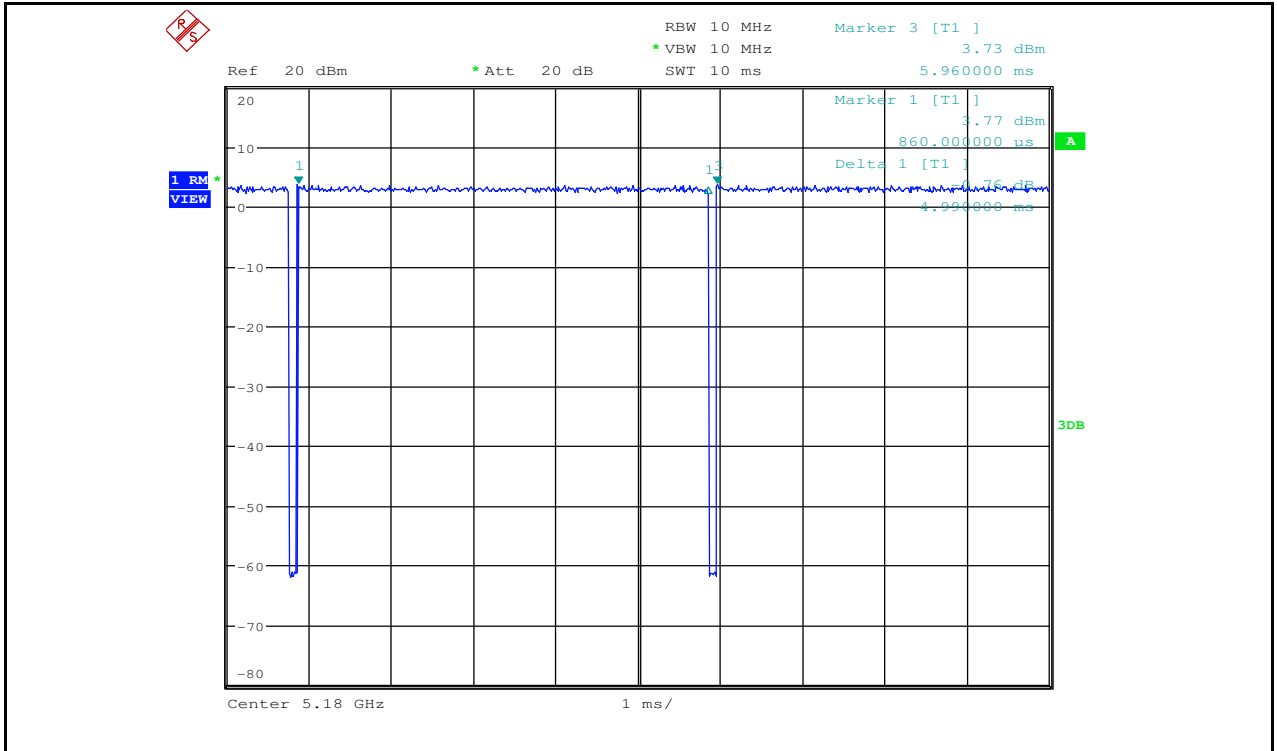
Duty Cycle_11N20_5180_Ant2
