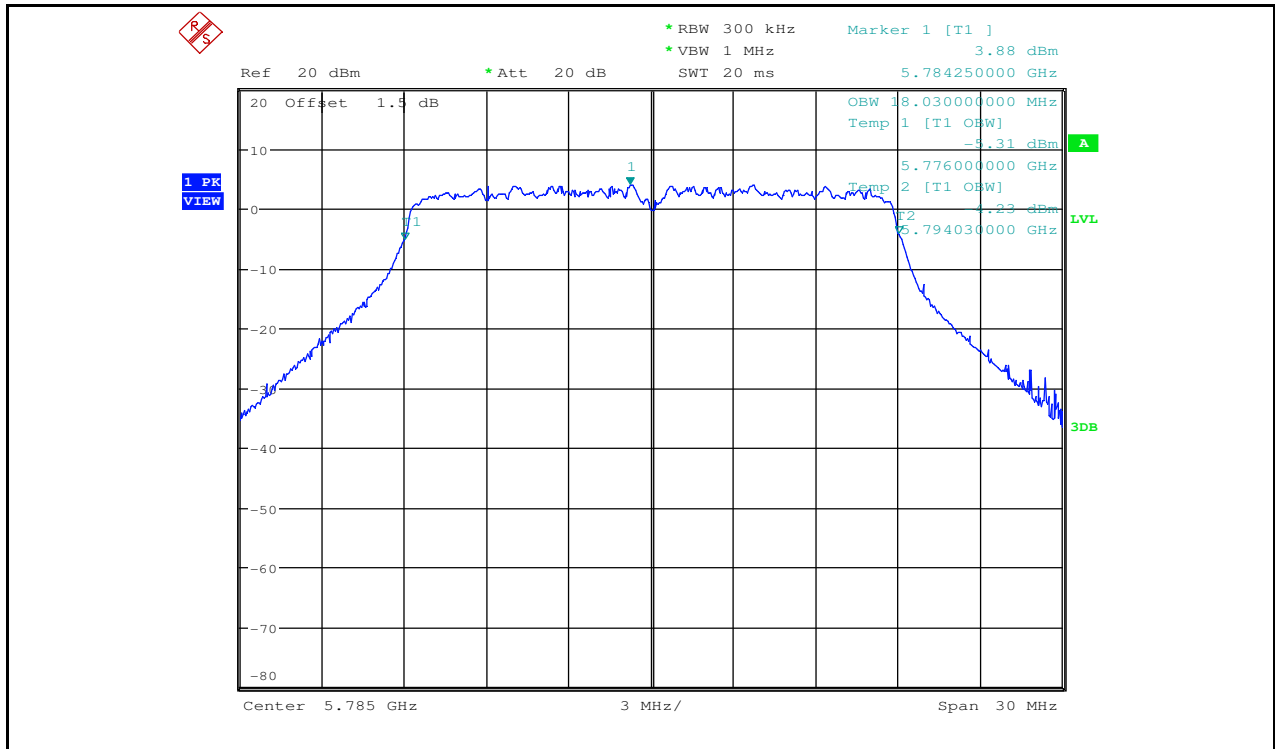
Occupied Bandwidth Measurement_11AC20_5785_Ant2
