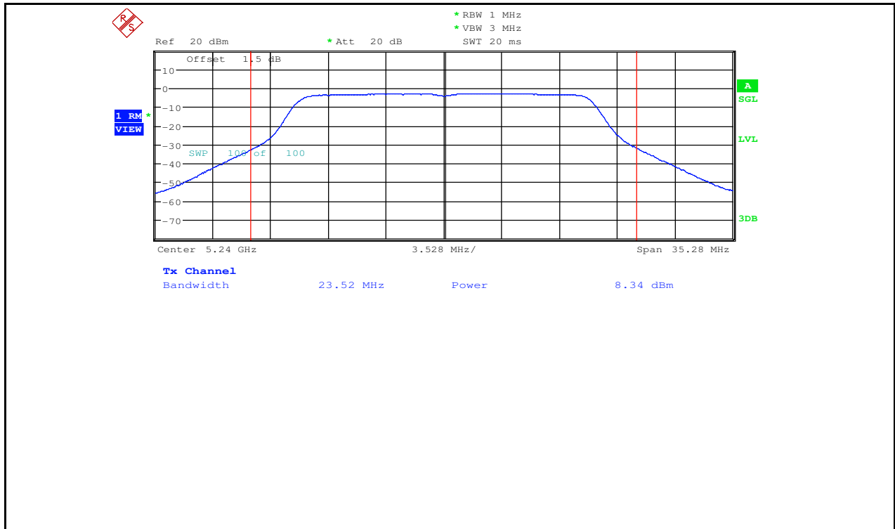
Maximum Conduct Output Power_11N20_5240_Ant2
