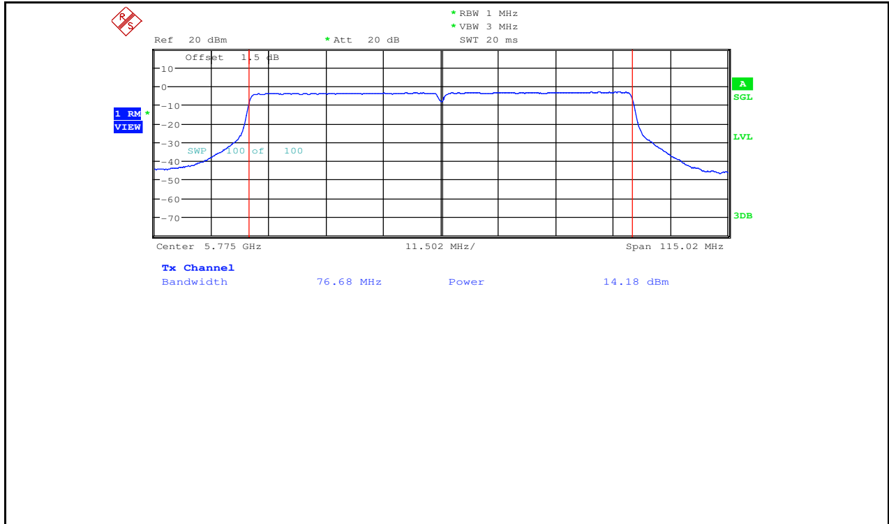
Maximum Conduct Output Power_11AC80_5775_Ant2
