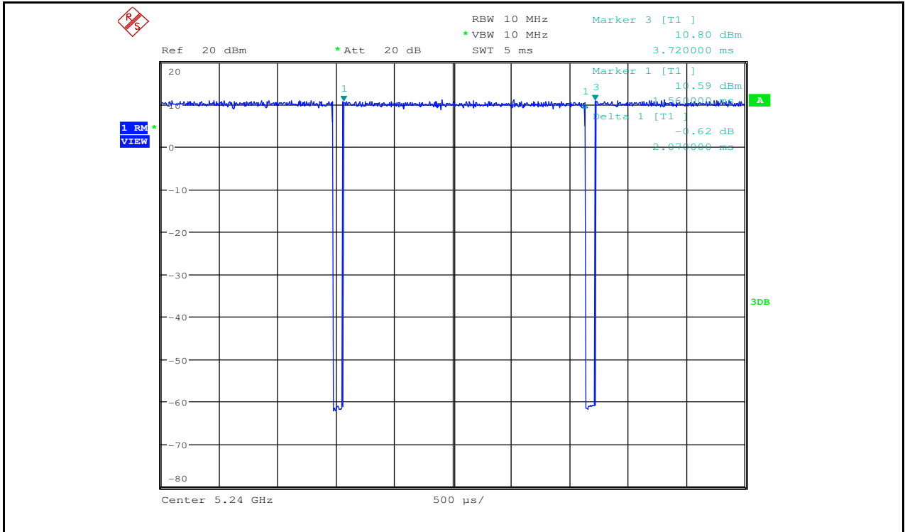
Duty Cycle_11A_5240_Ant2
