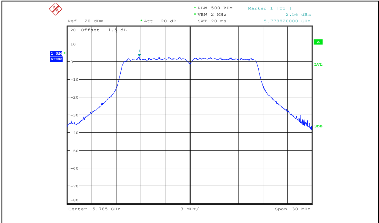
Maximum Power Spectral Density_TNVN_11A_5785_Ant2
