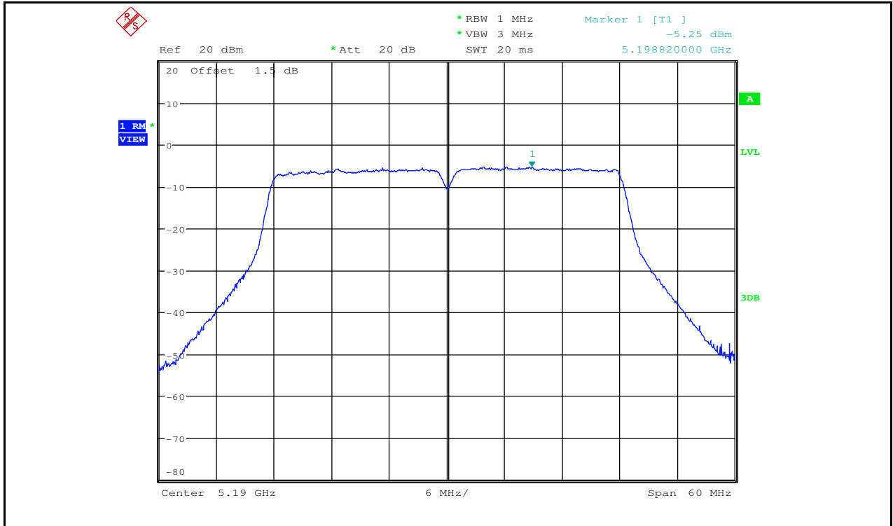
Maximum Power Spectral Density_TNVN_11N40_5190_Ant2
