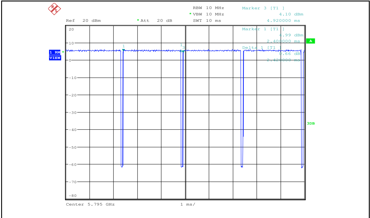
Duty Cycle_11AC40_5795_Ant2
