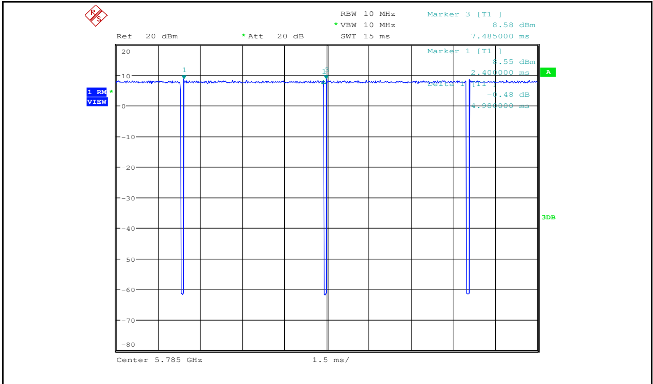
Duty Cycle_11AC20_5785_Ant2
