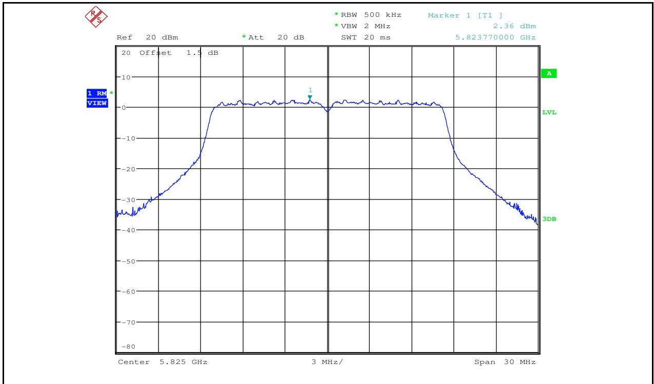
Maximum Power Spectral Density_TNVN_11A_5825_Ant2
