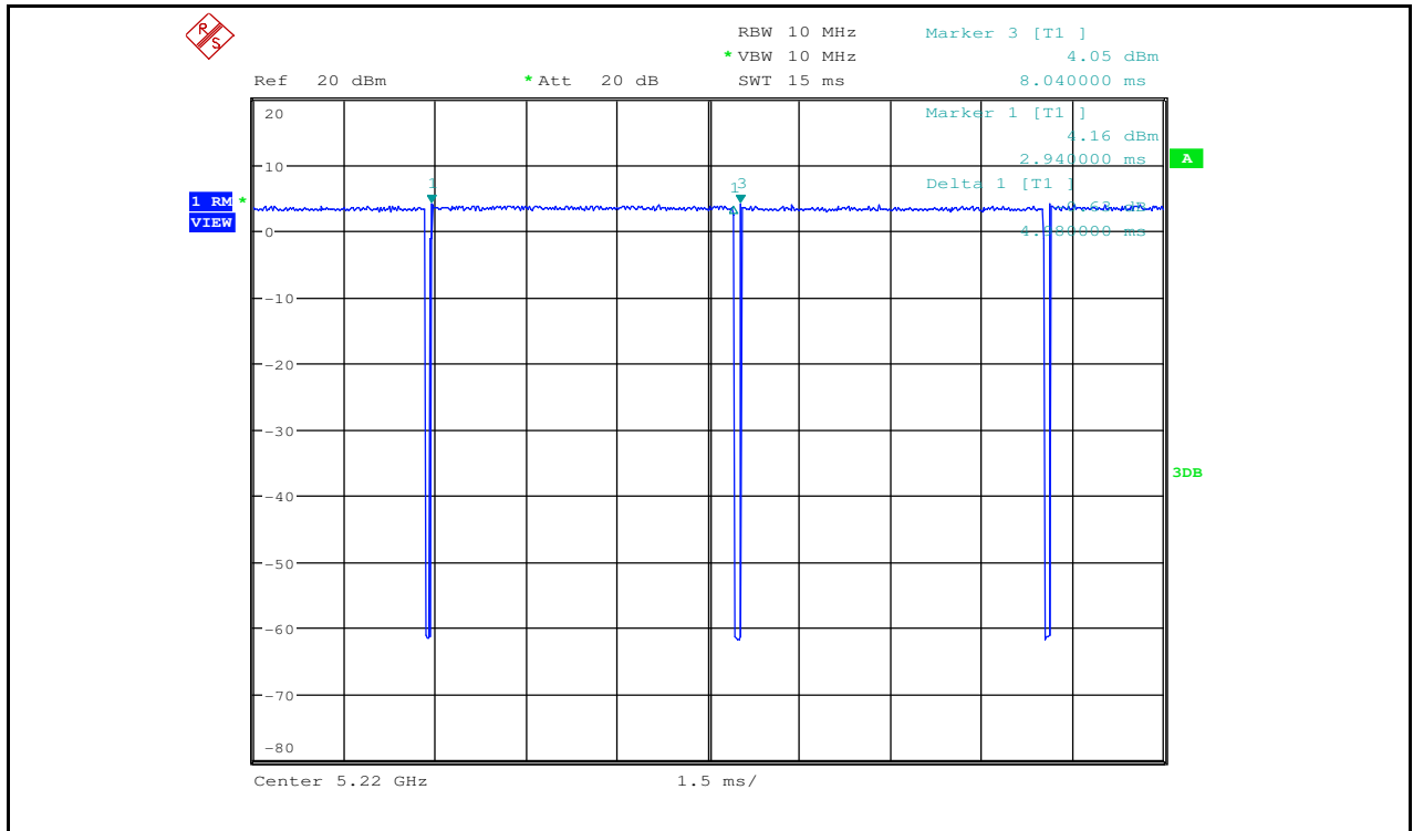
Duty Cycle_11AC20_5220_Ant2
