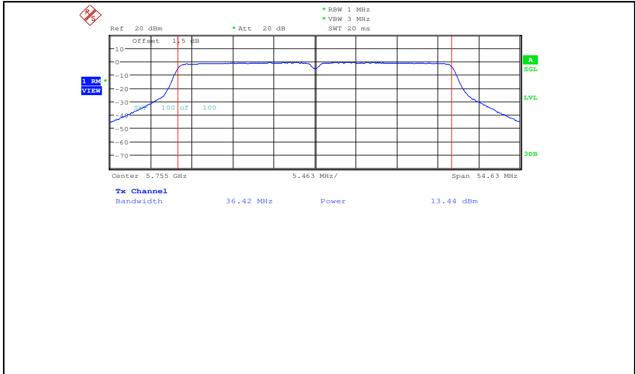
Maximum Conduct Output Power_11AC40_5755_Ant2
