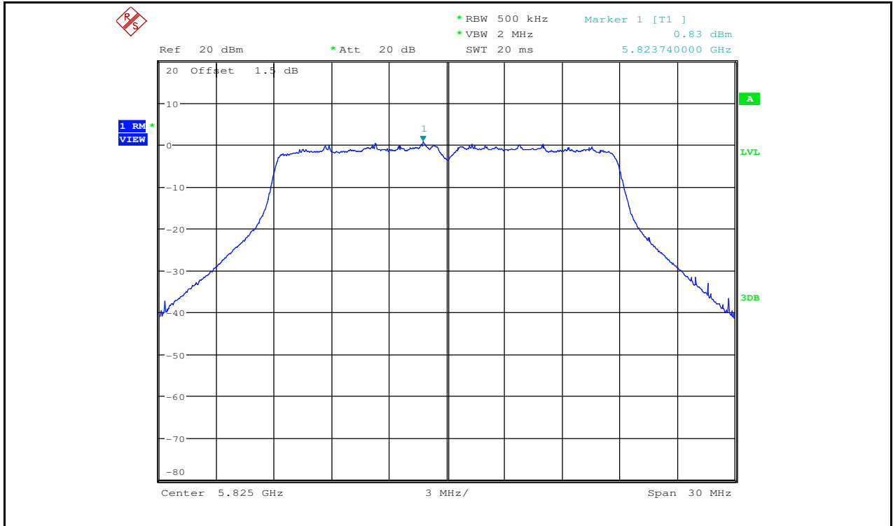
Maximum Power Spectral Density_TNVN_11AC20_5825_Ant2
