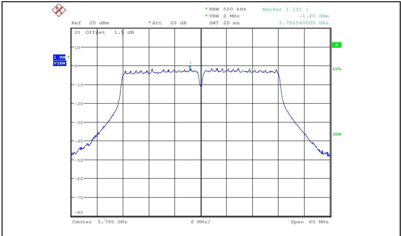
Maximum Power Spectral Density_TNVN_11N40_5795_Ant2
