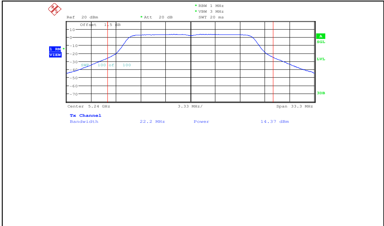
Maximum Conduct Output Power_11A_5240_Ant2
