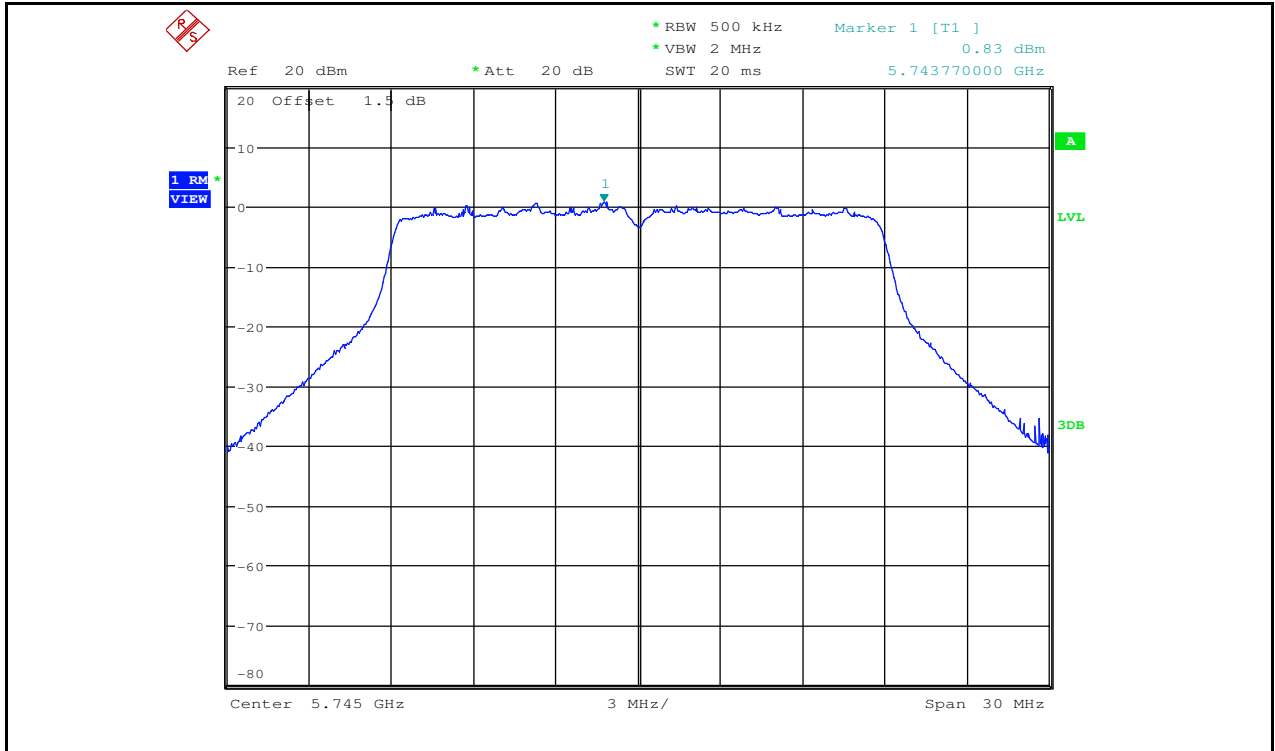
Maximum Power Spectral Density_TNVN_11AC20_5745_Ant2
