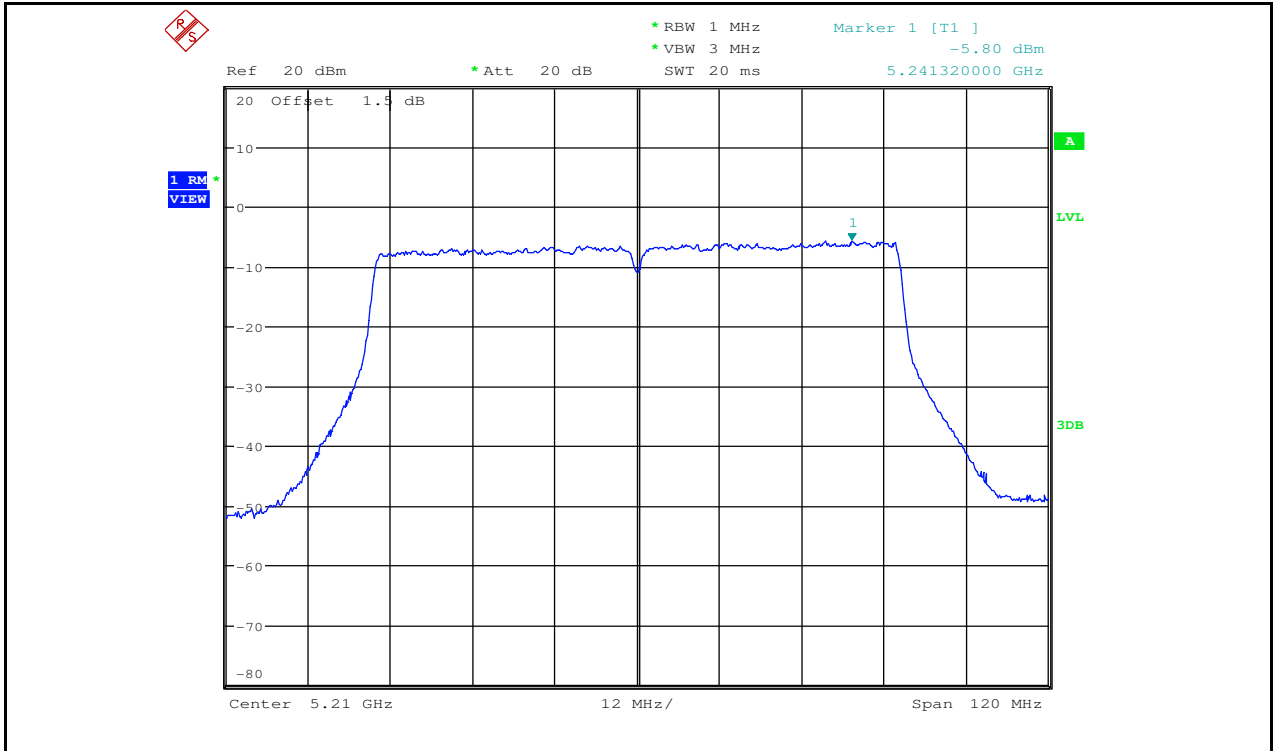
Maximum Power Spectral Density_TNVN_11AC80_5210_Ant2
