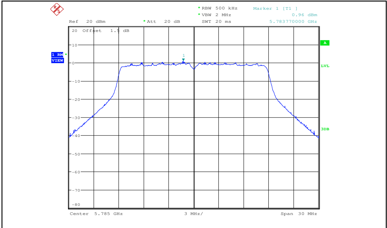
Maximum Power Spectral Density_TNVN_11AC20_5785_Ant2
