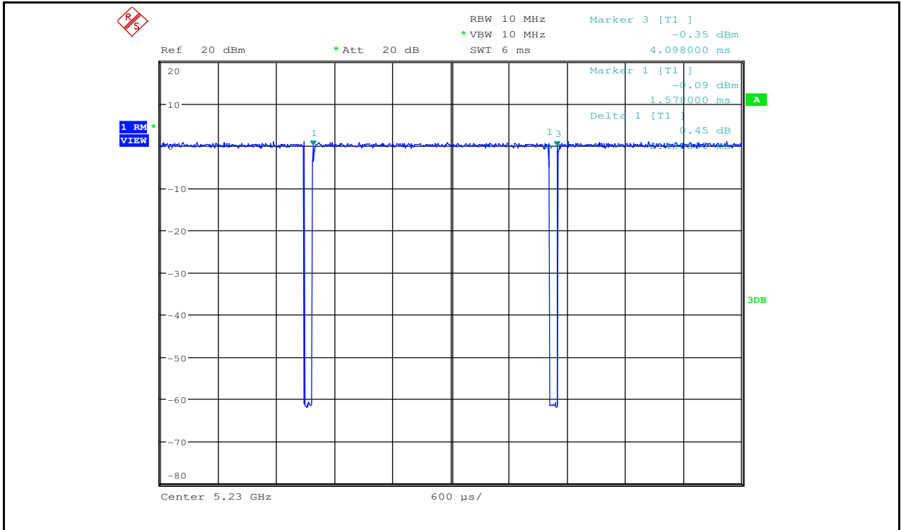
Duty Cycle_11N40_5230_Ant2
