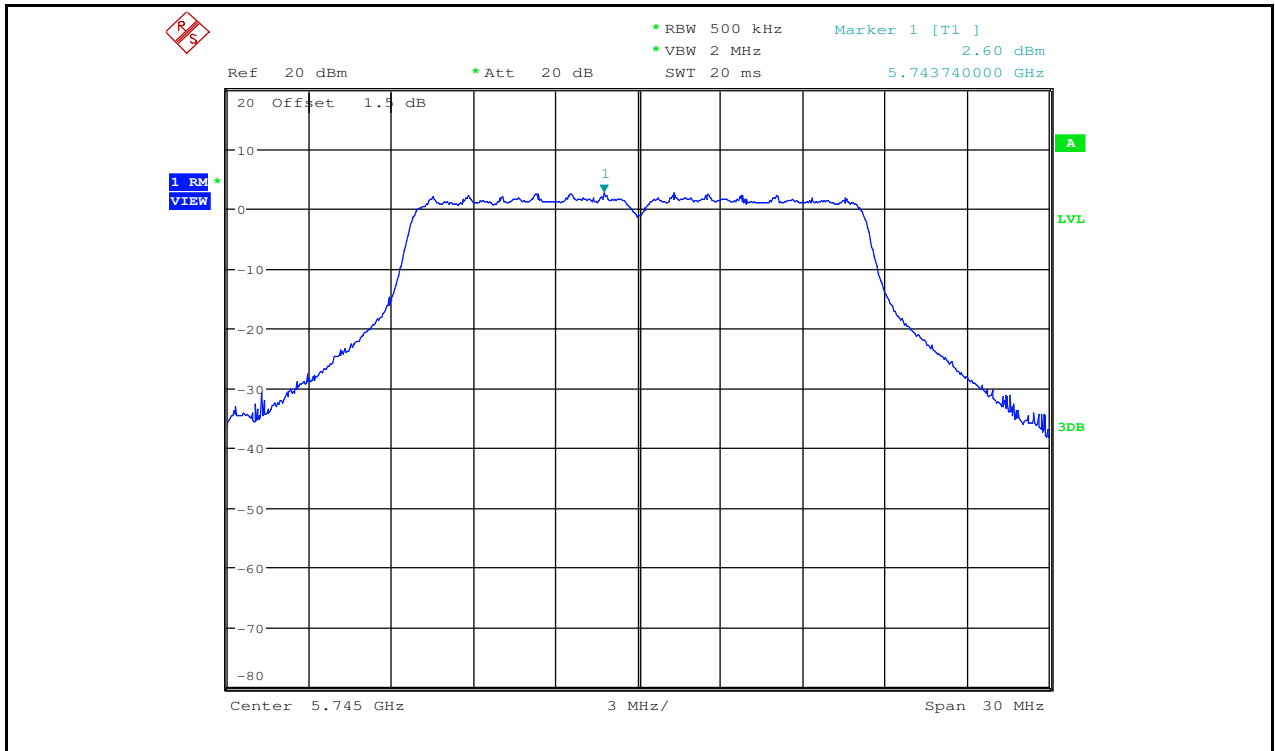
Maximum Power Spectral Density_TNVN_11A_5745_Ant2
