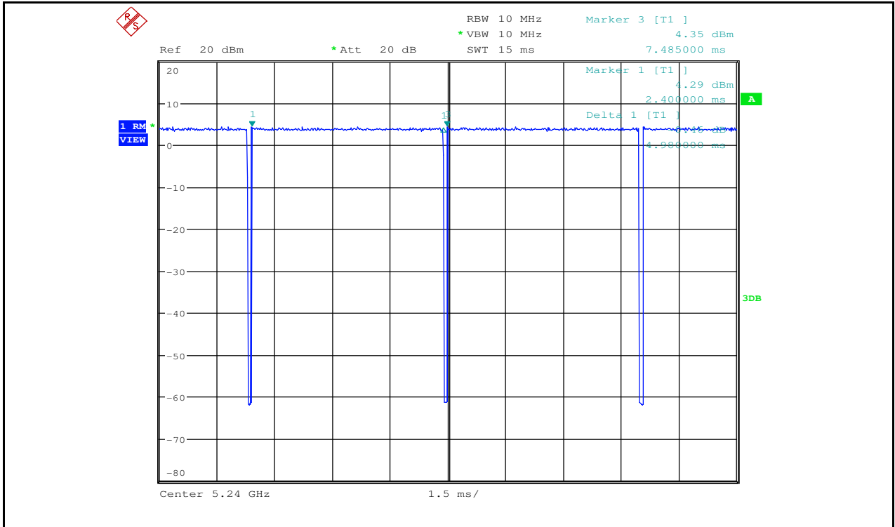
Duty Cycle_11AC20_5240_Ant2
