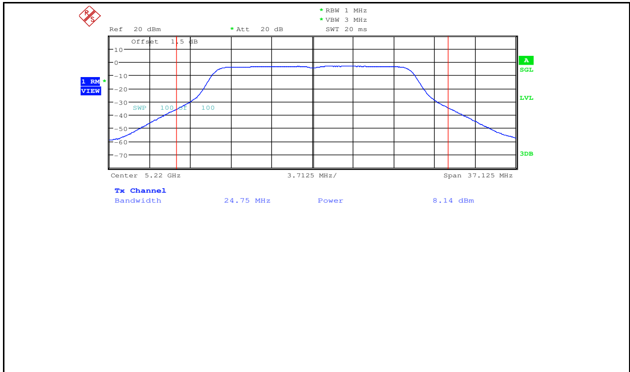
Maximum Conduct Output Power_11AC20_5220_Ant2
