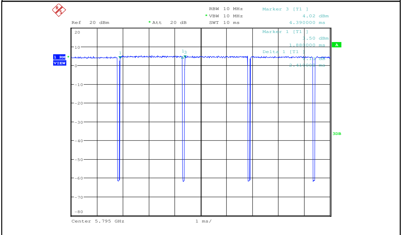
Duty Cycle_11AC40_5795_Ant2
