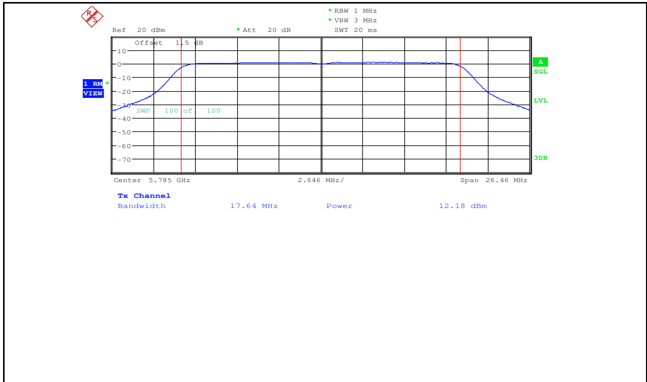
Maximum Conduct Output Power_11N20_5785_Ant2
