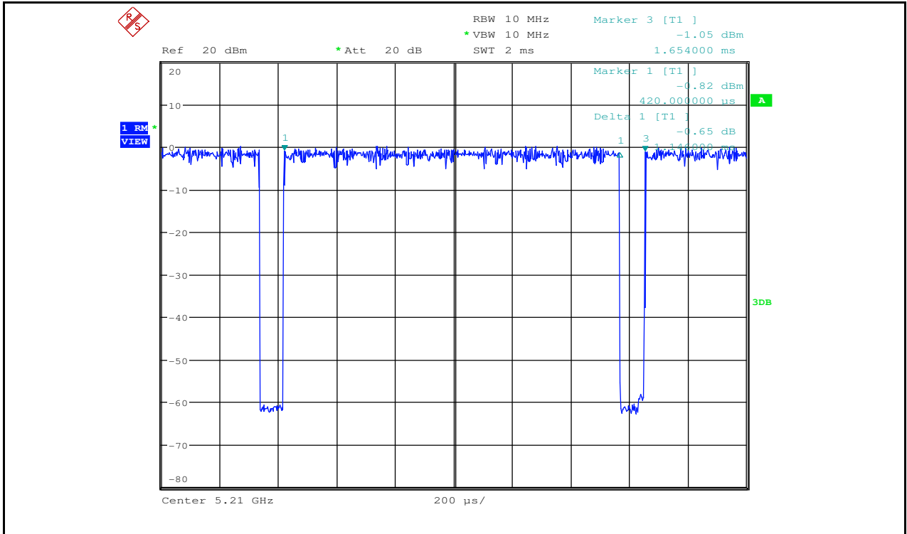
Duty Cycle_11AC80_5210_Ant2
