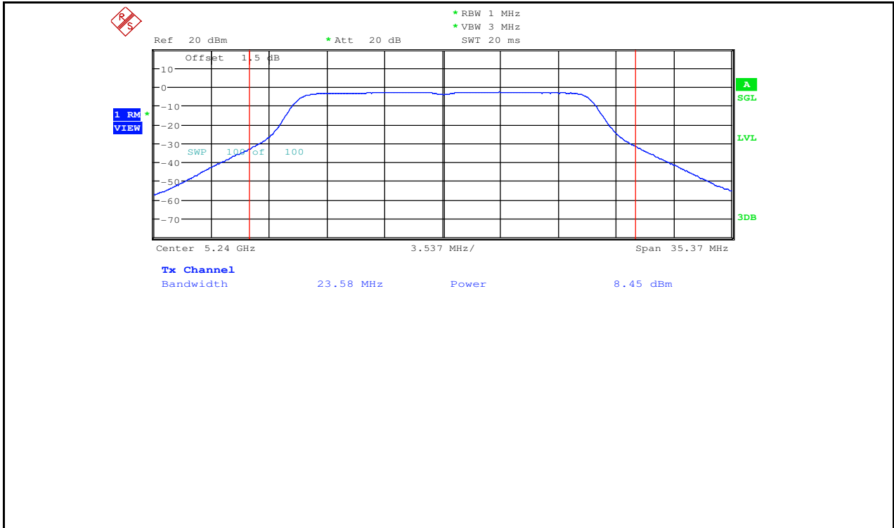
Maximum Conduct Output Power_11AC20_5240_Ant2
