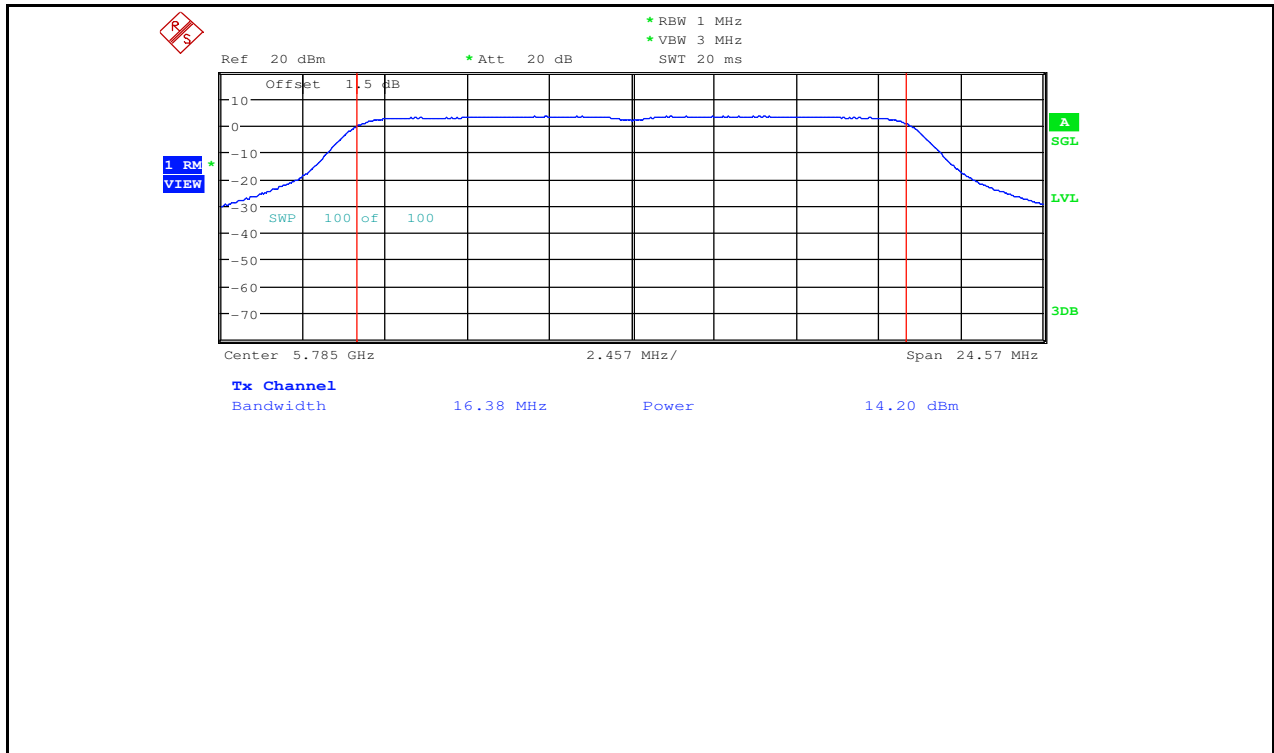
Maximum Conduct Output Power_11A_5785_Ant2
