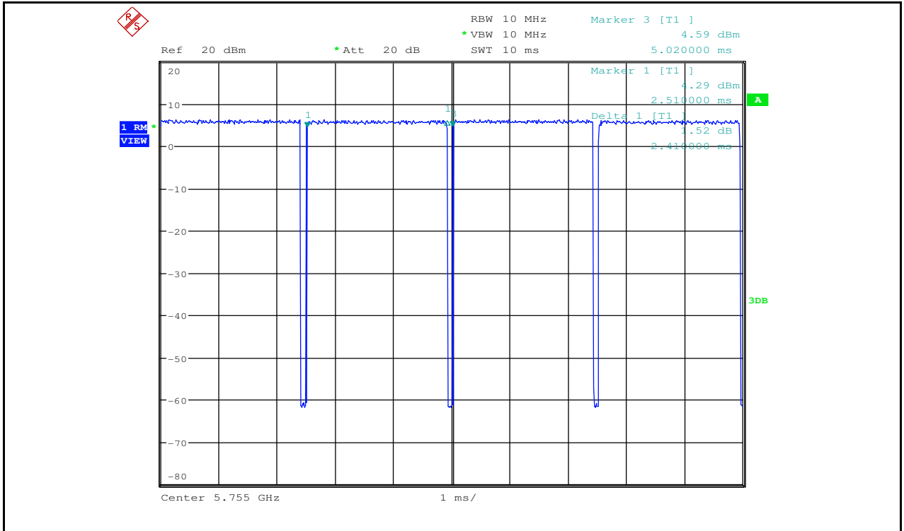
Duty Cycle_11AC40_5755_Ant2
