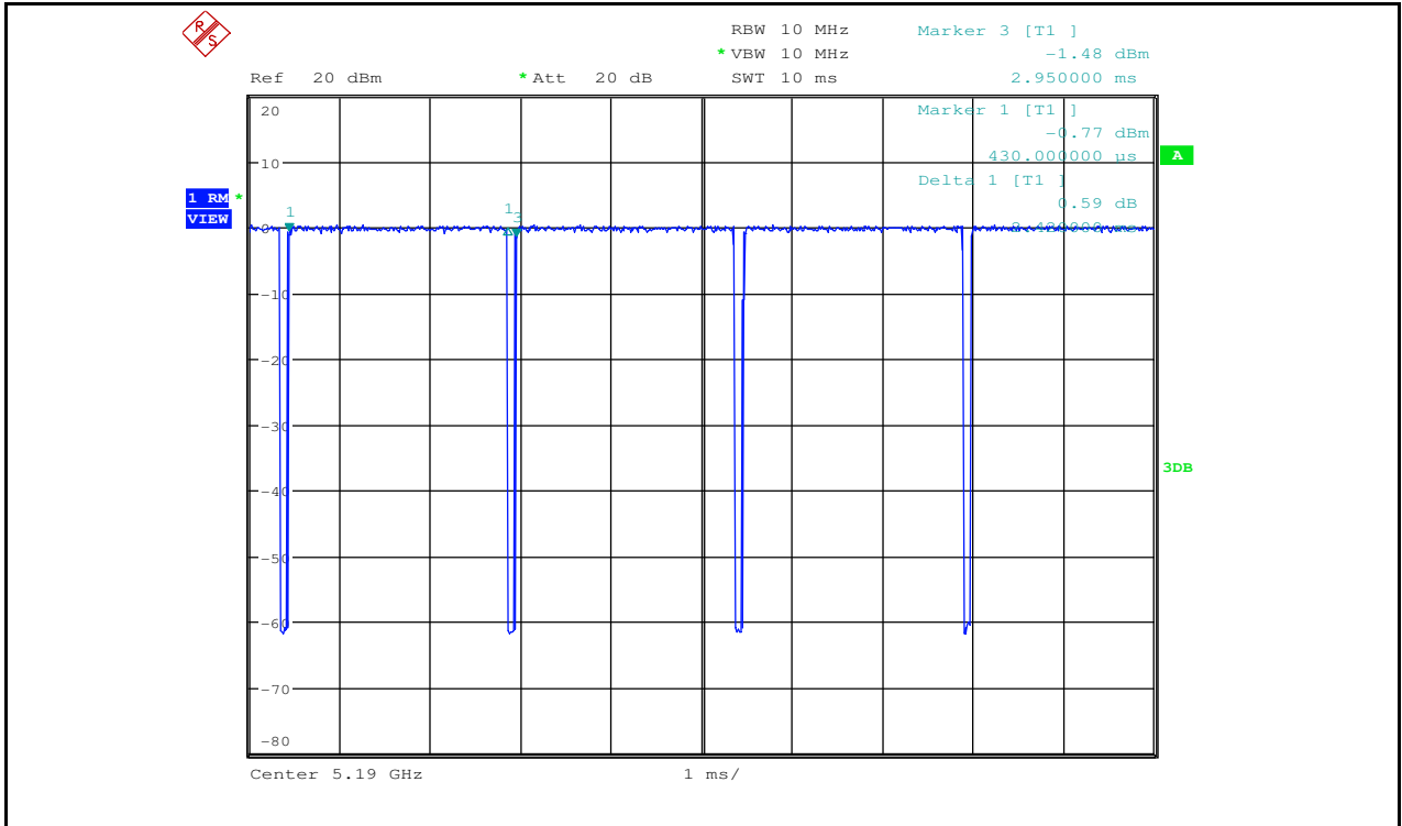
Duty Cycle_11AC40_5190_Ant2
