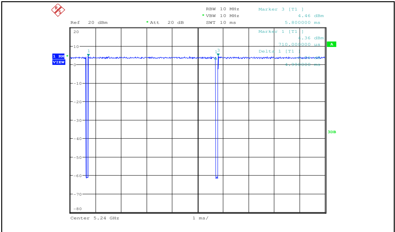
Duty Cycle_11N20_5240_Ant2
