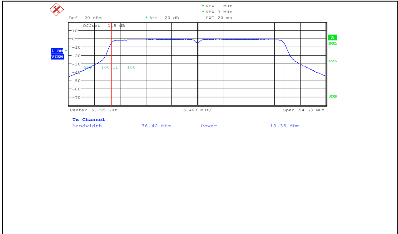
Maximum Conduct Output Power_11N40_5755_Ant2
