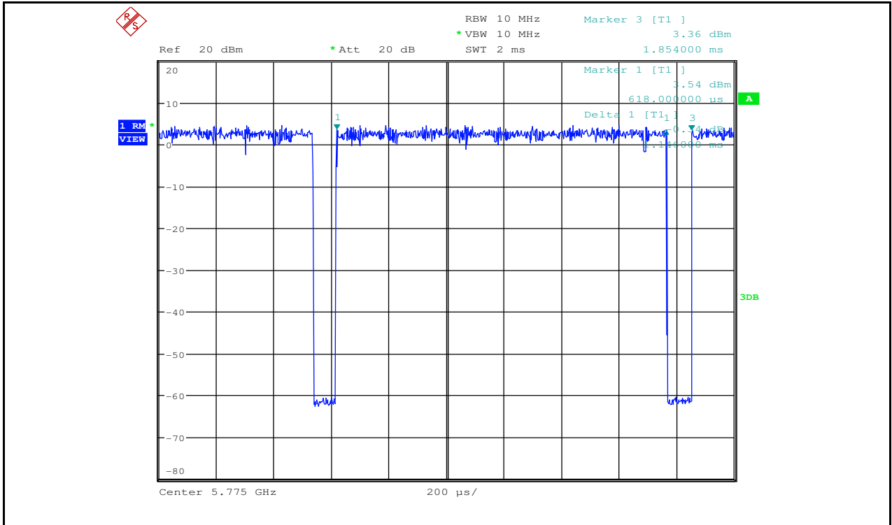
Duty Cycle_11AC80_5775_Ant2
