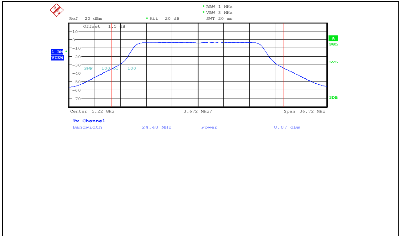
Maximum Conduct Output Power_11N20_5220_Ant2
