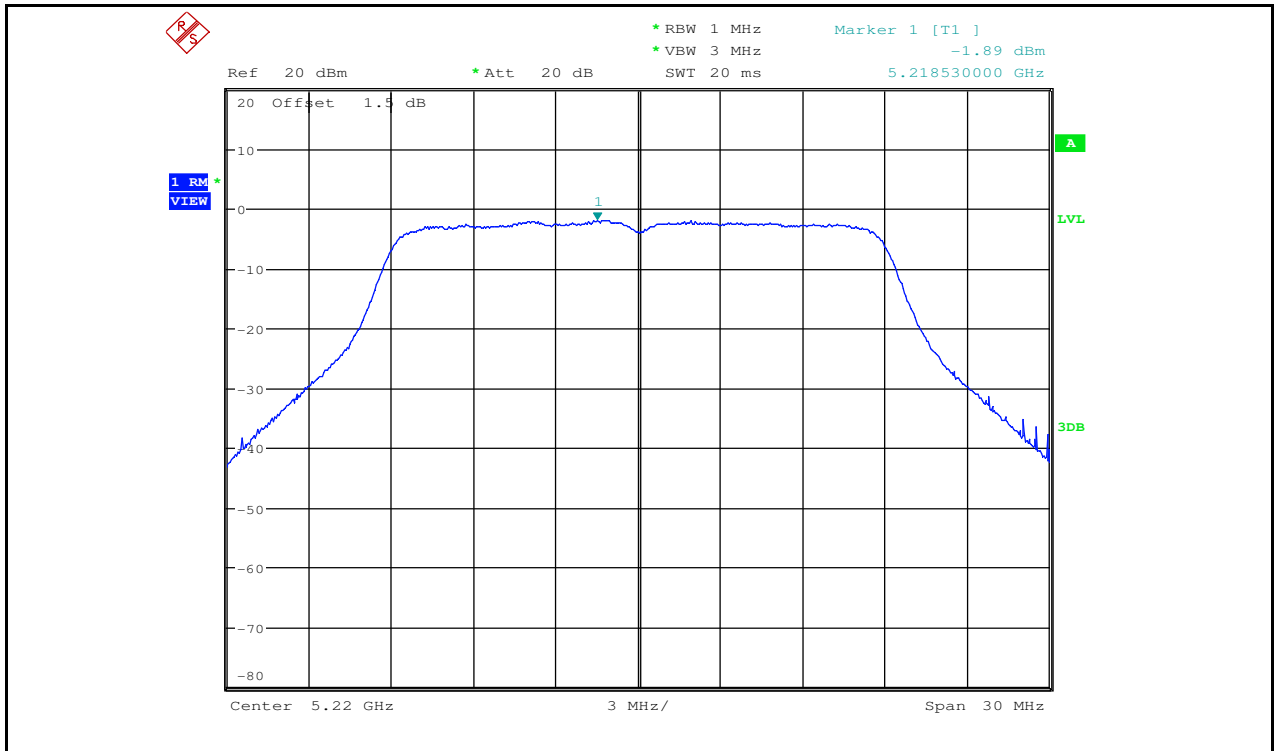
Maximum Power Spectral Density_TNVN_11AC20_5220_Ant2
