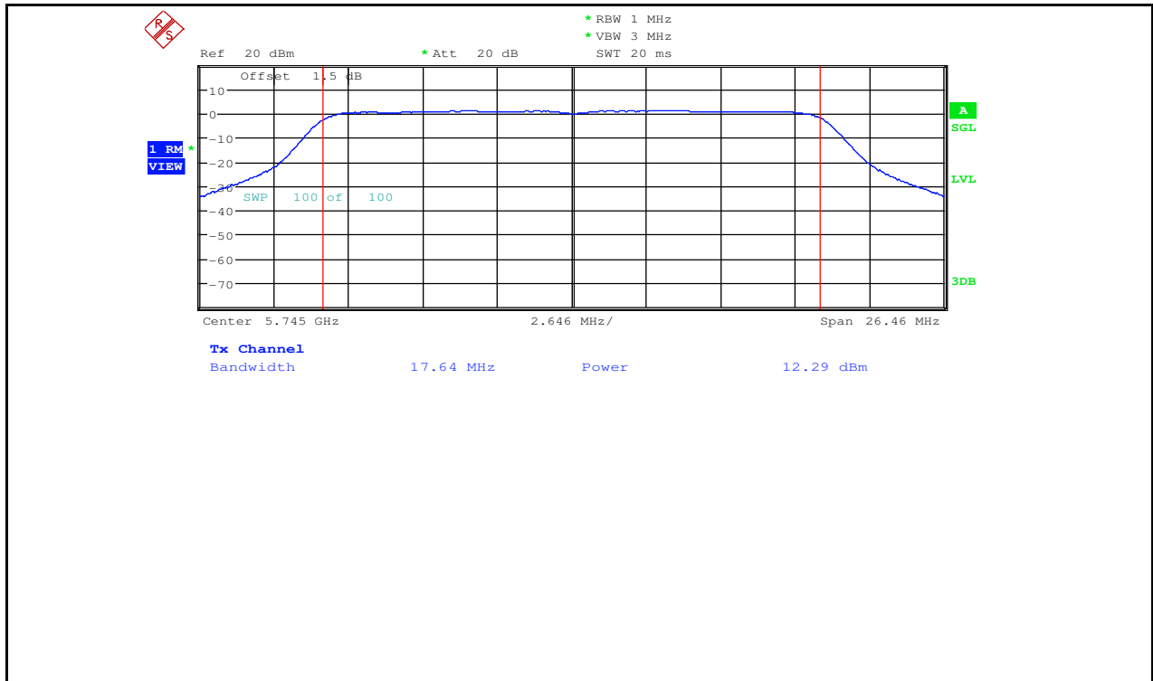
Maximum Conduct Output Power_11N20_5745_Ant2
