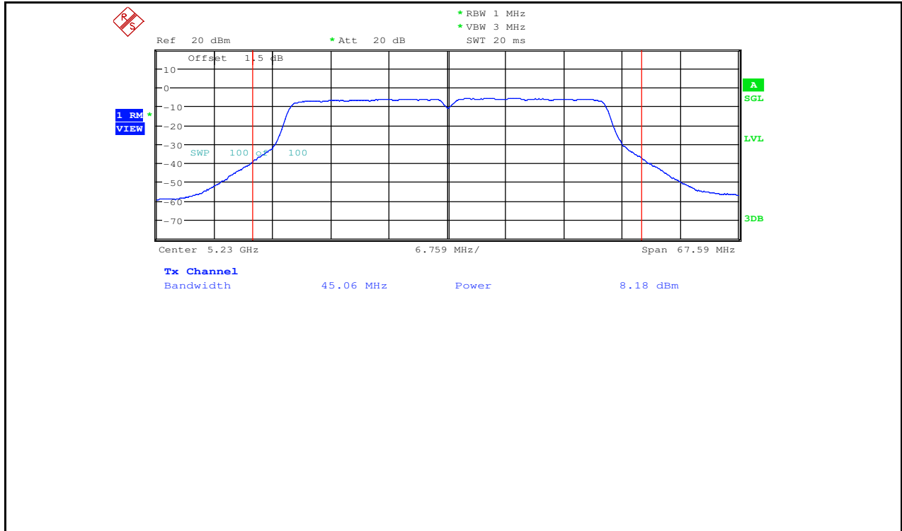
Maximum Conduct Output Power_11AC40_5230_Ant2
