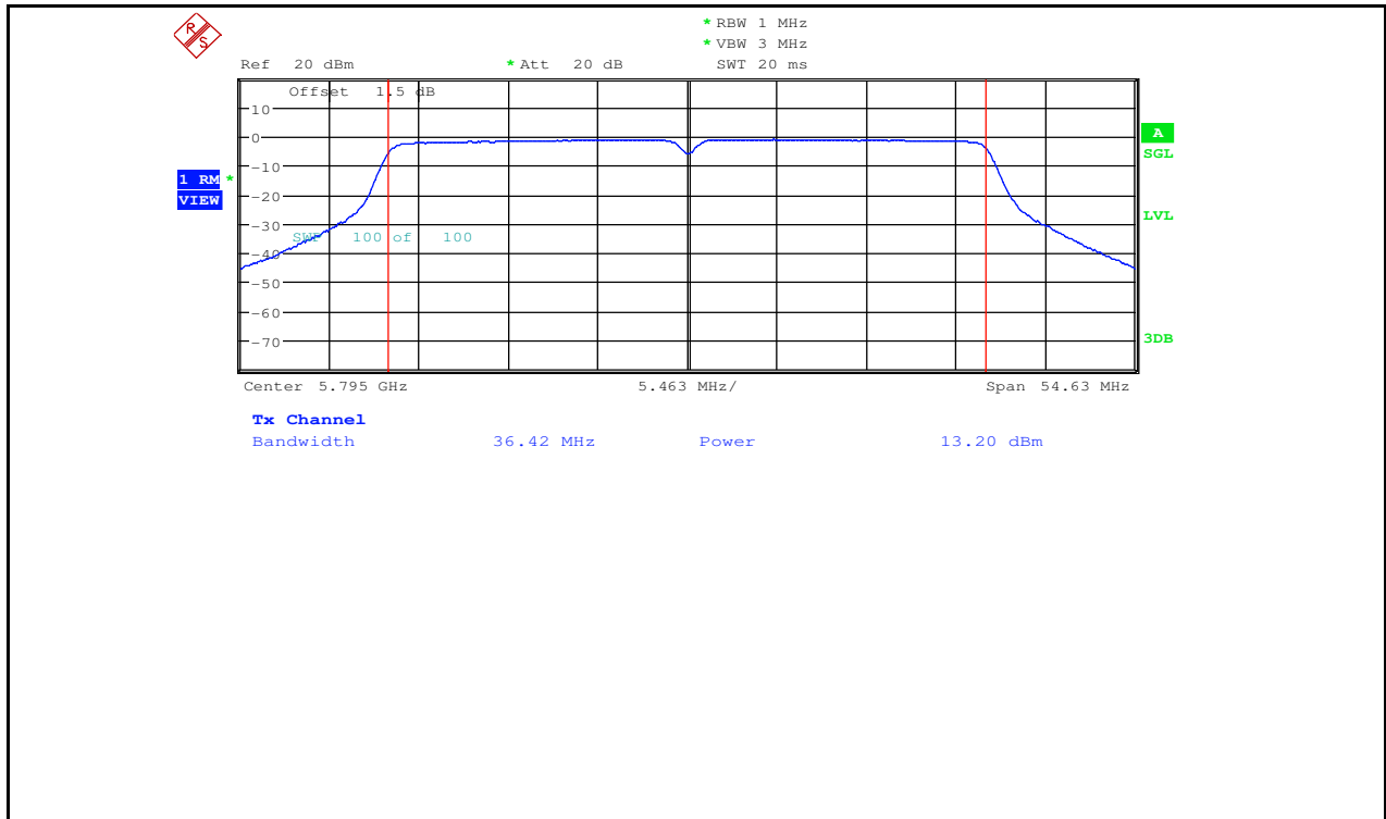
Maximum Conduct Output Power_11N40_5795_Ant2
