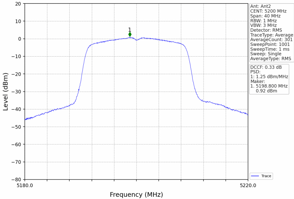
802.11ac(VHT20)_MCH_5200MHz_MIMO_NTNV
