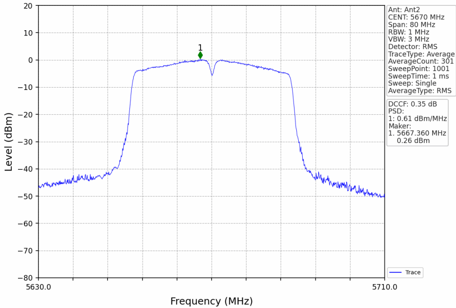
802.11n(HT40)_HCH_5670MHz_MIMO_NTNV
