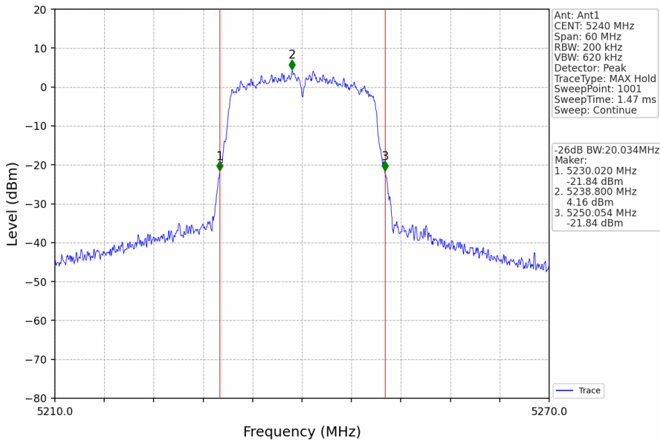
802.11ac(VHT20)_HCH_5240MHz_Ant1_NTNV
