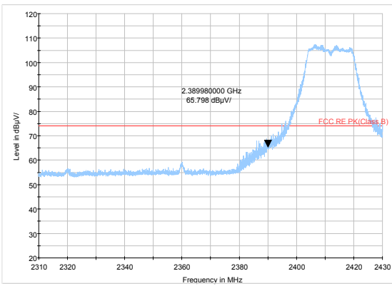
802.11g-Channel 1 Peak
