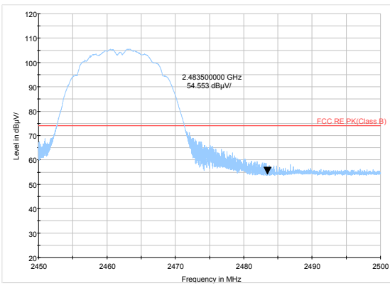
802.11b-Channel 11 Peak
