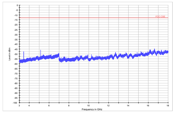
LTE Band 4 1.4MHz CH-Middle 3GHz~18GHz
