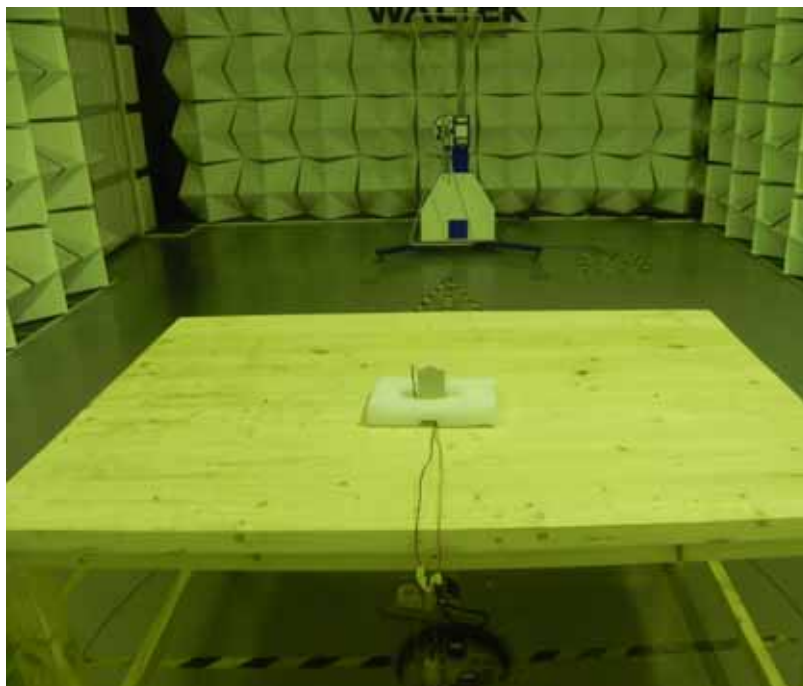
Photograph – Radiated Emission Test Setup for 30MHz ~ 1000MHz at Test Site 2#
