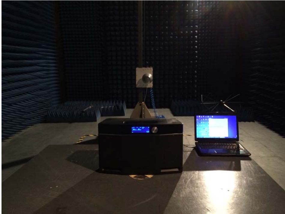
Above 1GHz
