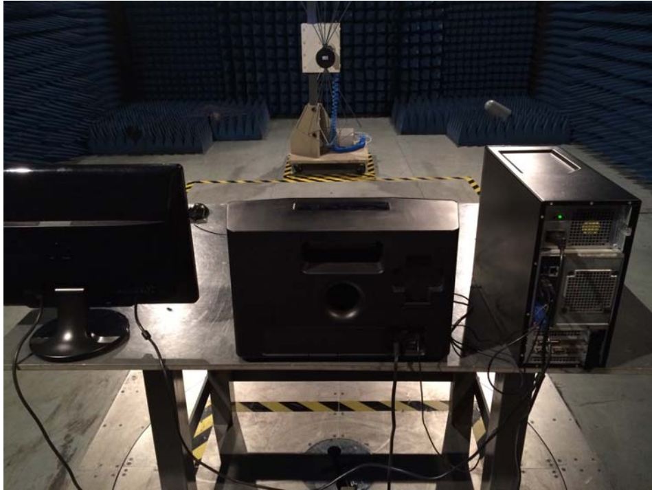
Setup Back and the cables shown
