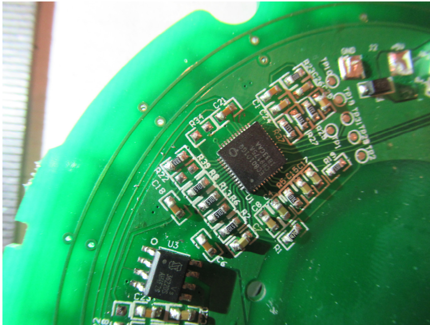
EUT – PCB Bottom IC Chip View
