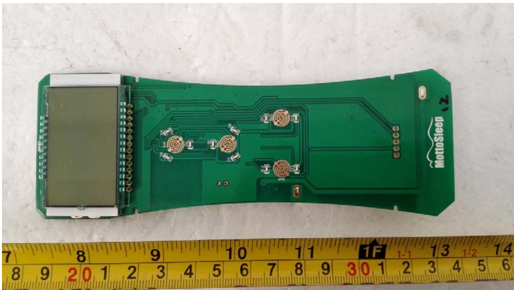
EUT –Mainboard Rear View
