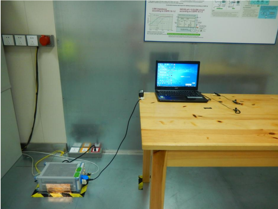
DSS conduction
