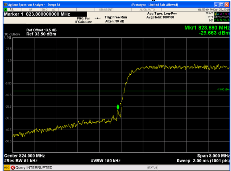
WCDMA band V band edge-left side
