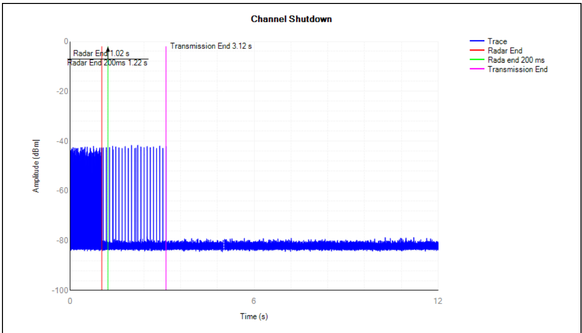
802.11ac80 channel 58 5290MHz
