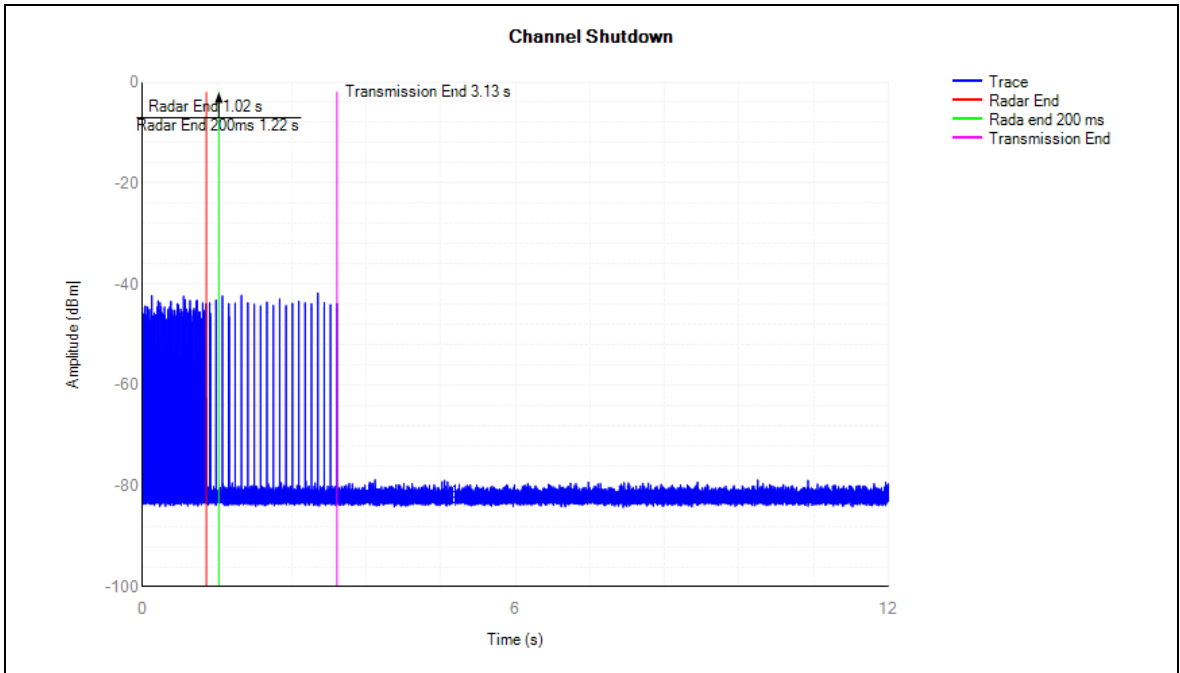
802.11n40 channel 54 5270MHz
