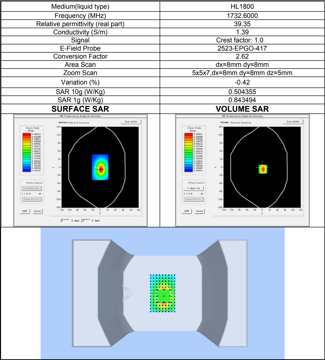
Plot 8: WCDMA BAND IV, Middle channel (Body-worn/Hotspot, Top Edge) Product Description: Smart Phone Test Date: 2024-08-05
