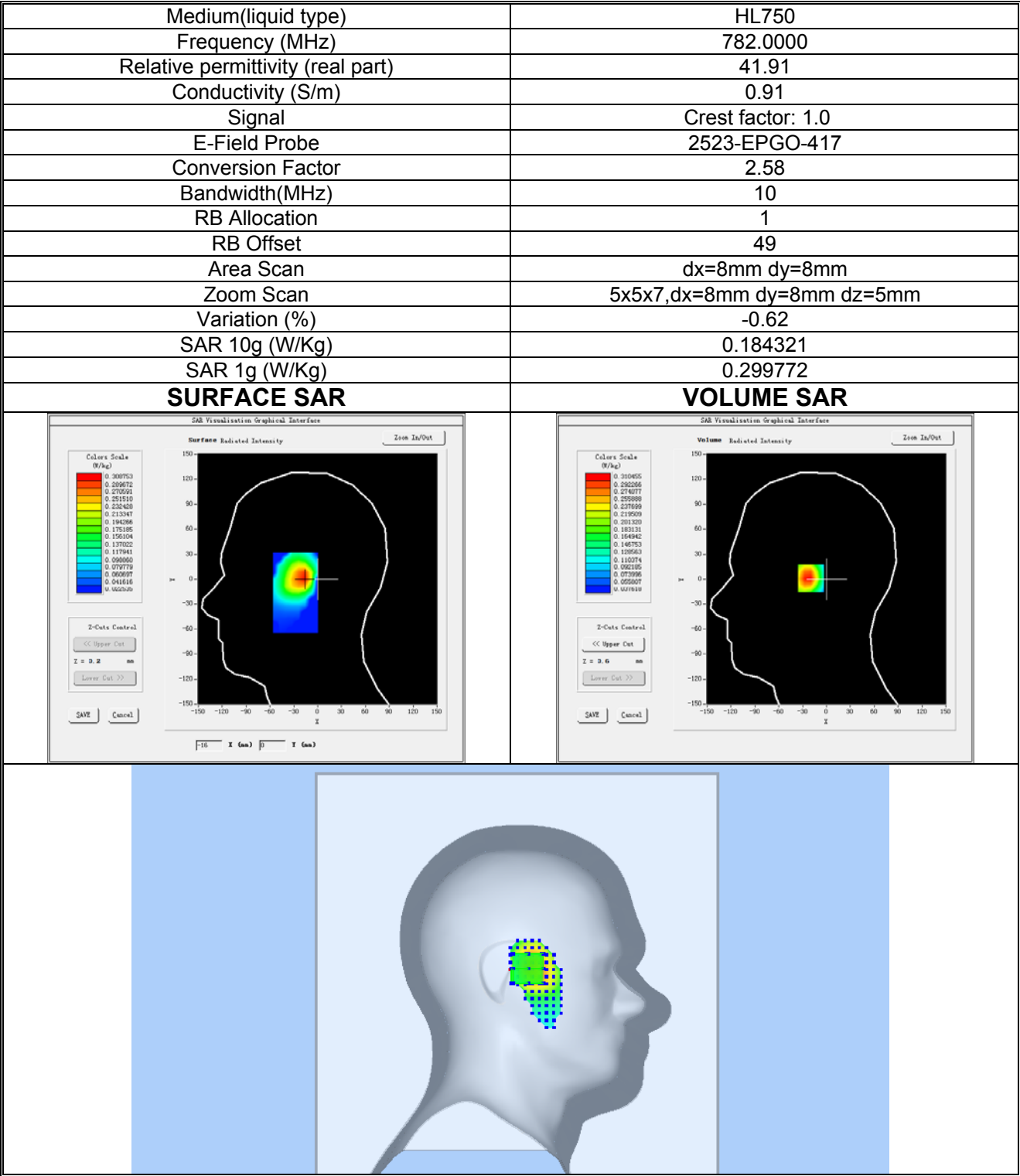
Plot 19:LTE BAND 13, Low channel (Left Head Cheek) Product Description: Smart Phone Test Date: 2024-07-30
