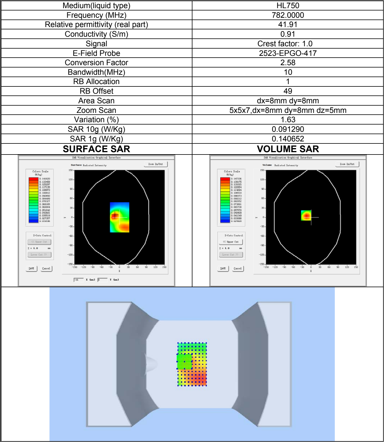
Plot 20: LTE BAND 13, Low channel (Body-worn/ Hotspot, Back Side) Product Description: Smart Phone Test Date: 2024-07-30
