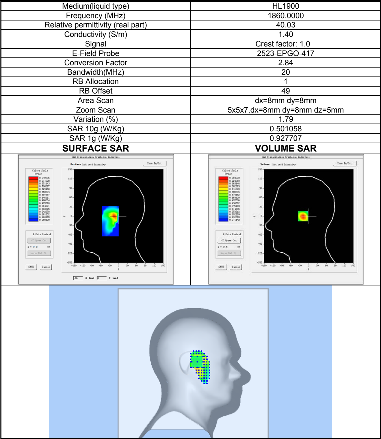
Plot 11:LTE BAND 2, Low channel (Left Head Cheek) Product Description:Smart Phone Test Date: 2024-08-02
