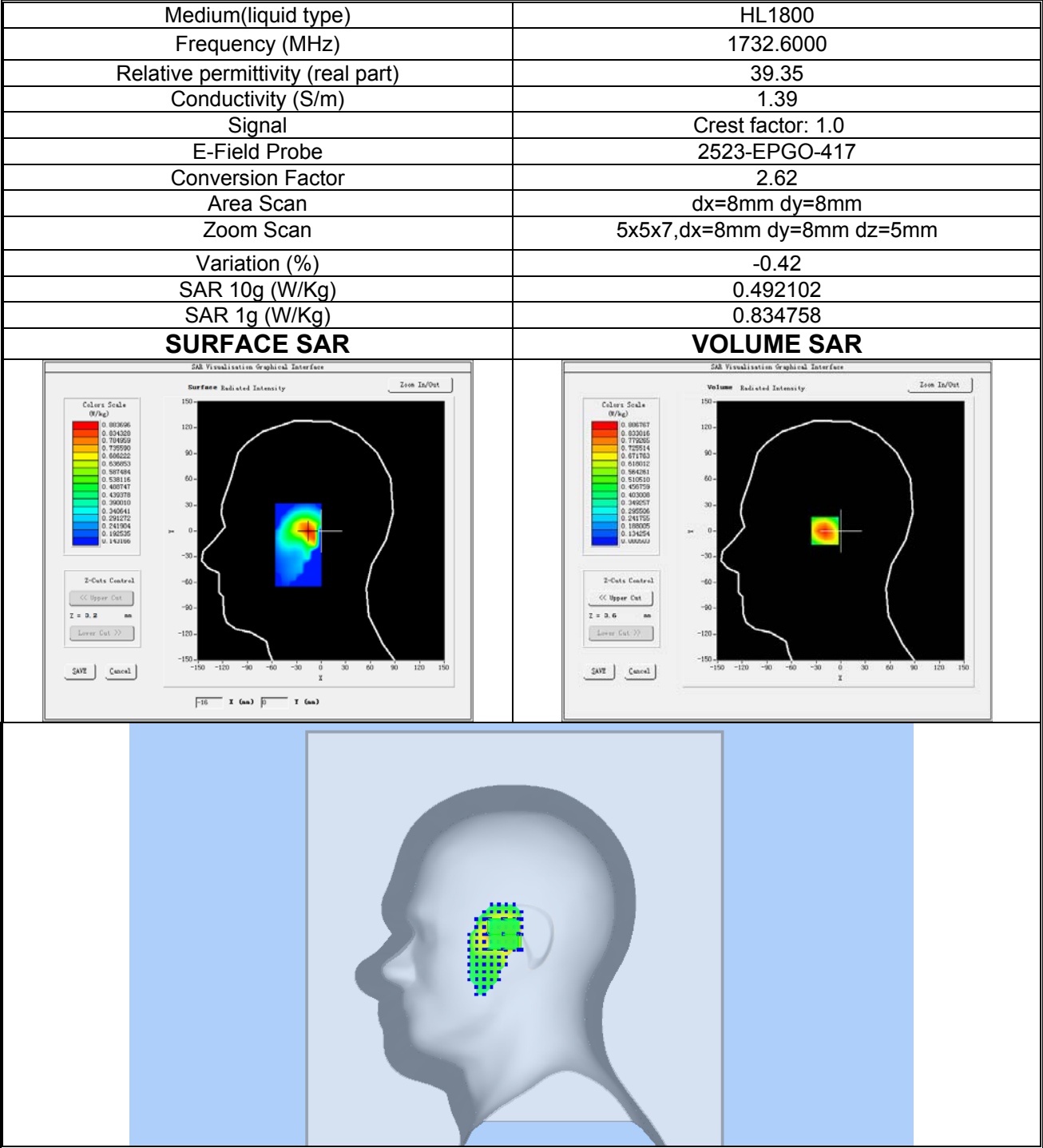
Plot 7: WCDMA BAND IV, Middle channel (Right Head Cheek) Product Description: Smart Phone Test Date: 2024-08-05
