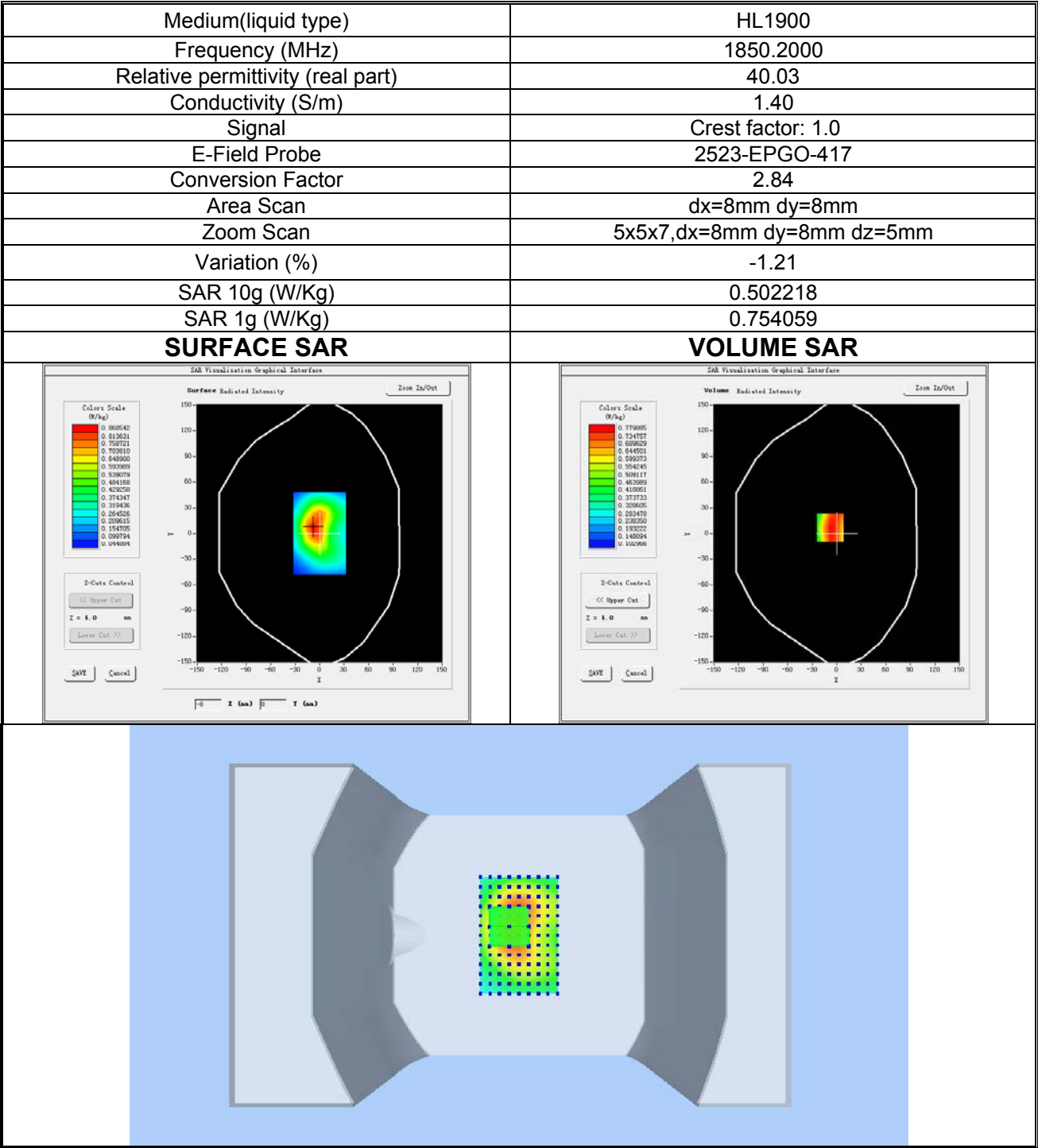
Plot 4: GPRS1900, Low channel (Body-worn /Hotspot, Back Side) Product Description: Smart Phone Test Date: 2024-08-02
