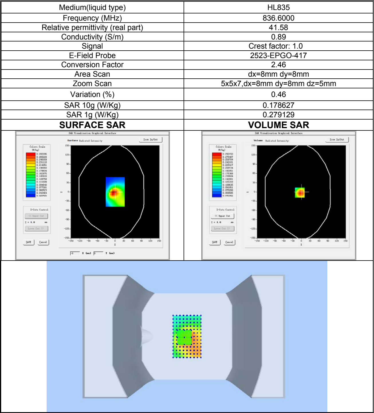
Plot 10: WCDMA BAND V, Middle channel (Body-worn/Hotspot, Back Side) Product Description: Smart Phone Test Date: 2024-07-30
