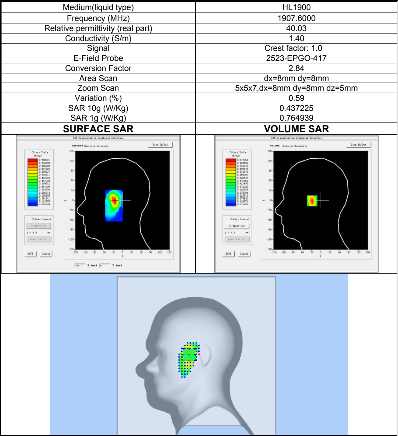
Plot 5: WCDMA BAND II, High channel (Right Head Cheek) Product Description: Smart Phone Test Date: 2024-08-02
