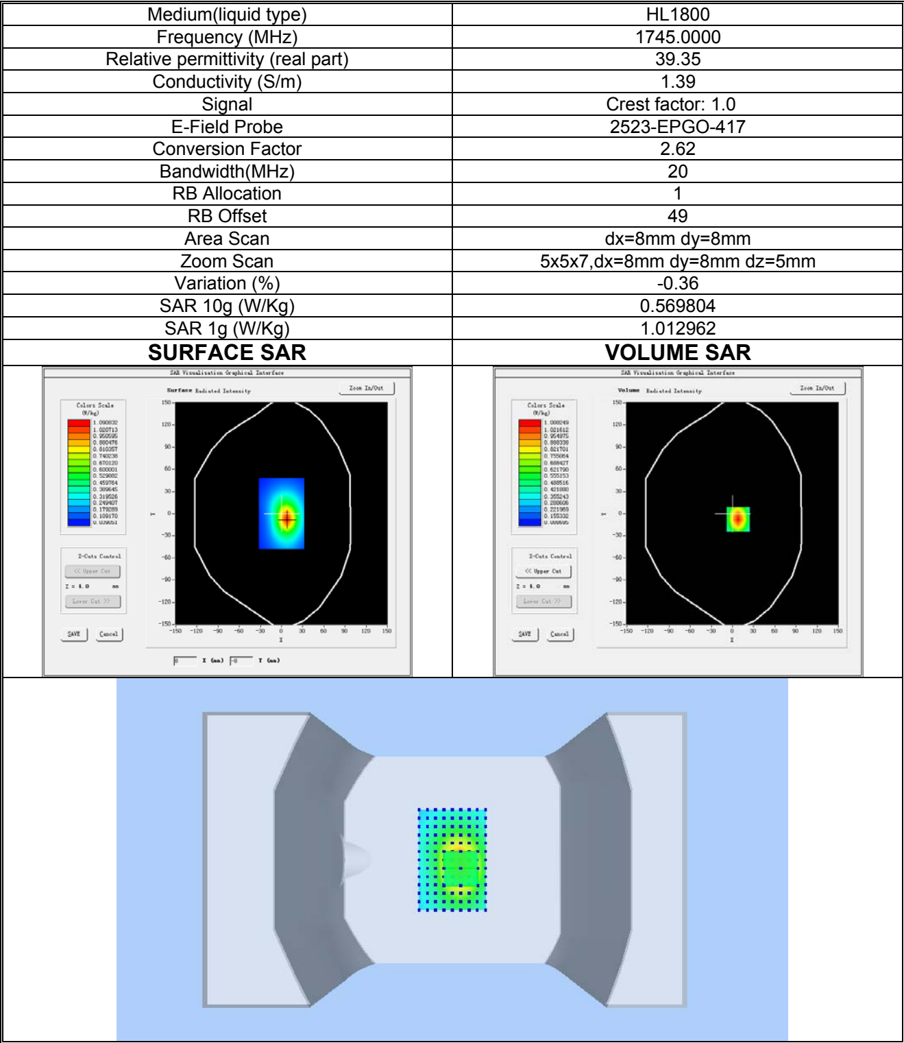
Plot 14: LTE BAND 4, High channel (Body-worn/ Hotspot, Top Edge) Product Description: Smart Phone Test Date: 2024-08-05
