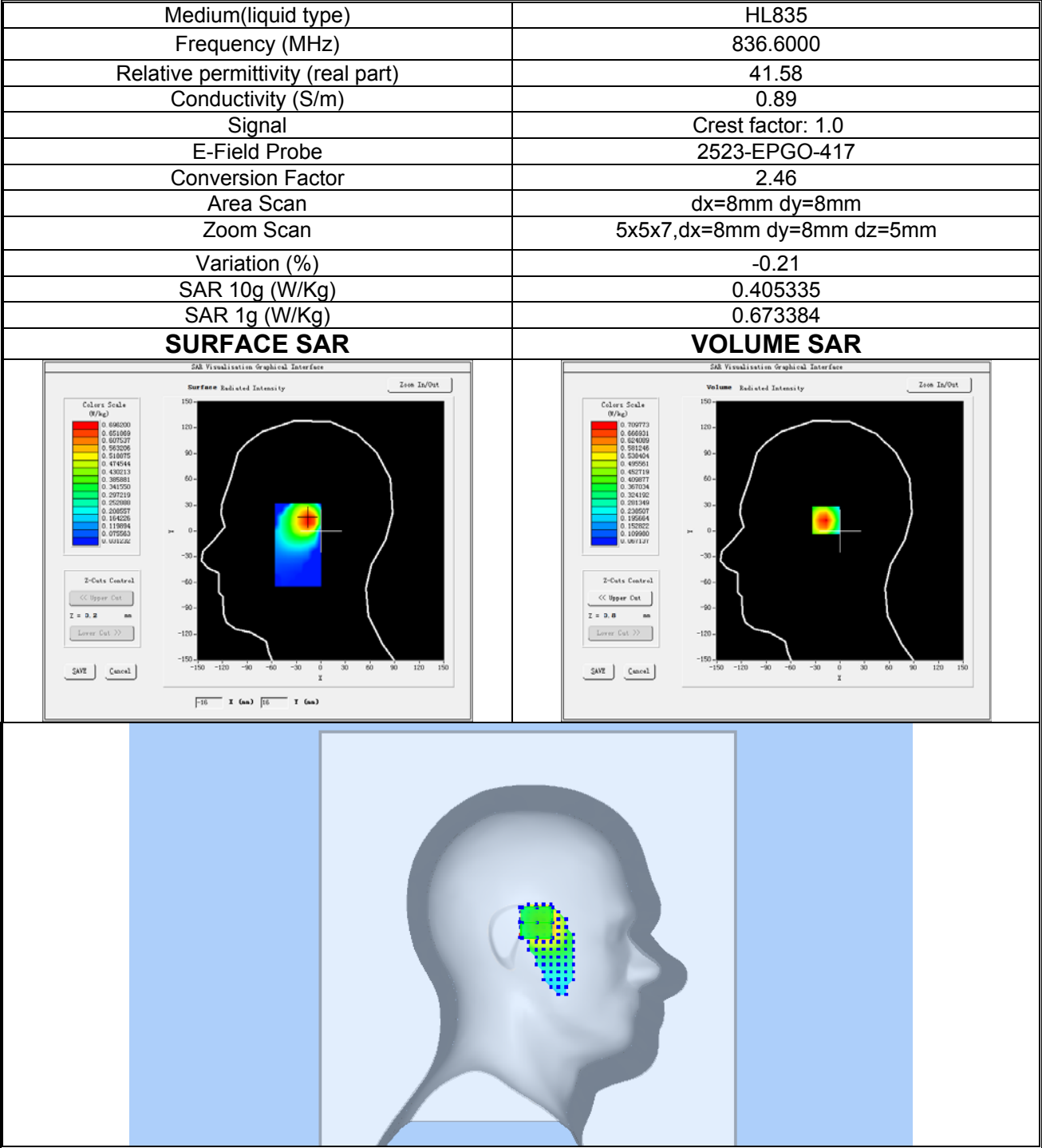
Plot 9: WCDMA BAND V, Middle channel (Left Head Cheek) Product Description: Smart Phone Test Date: 2024-07-30
