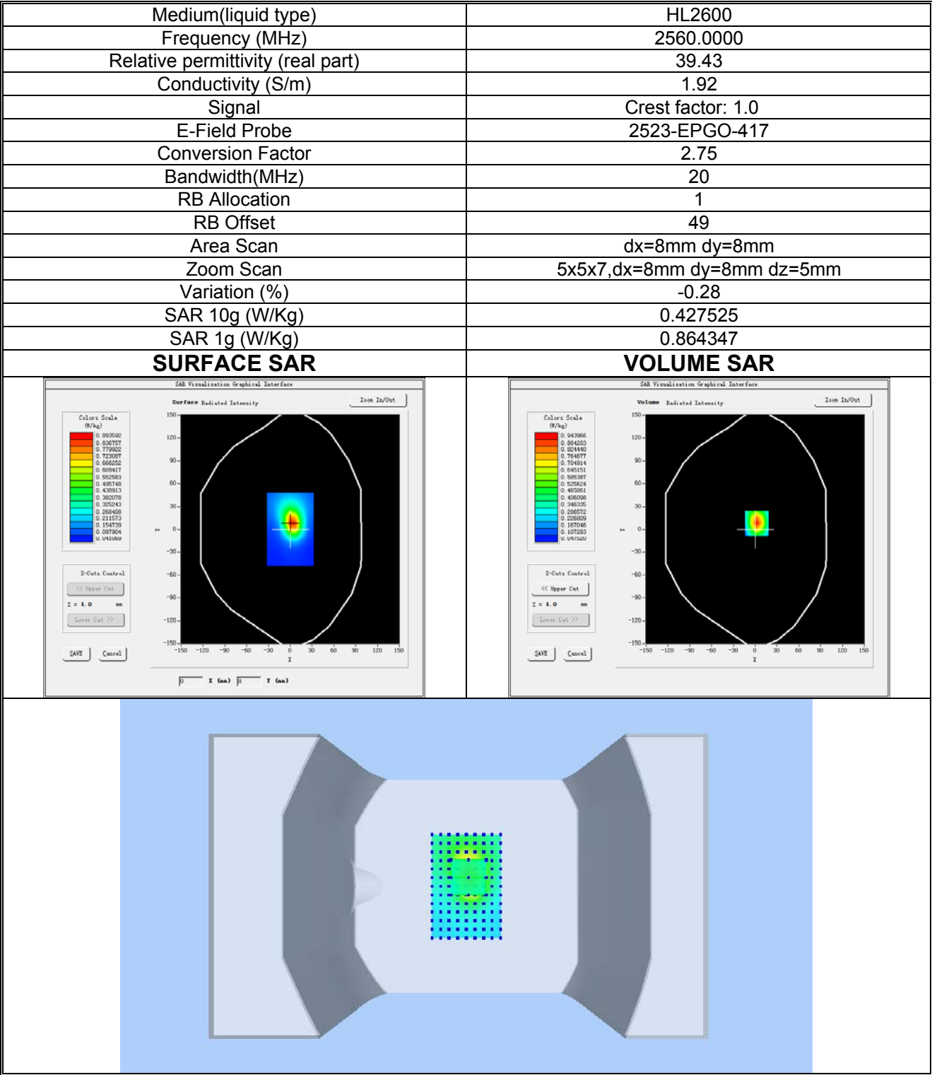
Plot 18: LTE BAND 7, High channel (Body-worn/ Hotspot, Top Edge) Product Description: Smart Phone Test Date: 2024-07-29
