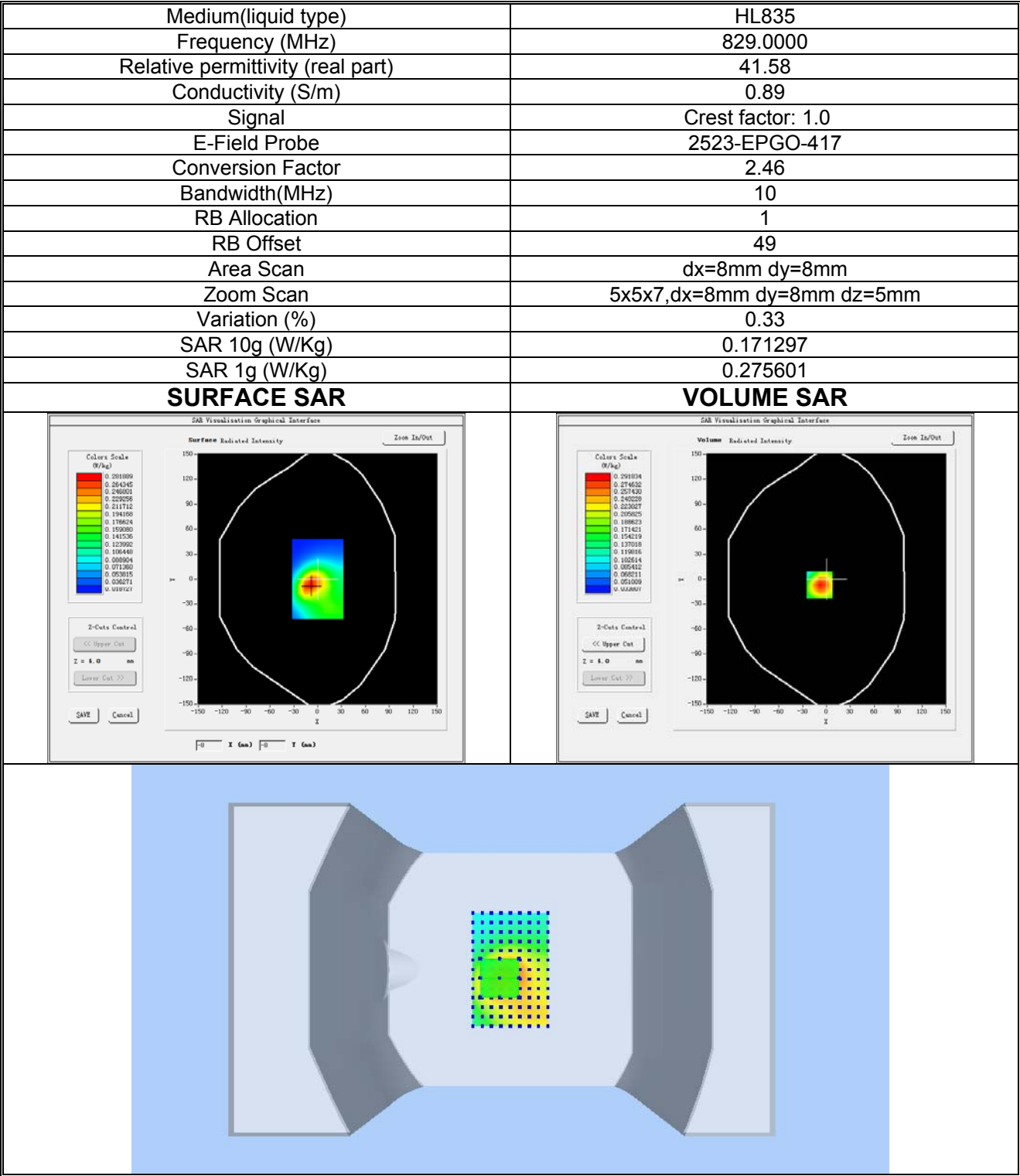
Plot 16: LTE BAND 5, Low channel (Body-worn/ Hotspot, Back Side) Product Description: Smart Phone Test Date: 2024-07-30
