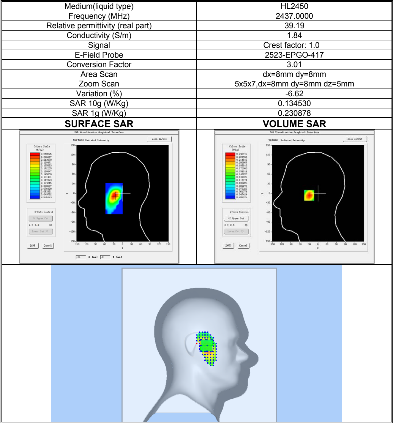
Plot 21:2.4G Wi-Fi, Middle channel (Left Head Cheek) Product Description: Smart Phone Test Date: 2024-07-29
