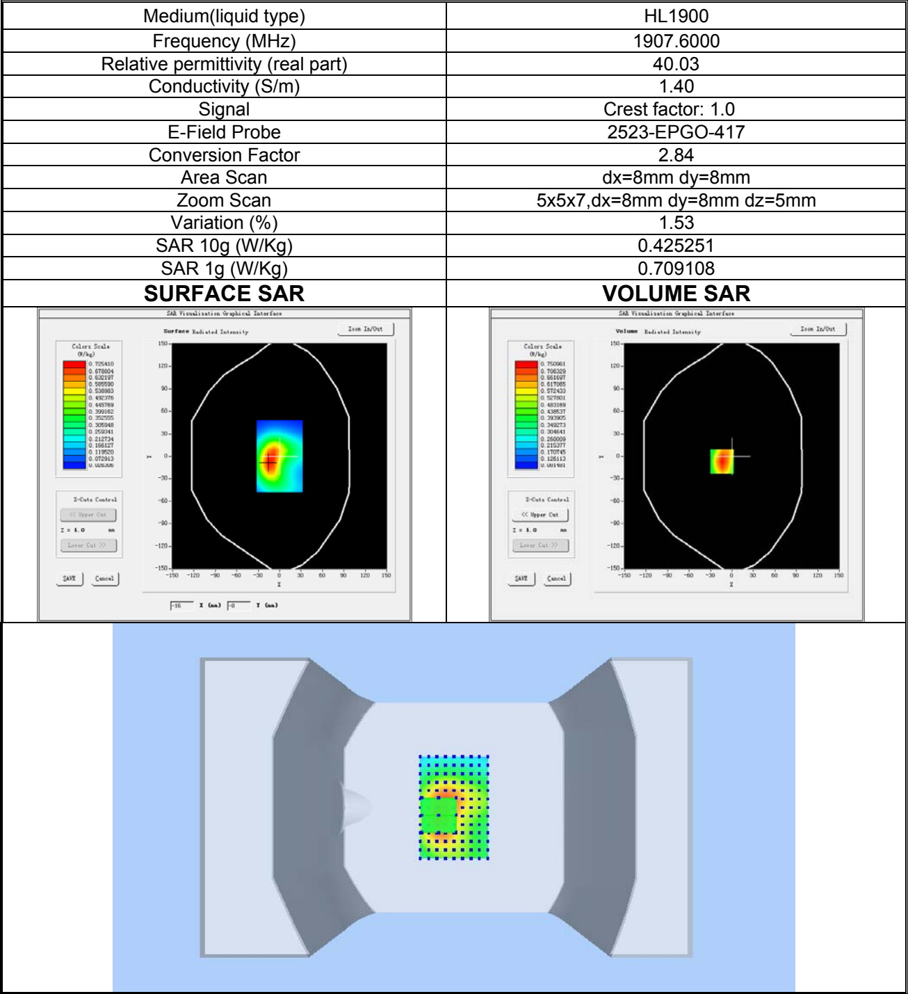
Plot 6: WCDMA BAND II, High channel (Body-worn /Hotspot, Back Side) Product Description: Smart Phone Test Date: 2024-08-02
