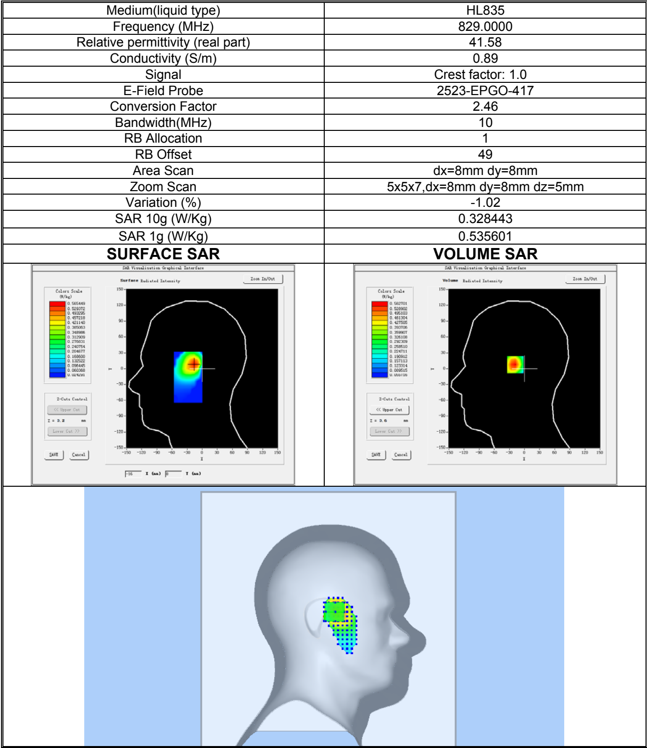
Plot 15:LTE BAND 5, Low channel (Left Head Cheek) Product Description: Smart Phone Test Date: 2024-07-30
