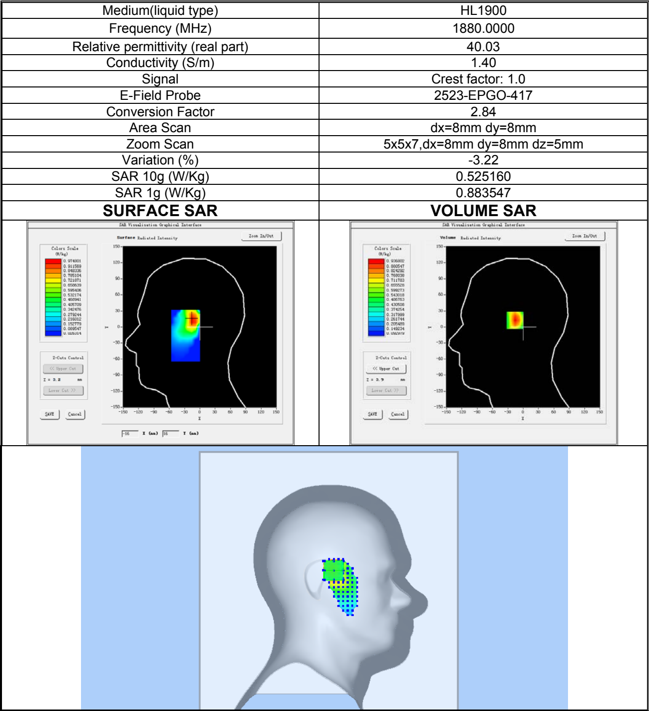
Plot 3: GPRS1900, Middle channel (Left Head Cheek) Product Description: Smart Phone Test Date: 2024-08-02
