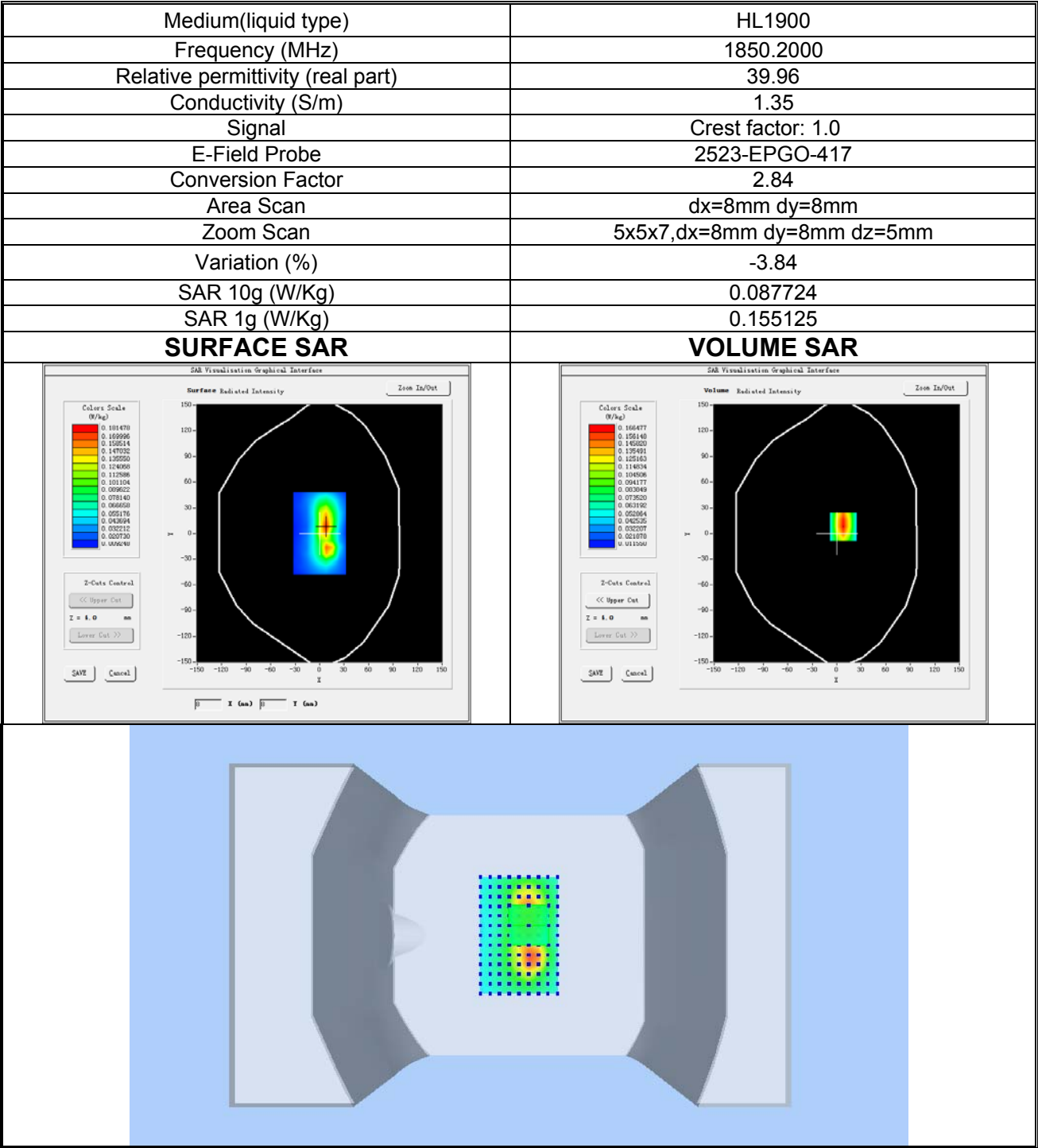
Plot 4: GPRS1900, Low channel (Body-worn /Hotspot, Bottom Edge) Product Description: Smart Phone Test Date: 2024-10-12
