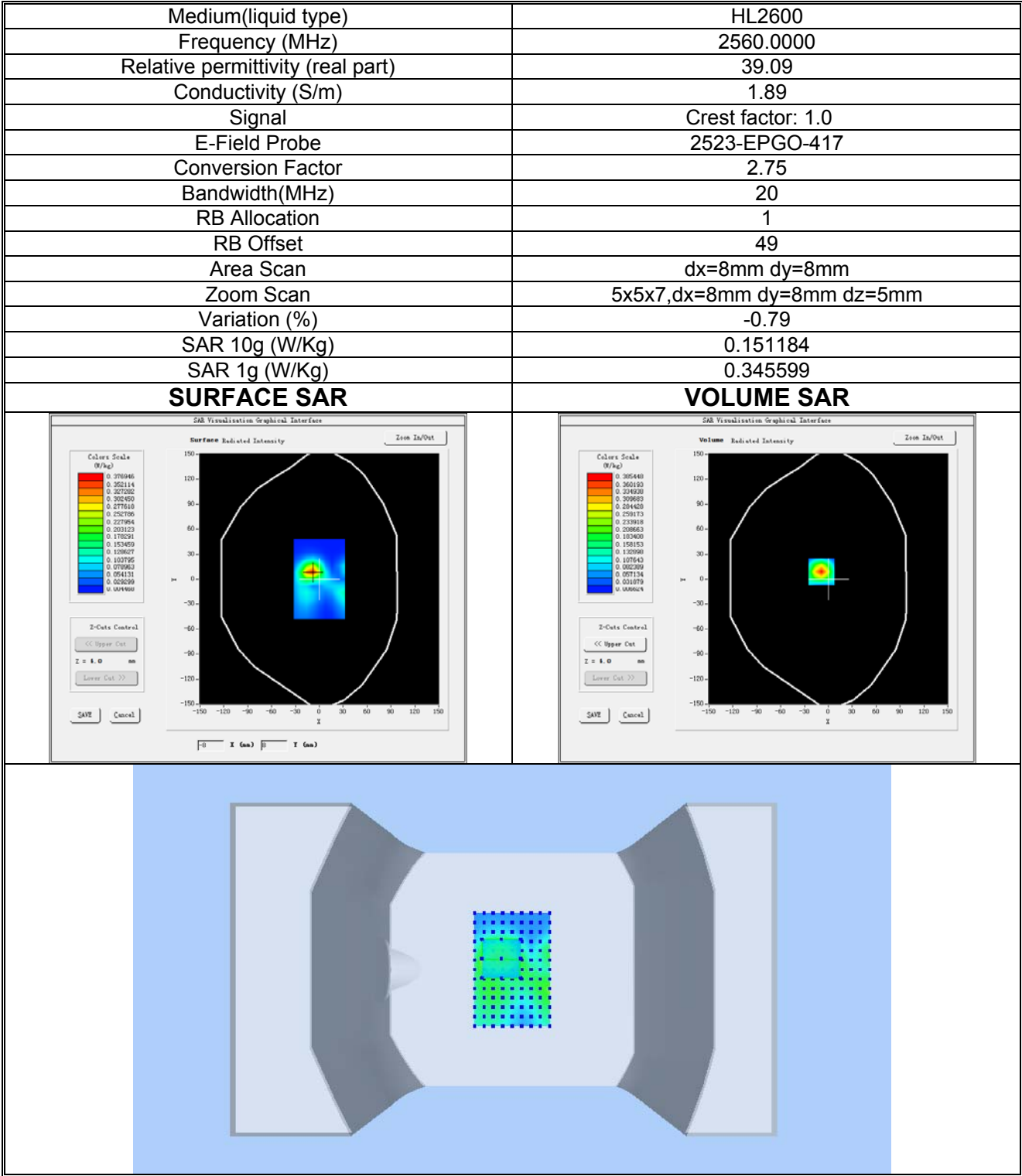
Plot 18: LTE BAND 7, High channel (Body-worn/ Hotspot, Back Side) Product Description: Smart Phone Test Date: 2024-10-18
