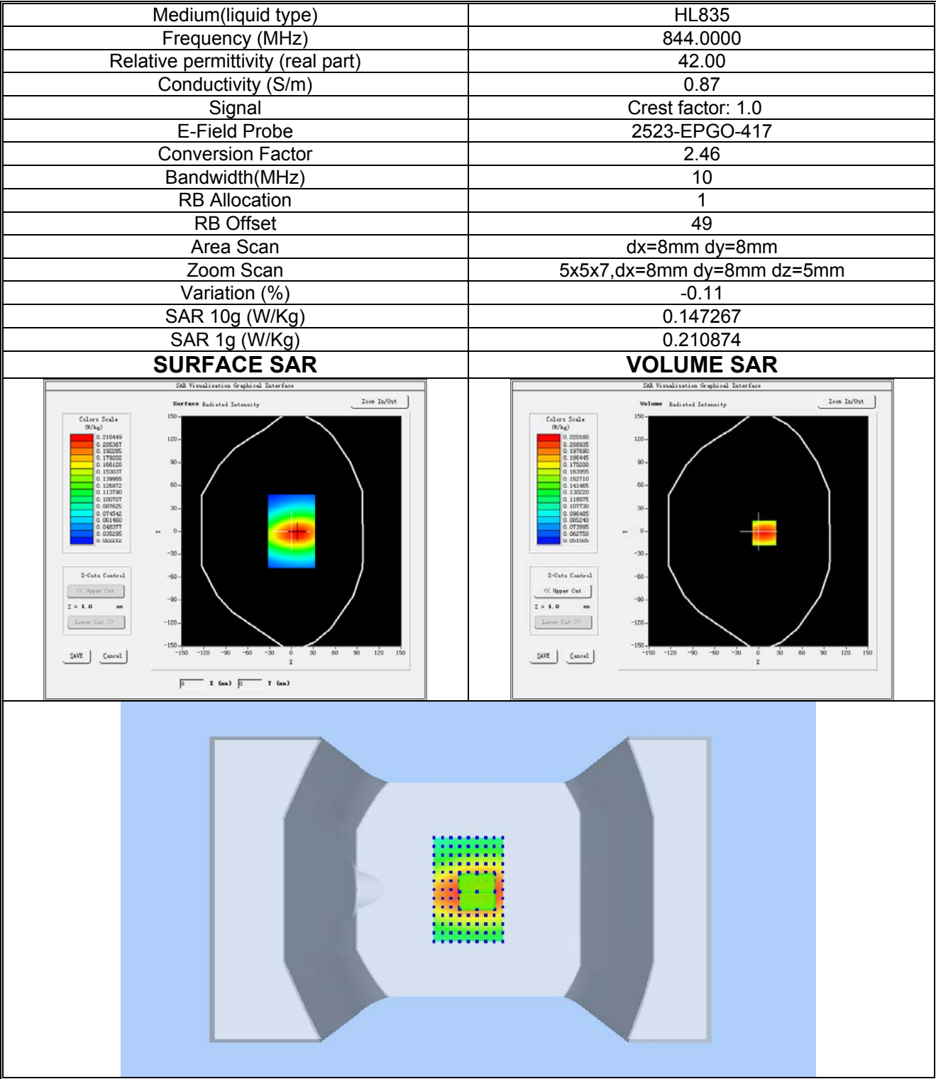
Plot 16: LTE BAND 5, High channel (Body-worn/ Hotspot, Right Edge) Product Description: Smart Phone Test Date: 2024-10-14
