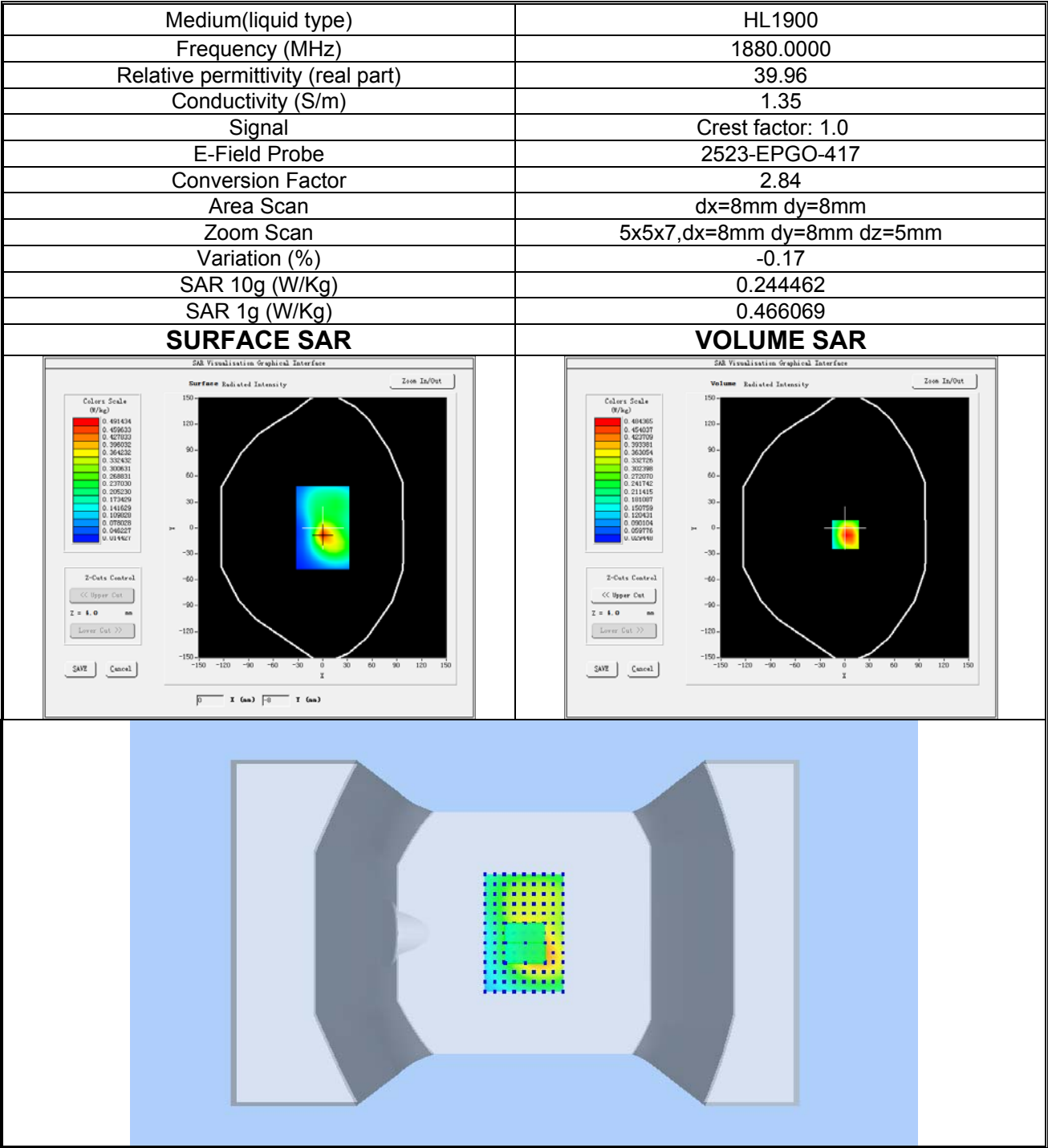
Plot 6: WCDMA BAND II, Middle channel (Body-worn /Hotspot, Back Side) Product Description: Smart Phone Test Date: 2024-10-12
