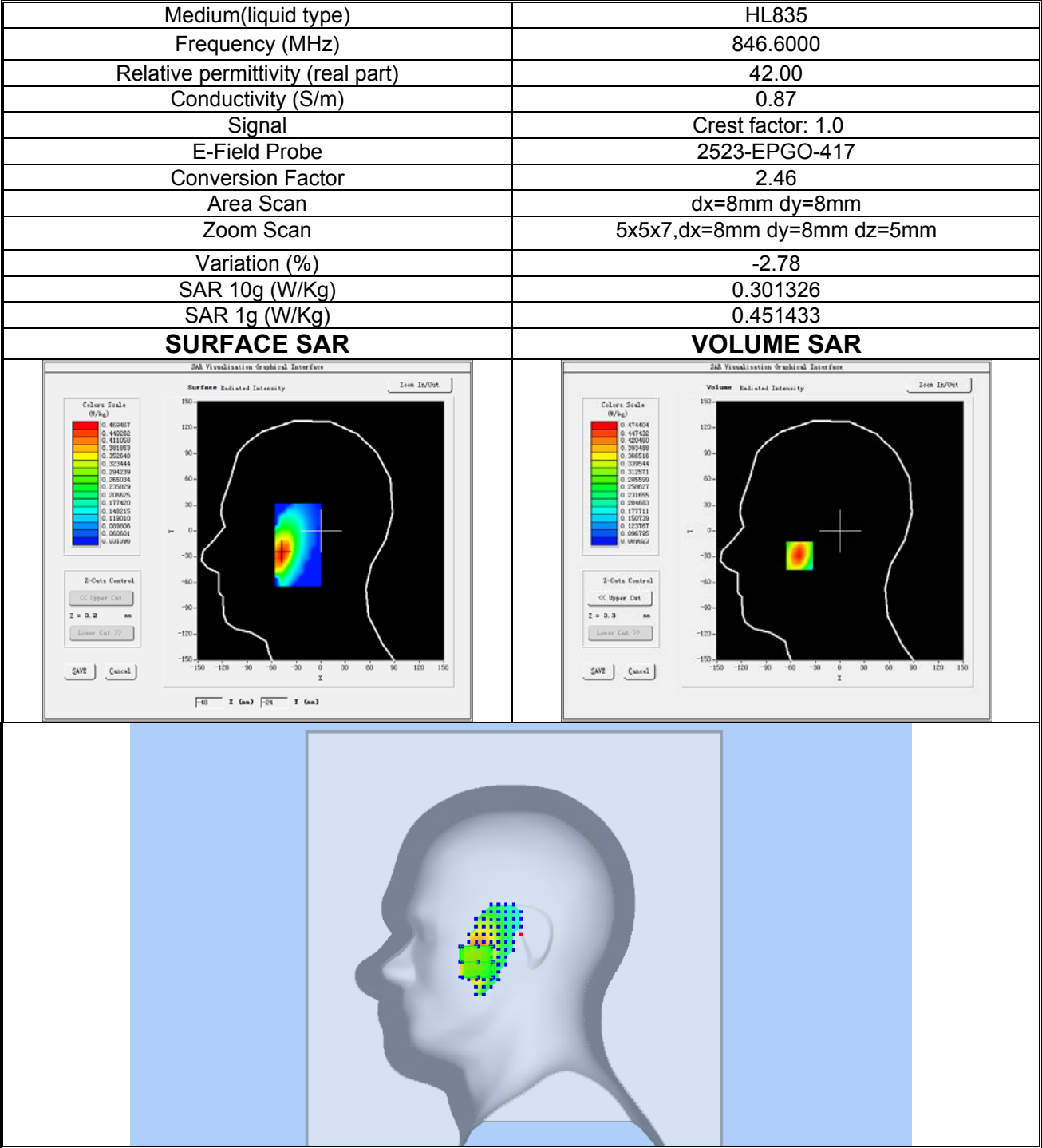
Plot 9: WCDMA BAND V, High channel (Right Head Cheek) Product Description: Smart Phone Test Date: 2024-10-14
