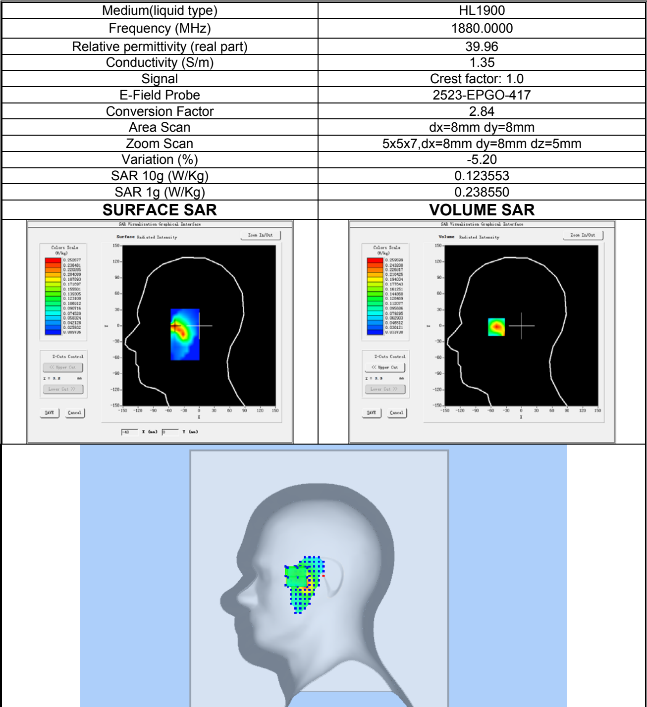
Plot 3: GPRS1900, Middle channel (Right Head Cheek) Product Description: Smart Phone Test Date: 2024-10-12
