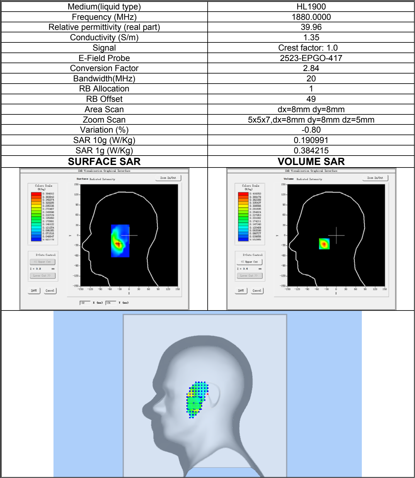
Plot 11:LTE BAND 2, Middle channel (Right Head Cheek) Product Description:Smart Phone Test Date: 2024-10-12
