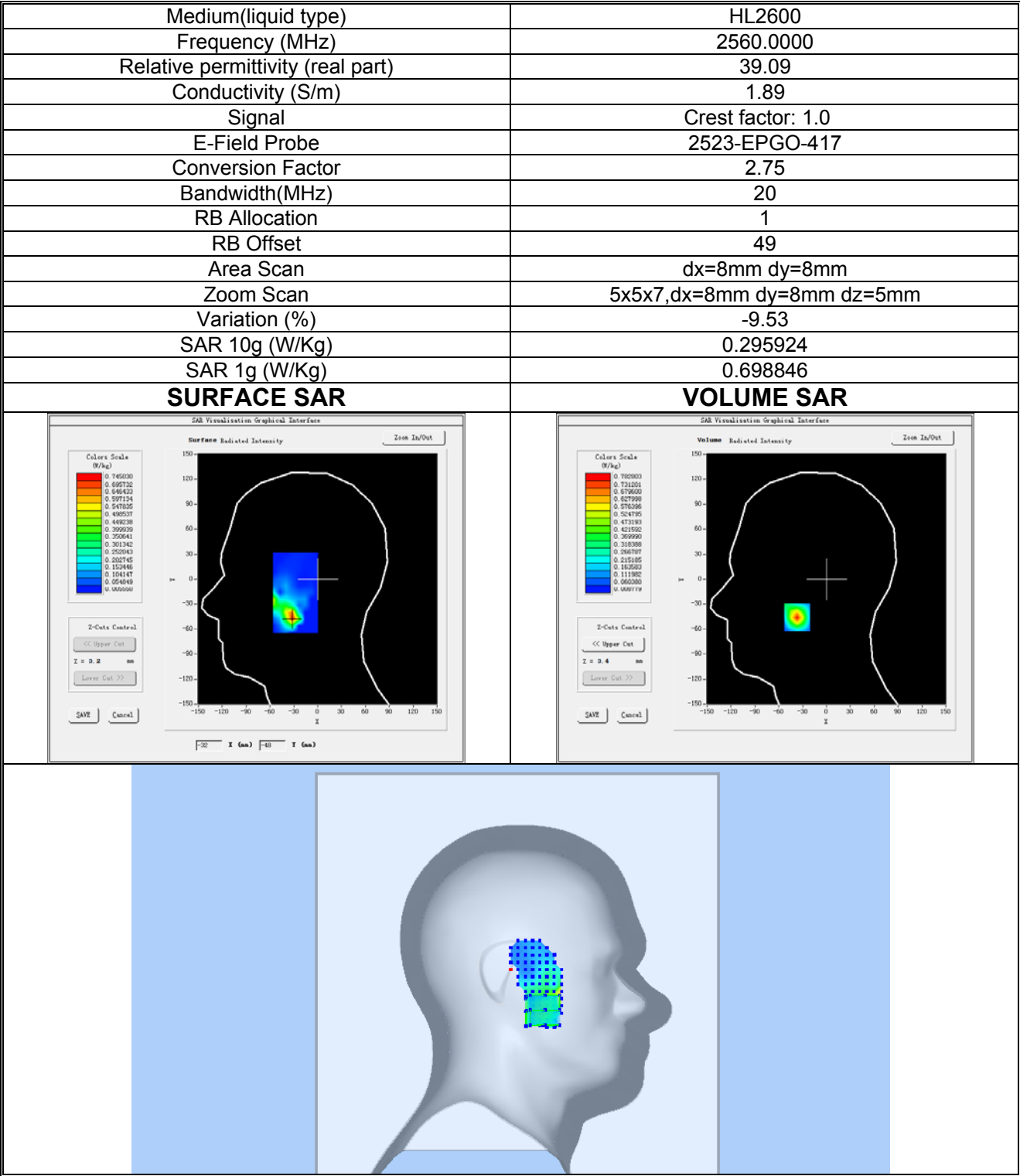
Plot 17:LTE BAND 7, High channel (Left Head Cheek) Product Description: Smart Phone Test Date: 2024-10-18
