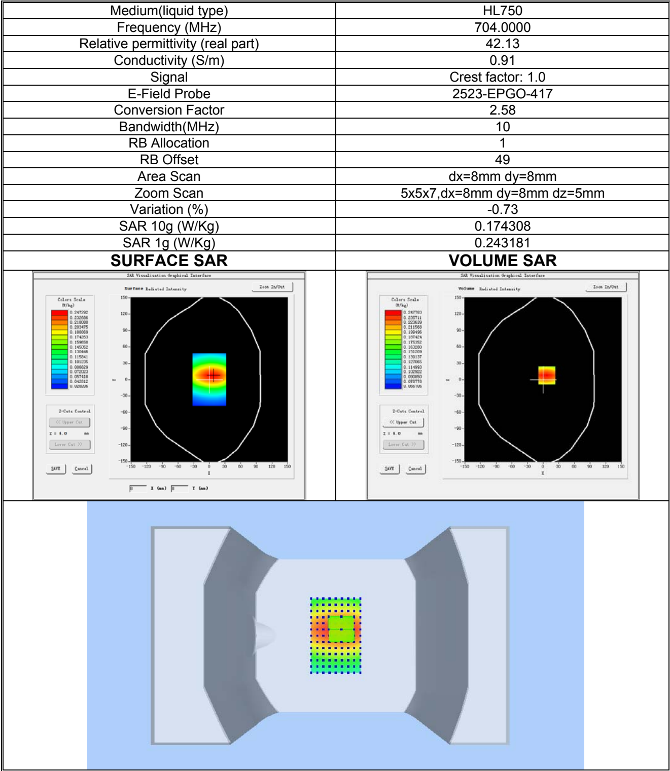
Plot 20: LTE BAND 12, Low channel (Body-worn/ Hotspot, Right Edge) Product Description: Smart Phone Test Date: 2024-10-15
