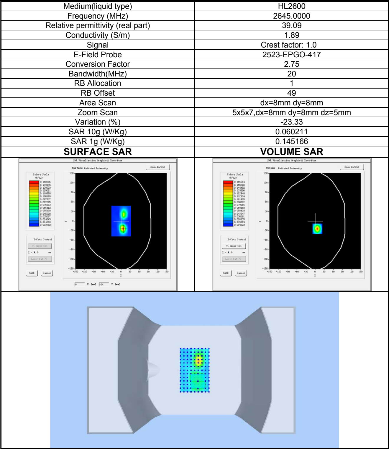
Plot 24: LTE BAND 41, High channel (Body-worn/ Hotspot, Bottom Edge) Product Description: Smart Phone Test Date: 2024-10-18
