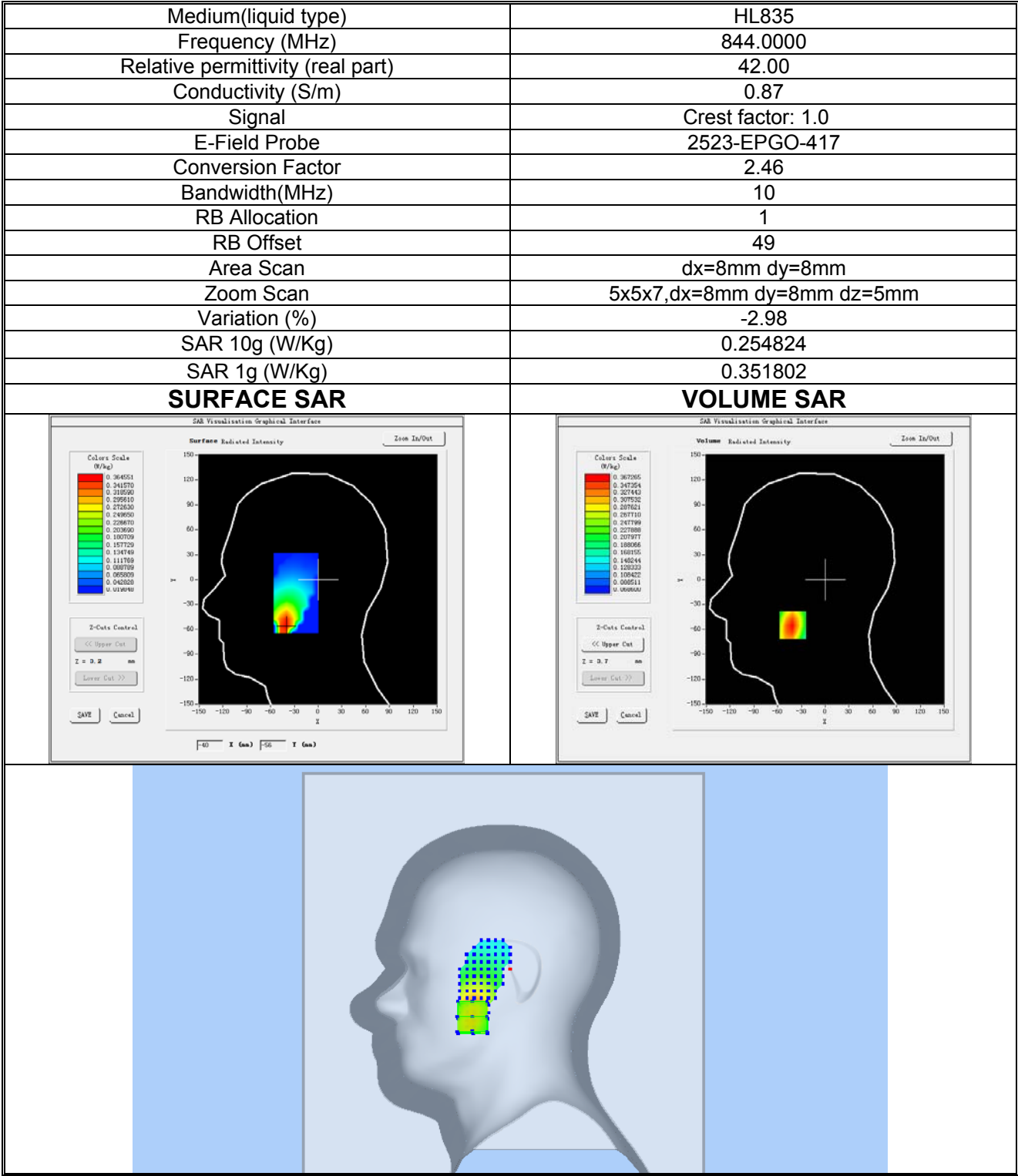
Plot 15:LTE BAND 5, High channel (Right Head Cheek) Product Description: Smart Phone Test Date: 2024-10-14
