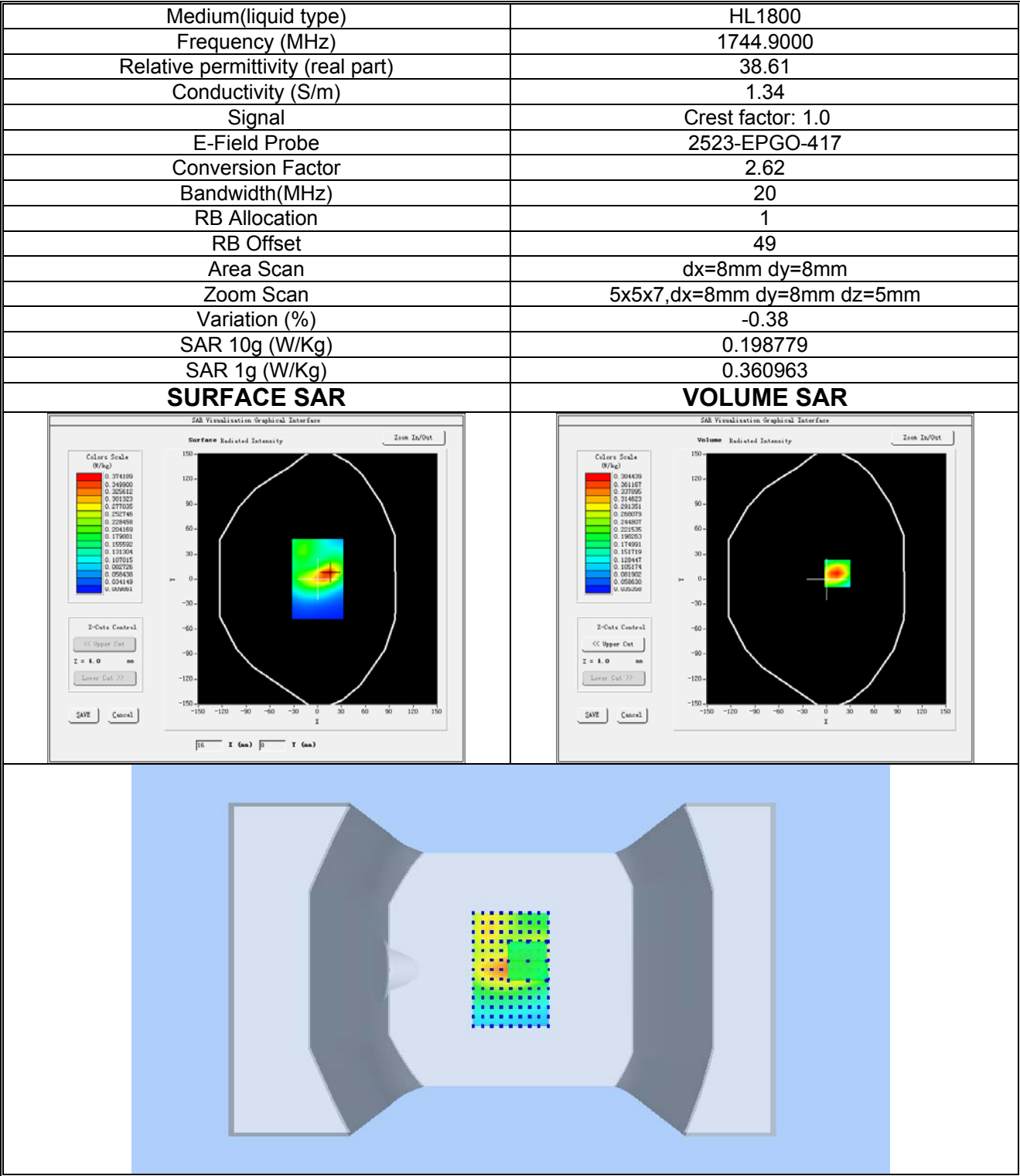
Plot 26: LTE BAND 66, Middle channel (Body-worn/ Hotspot, Back Side) Product Description: Smart Phone Test Date: 2024-10-21
