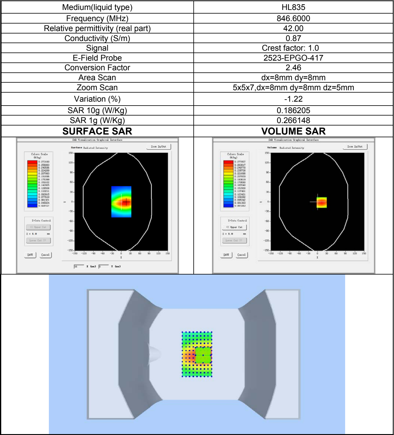
Plot 10: WCDMA BAND V, High channel (Body-worn/Hotspot, Left Edge) Product Description: Smart Phone Test Date: 2024-10-14
