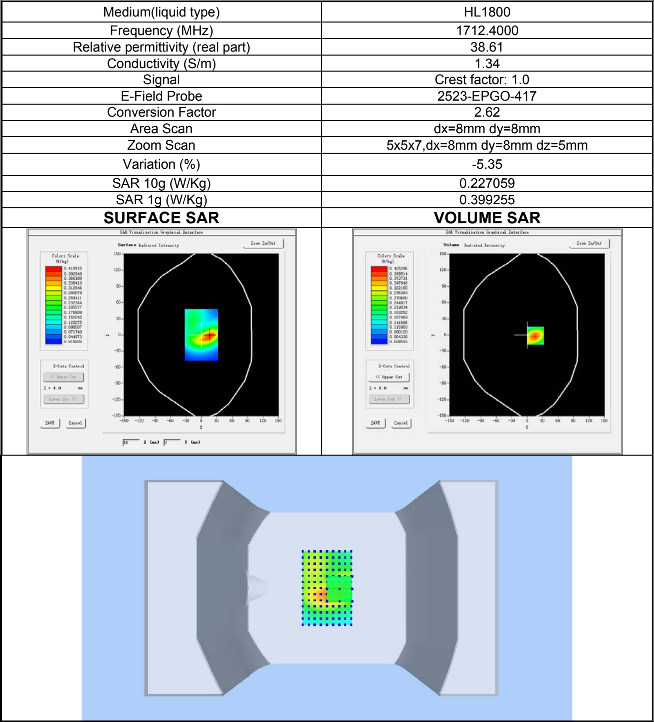
Plot 8: WCDMA BAND IV, Low channel (Body-worn/Hotspot, Back Side) Product Description: Smart Phone Test Date: 2024-10-21
