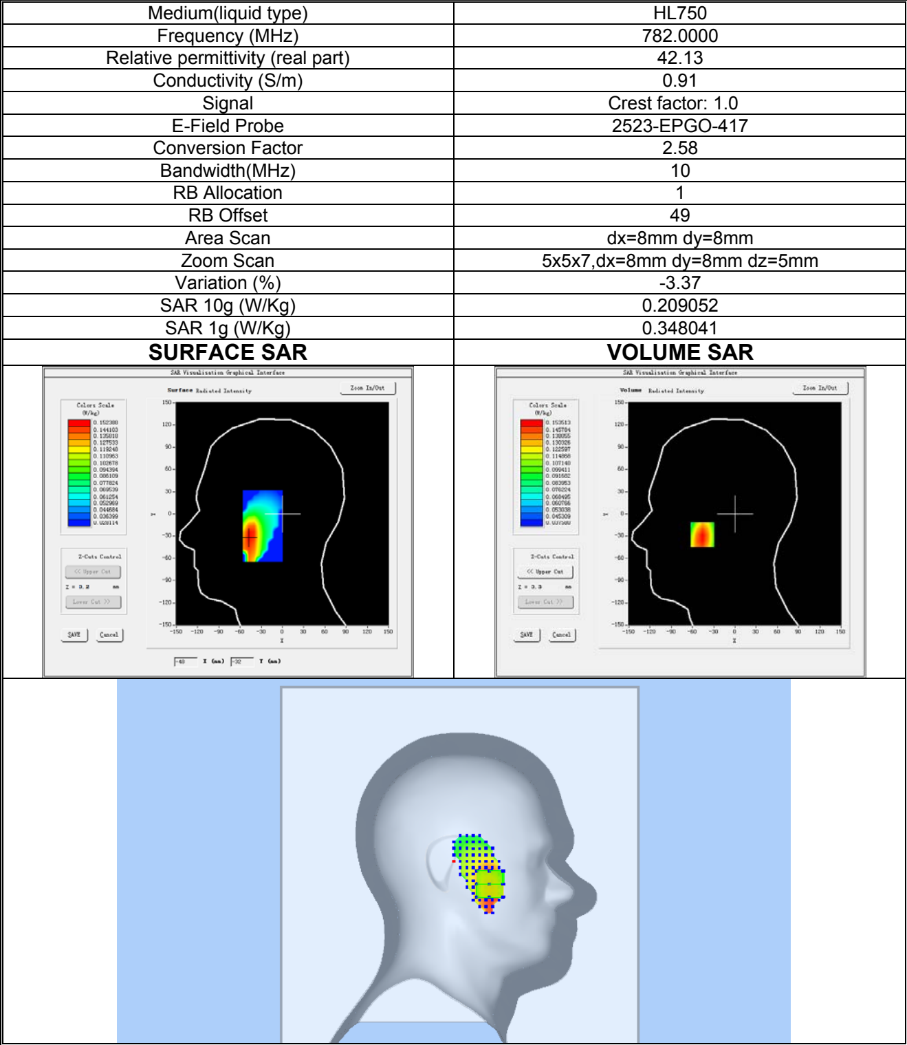
Plot 21:LTE BAND 13, Low channel (Left Head Cheek) Product Description: Smart Phone Test Date: 2024-10-15
