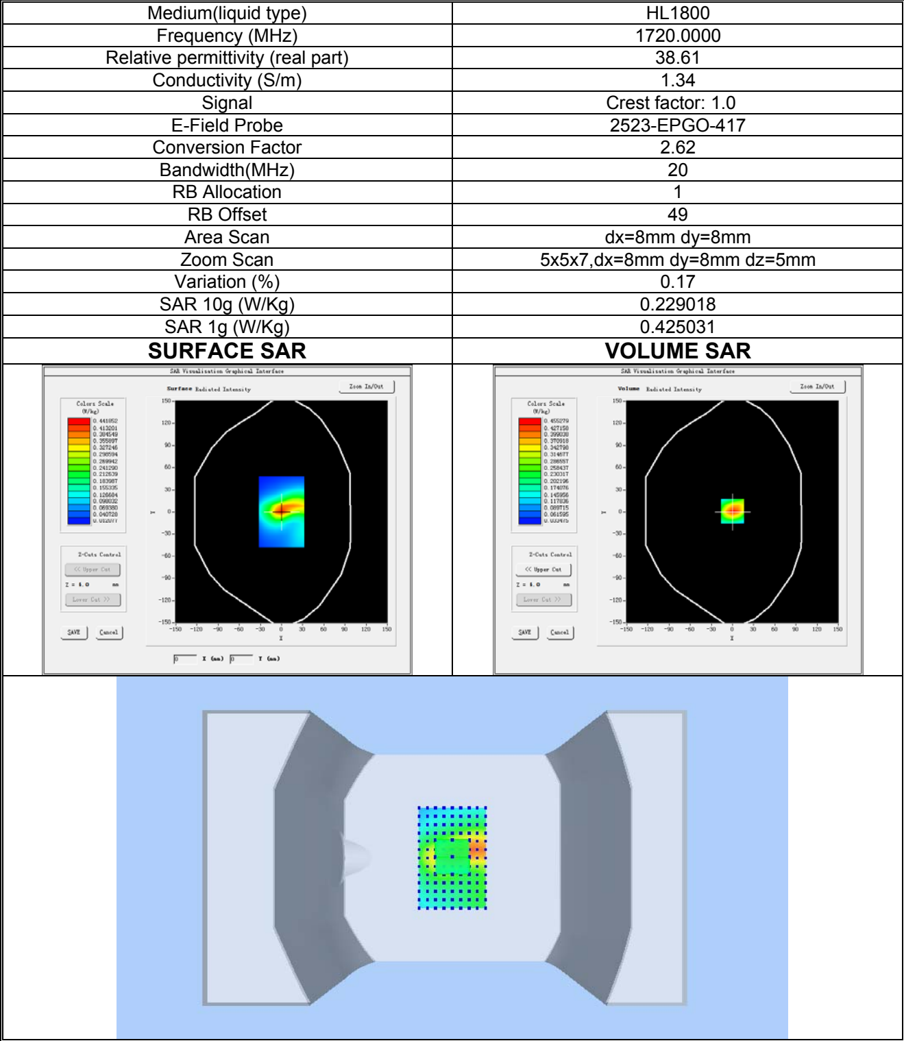
Plot 14: LTE BAND 4, Low channel (Body-worn/ Hotspot, Back Side) Product Description: Smart Phone Test Date: 2024-10-21
