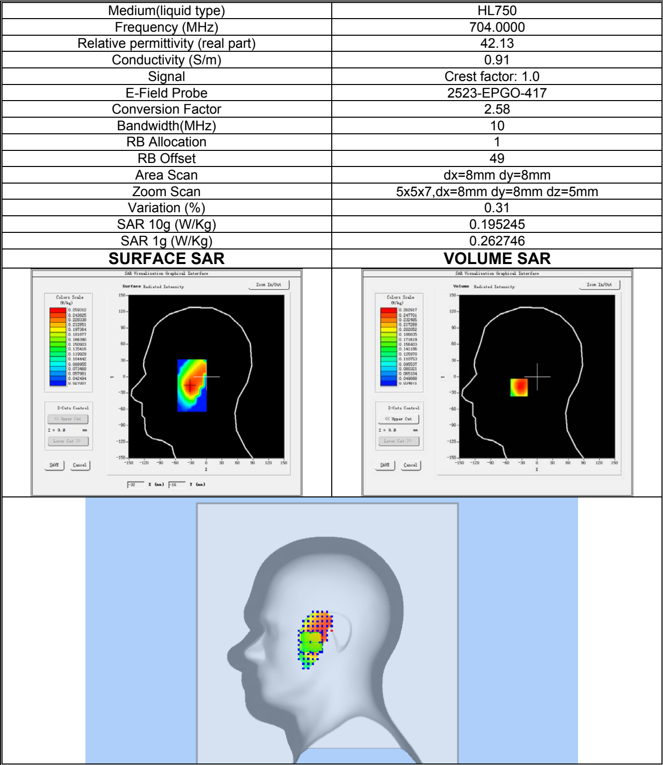
Plot 19:LTE BAND 12, Low channel (Right Head Cheek) Product Description: Smart Phone Test Date: 2024-10-15
