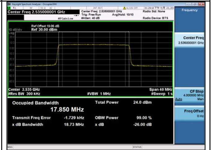
LTE band 7 - Middle CH 16QAM-20
