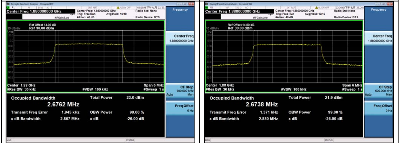
LTE band 2 - Middle CH QPSK-3
