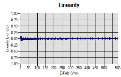
Linearity: +/-1.43% (+/-0.06dB)
