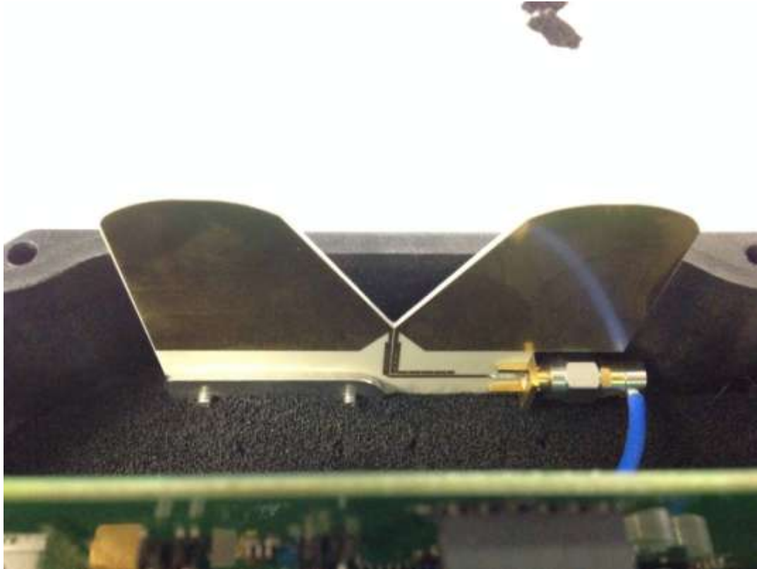
Figure 5. Bowtie Antenna
