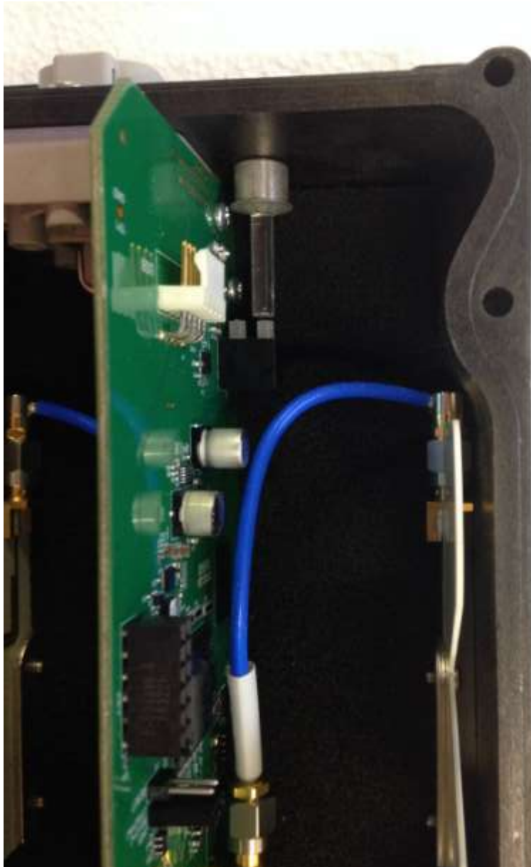
Figure 7. EUT with no USB Access (HT5200)
