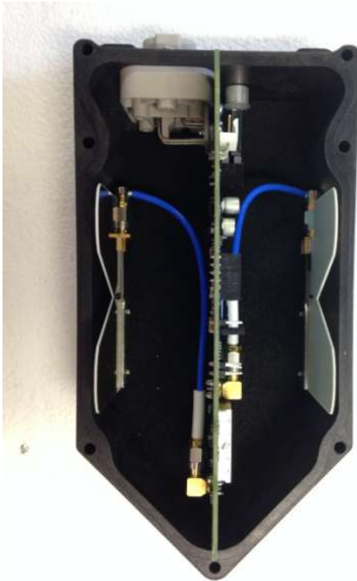
Figure 6. EUT with no USB Access (Top view)
