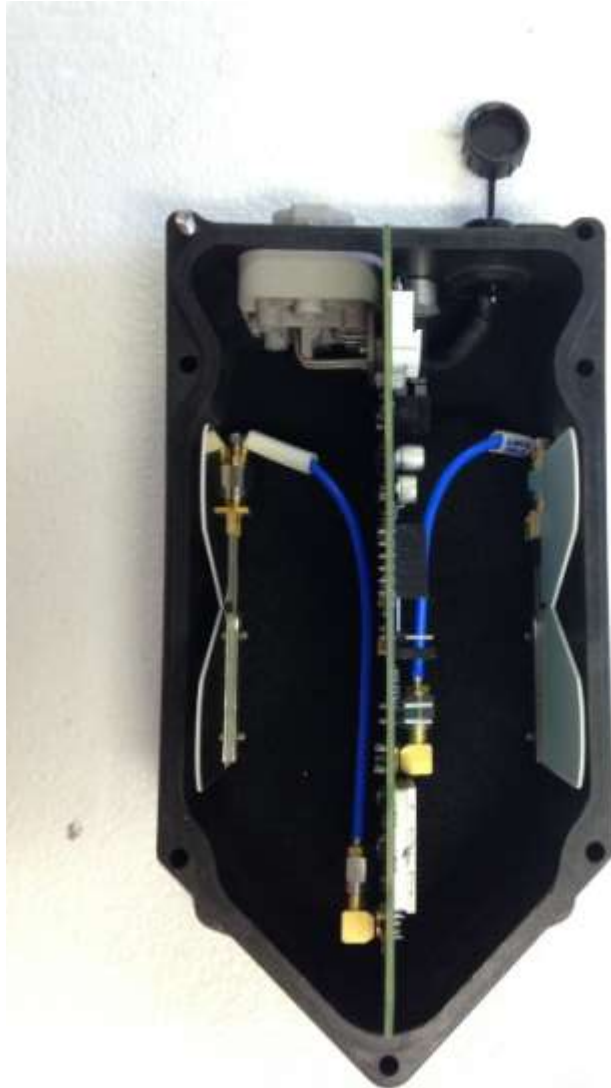
Figure 8. EUT with USB Access Port (Top View)
