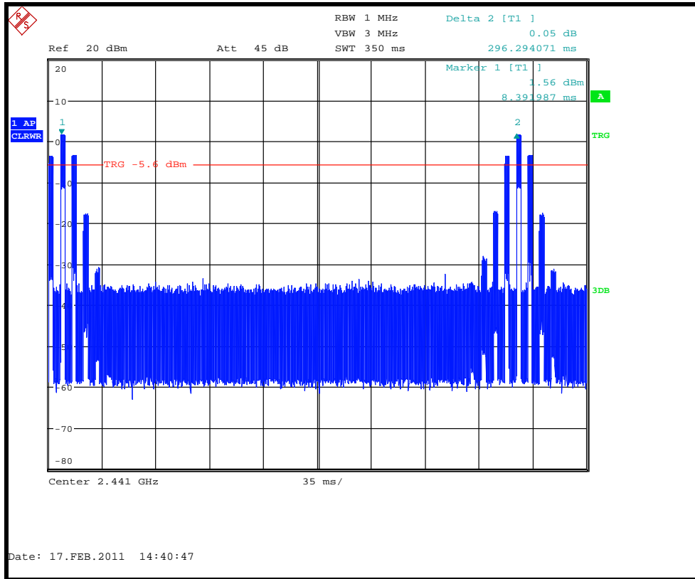
Channel repetition time – 3Mbps
