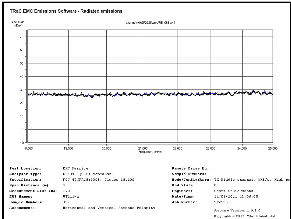
Radiated Spurious emissions 18 GHz to 25 GHz – 2441MHz – 3Mbps
