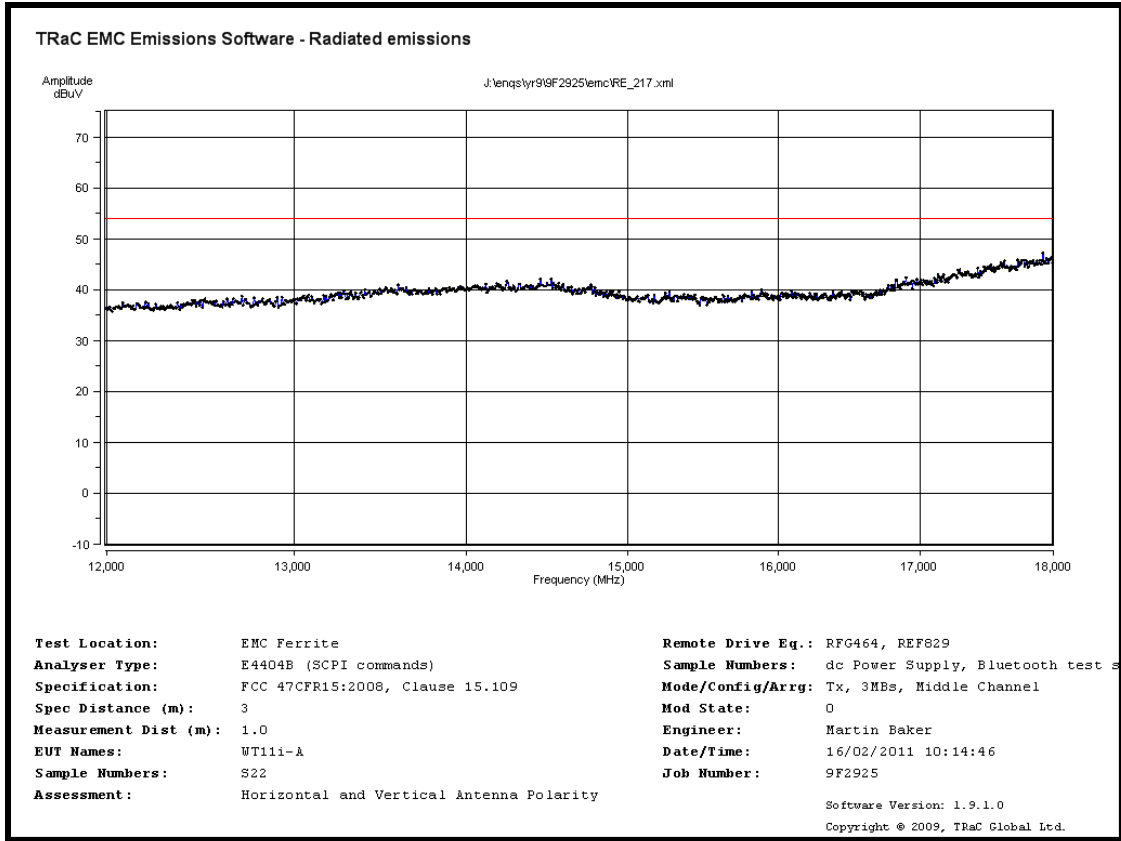
Radiated Spurious emissions 12 GHz to 18 GHz – 2441MHz – 3Mbps
