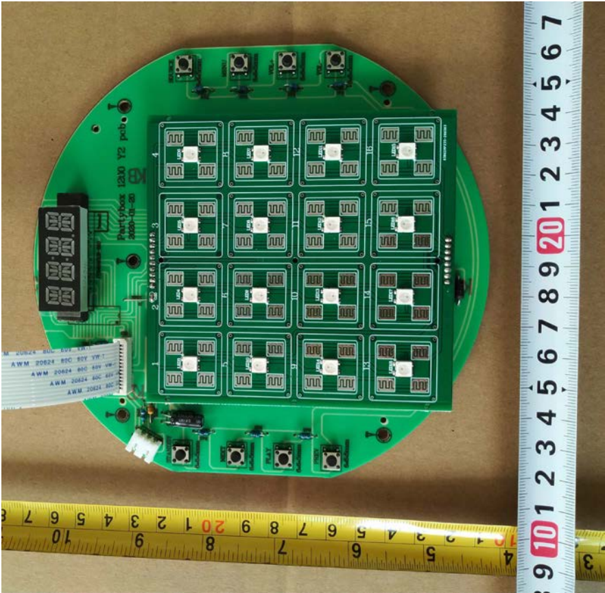
Solder Board-Component View 10
