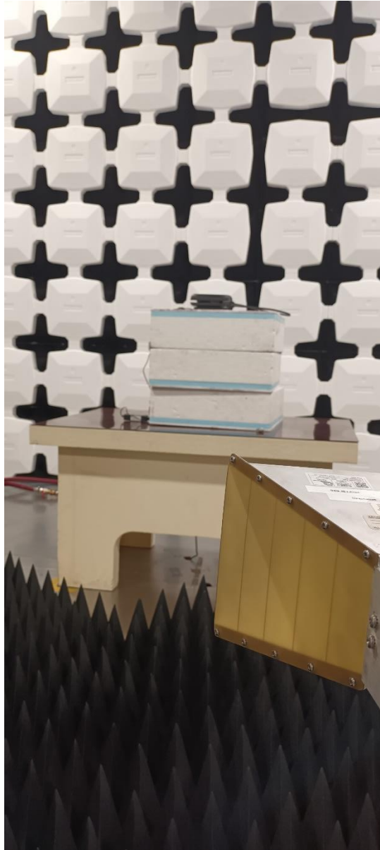
Photo 4 Photograph test setup radiated emissions 1-18 GHz
