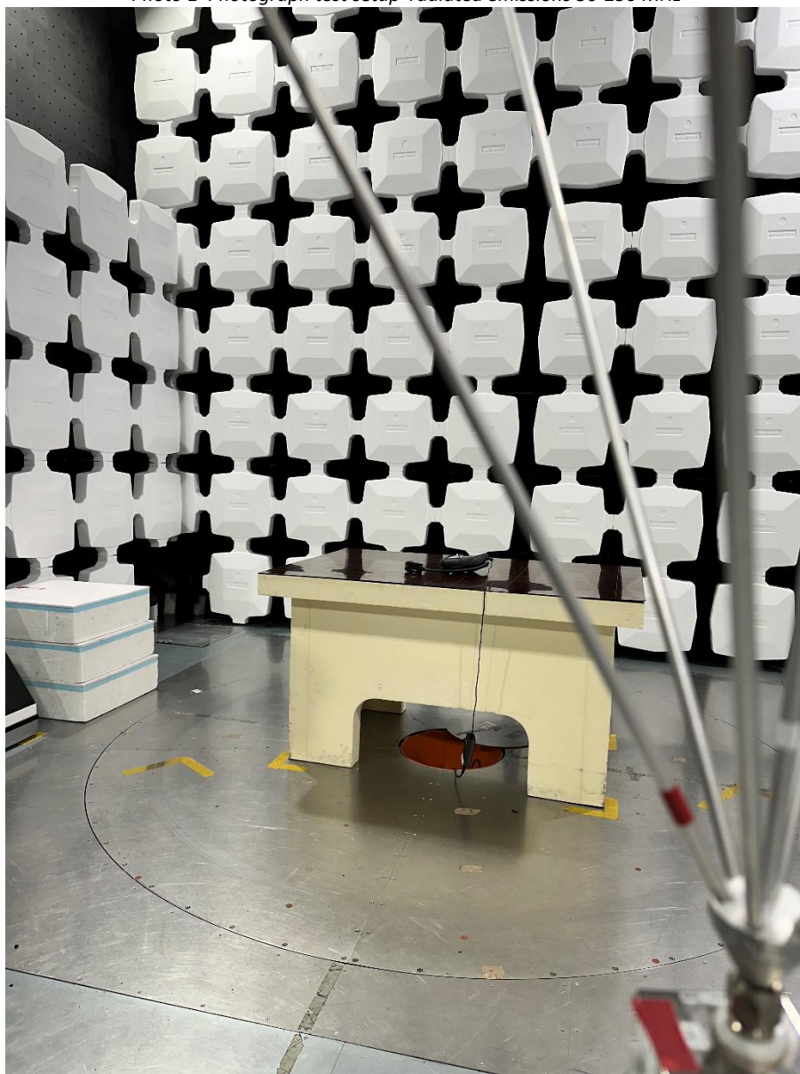
Photo 1 Photograph test setup radiated emissions 30-250 MHz
