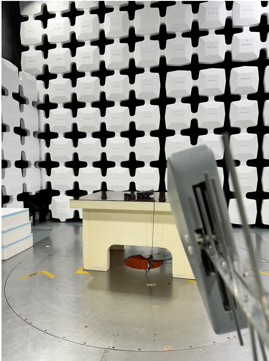
Photo 2 Photograph test setup radiated emissions 250-1000 MHz
