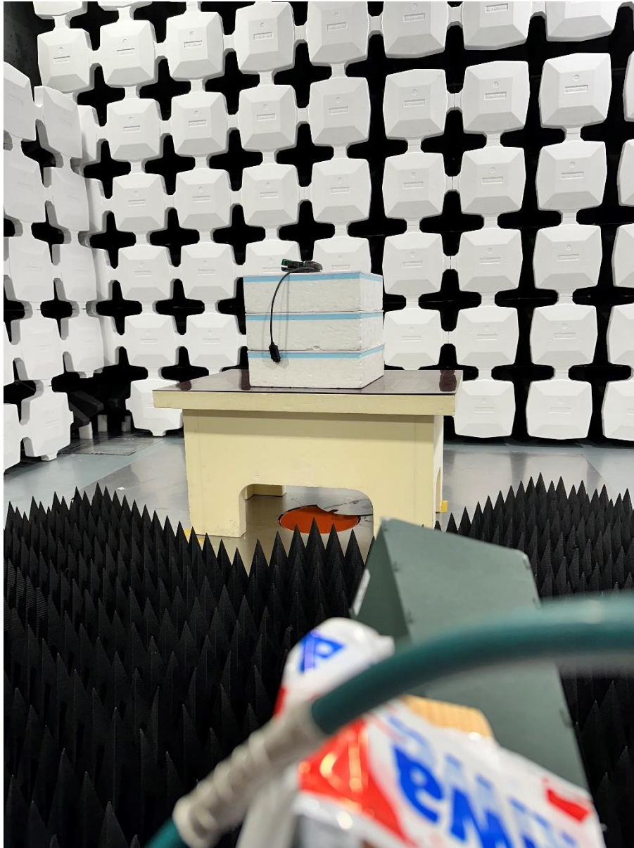
Photo 5 Photograph test setup radiated emissions 18- 26 GHz
