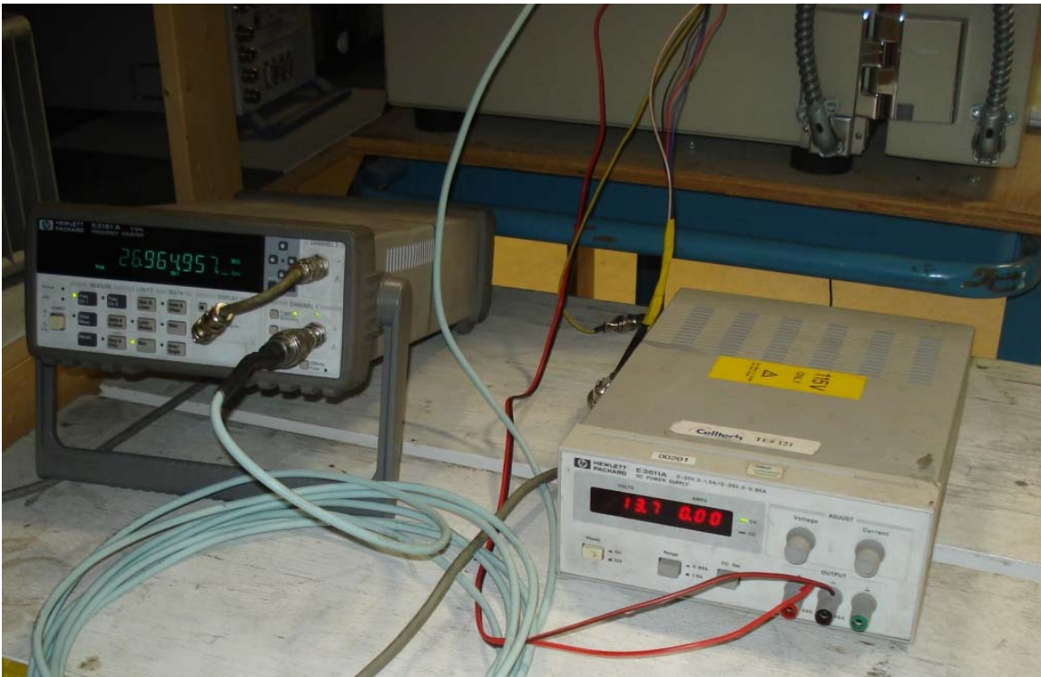
Figure 3 – Frequency Stability
