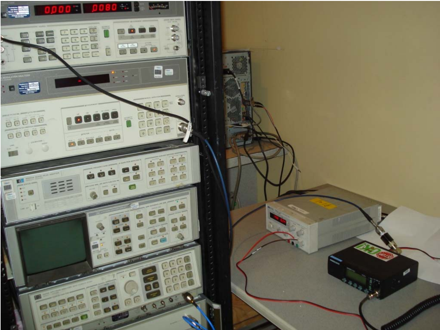
Figure 1 – Modulation Characteristics
