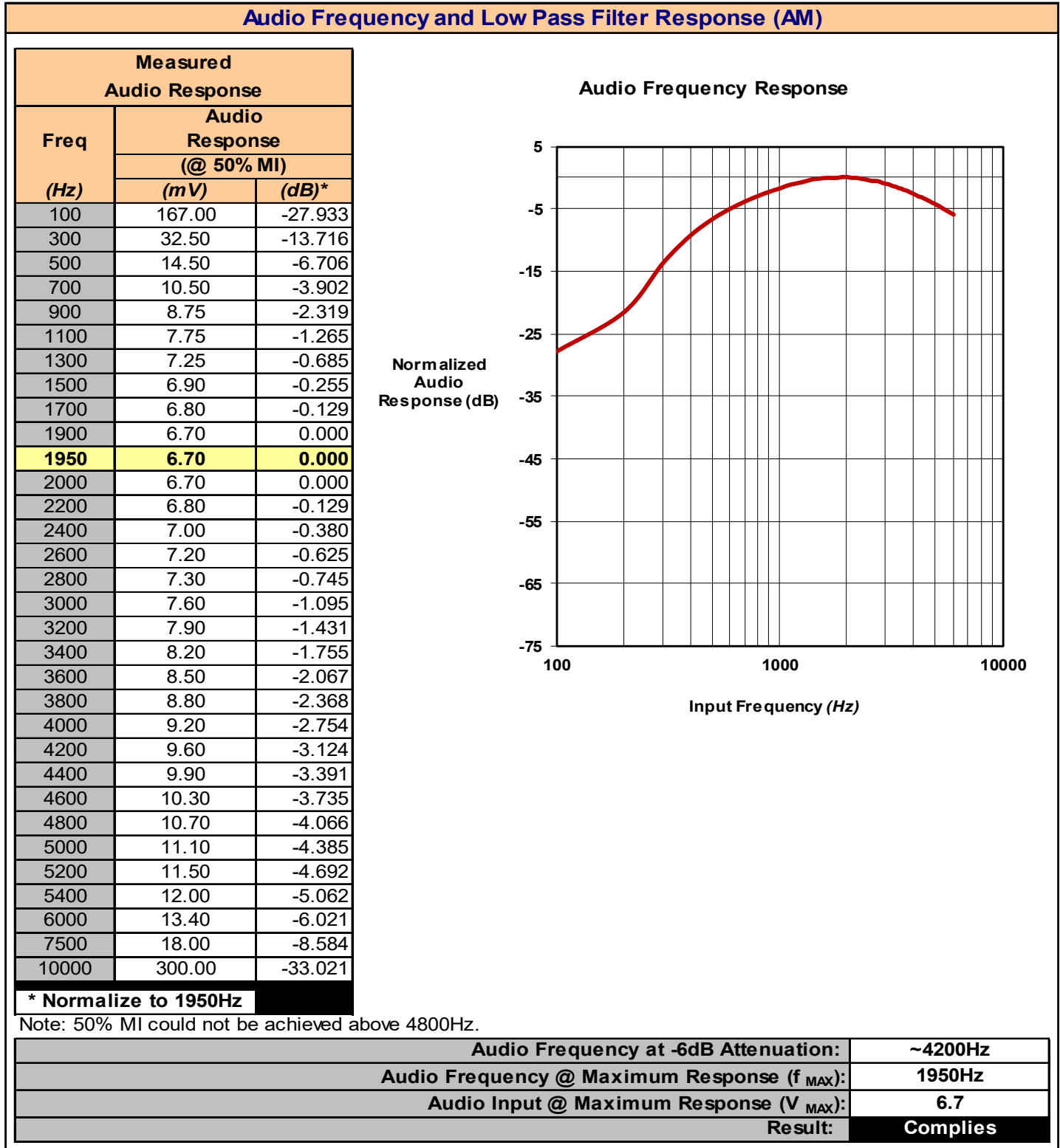
Plot 8.1 – Audio Frequency and Low Pass Filter Response, AM
