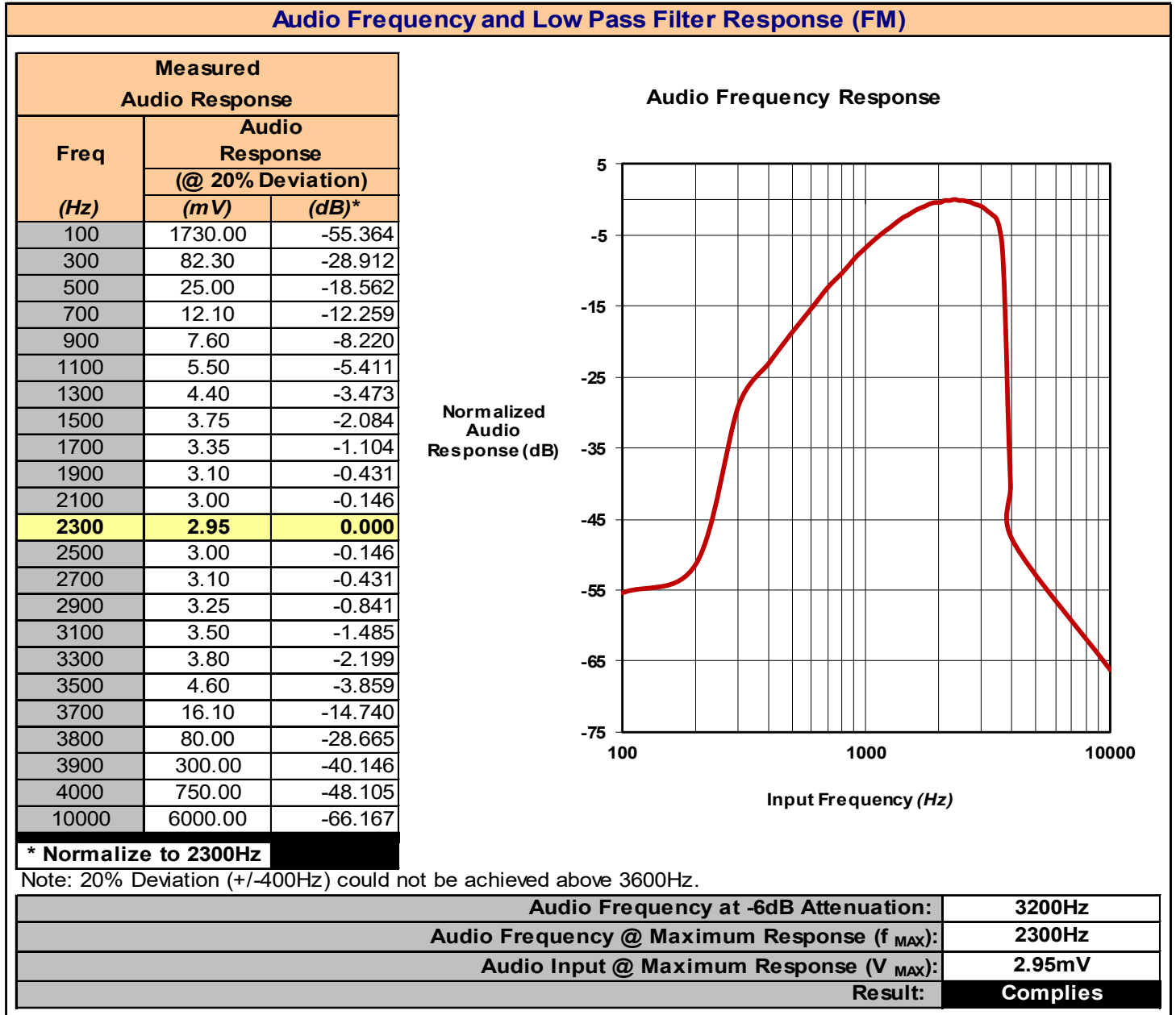
Plot 8.3 – Audio Frequency and Low Pass Filter Response, FM
