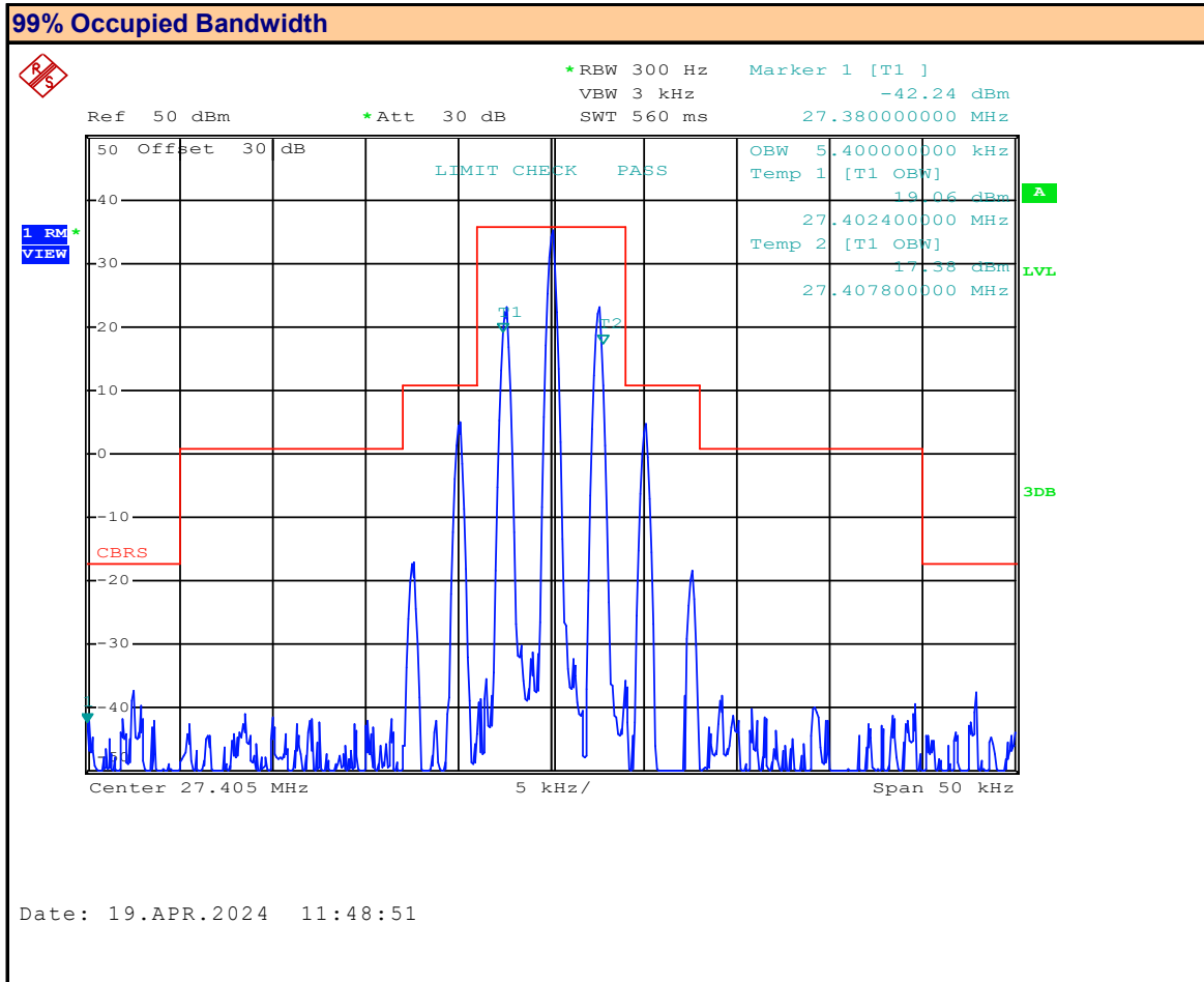
Plot 9.6 – Occupied Bandwidth, Channel 40, FM
