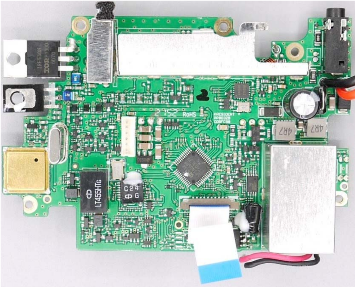
Figure E16.4 – Internal – PCB Top
