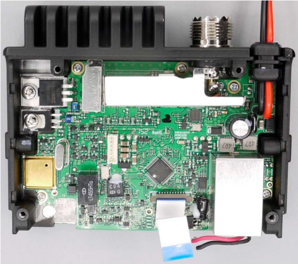
Figure E16.2 – Internal – Top Removed
