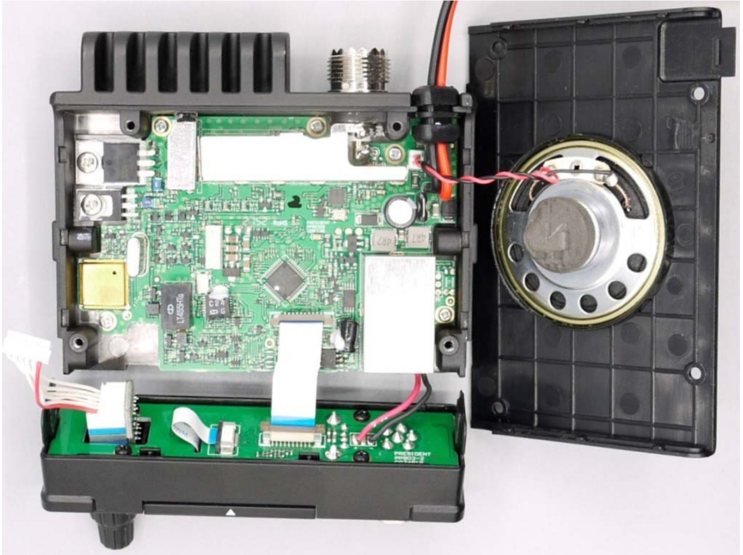
Figure E16.1 – Internal – Bottom Removed
