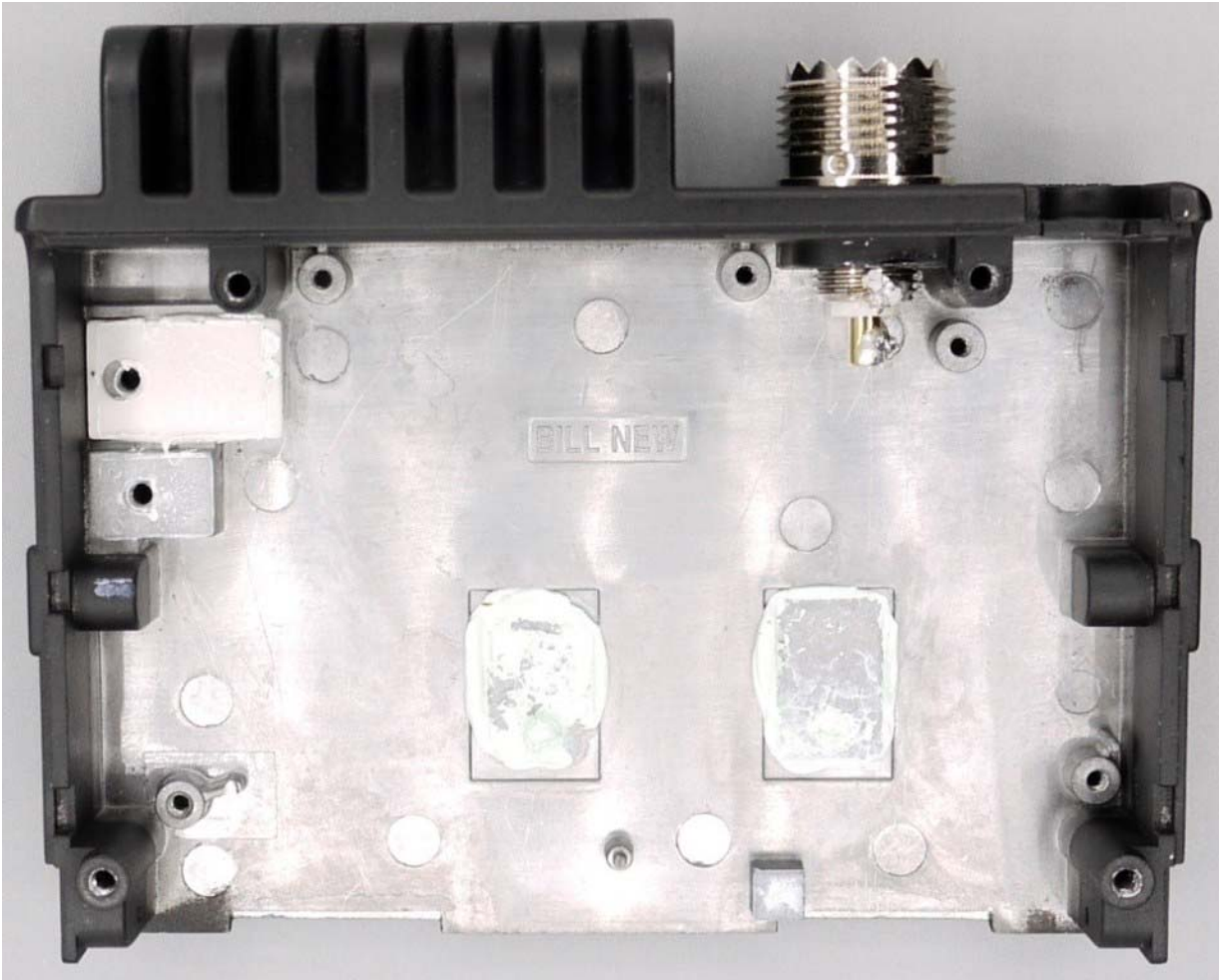
Figure E16.3 – Internal – Heat Sink
