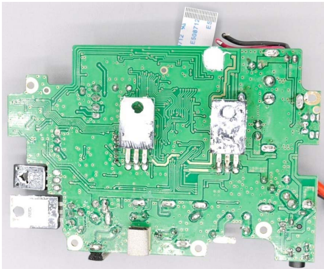
Figure E16.6 – Internal – PCB Bottom
