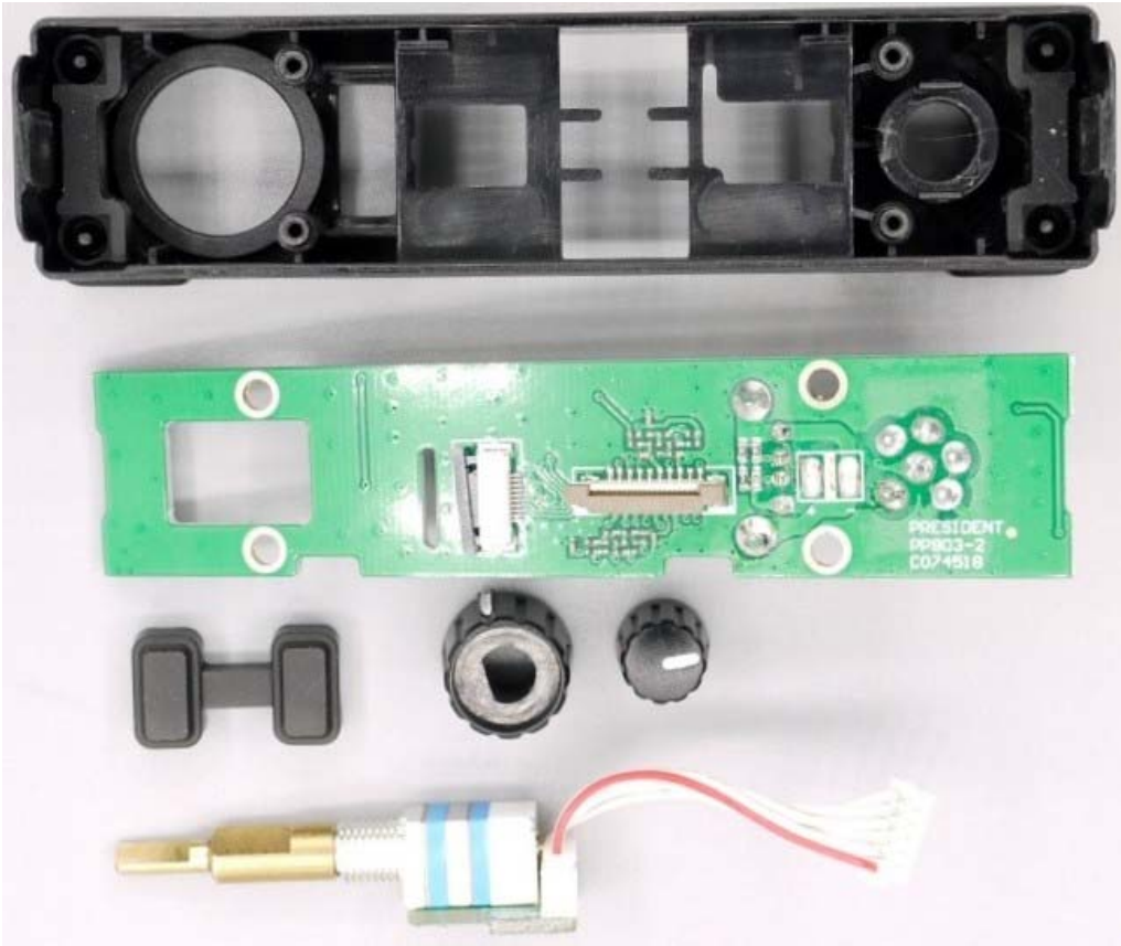
Figure E16.7 – Internal – Front Controls, Rear View
