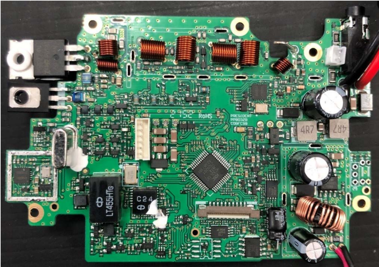
Figure E16.5 – Internal – PCB Top, Shields Removed
