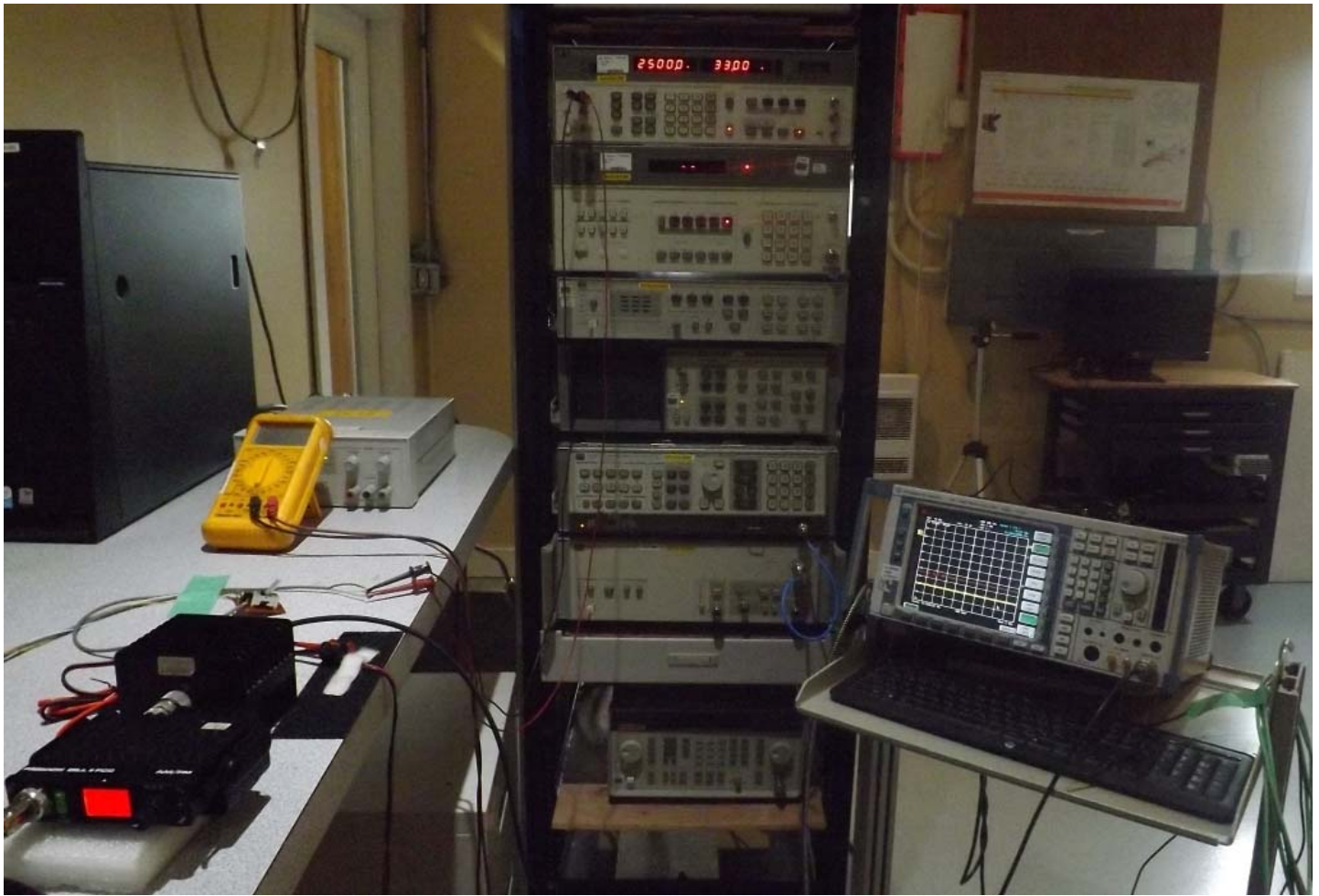
Figure E17.3 – Setup, Conducted Power
