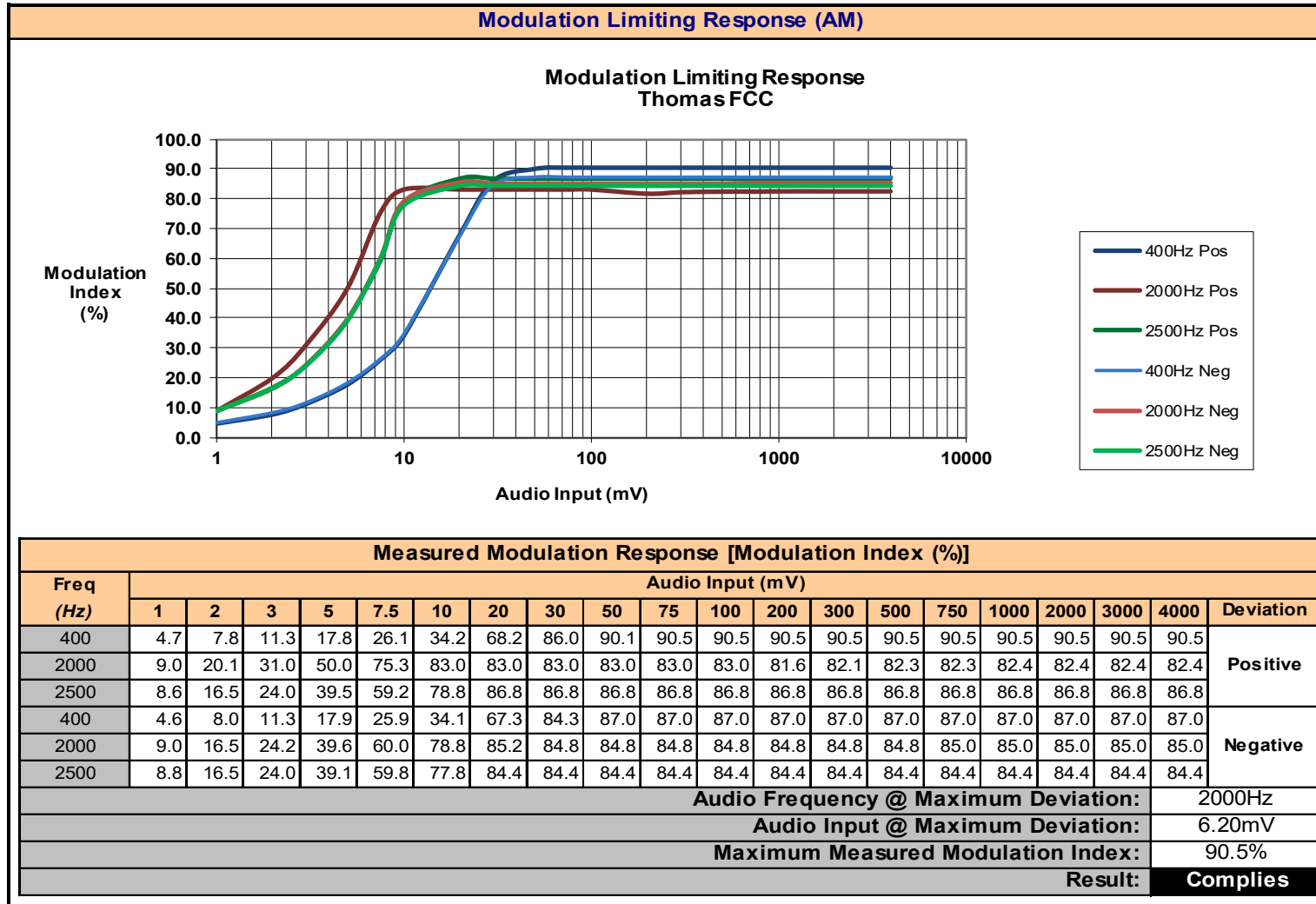
Plot 8.2 – Modulation Limiting Response, AM
