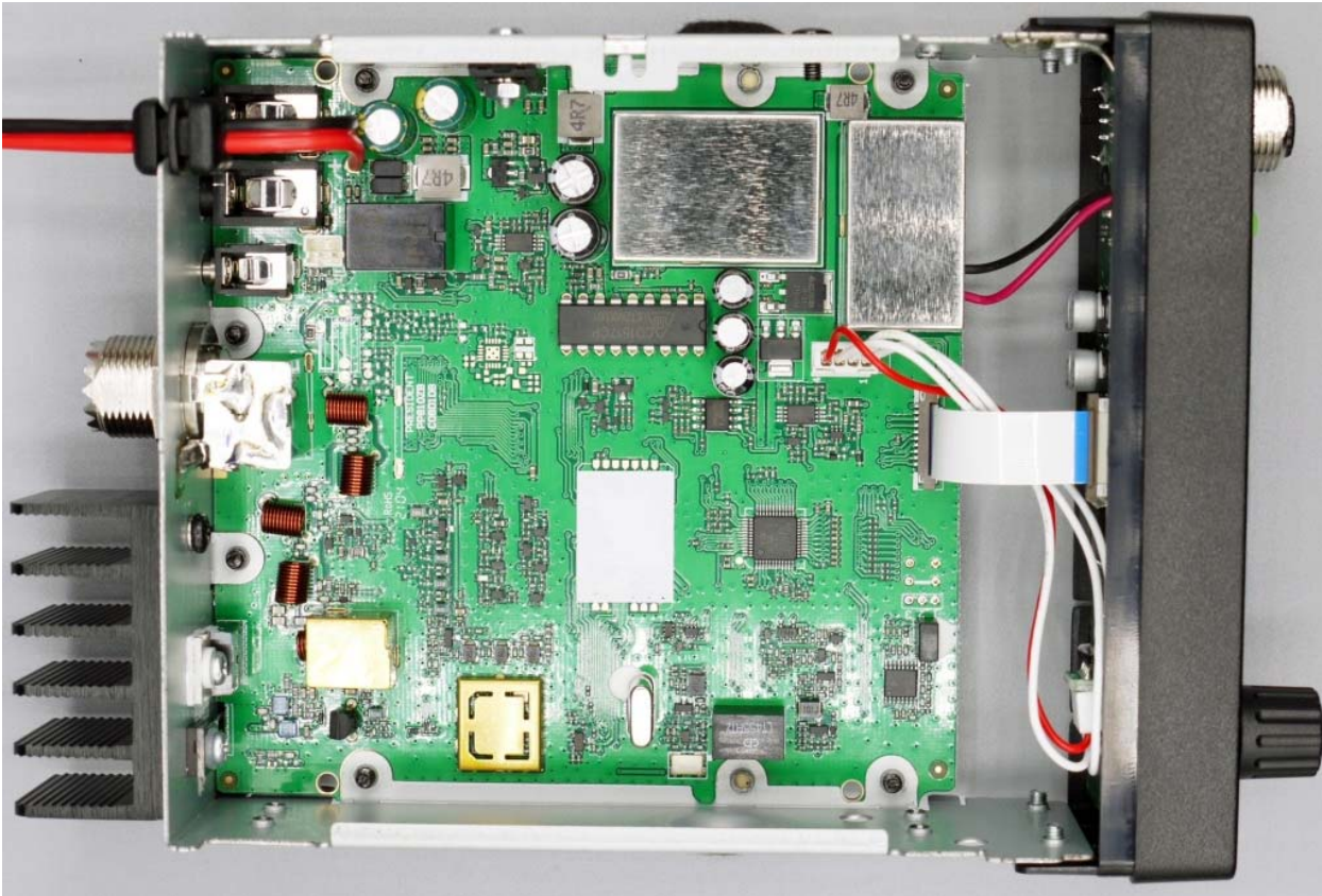
Figure E22.3 – Internal, PCB Top
