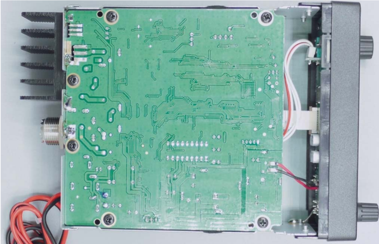
Figure E22.1 – Internal, PCB Bottom
