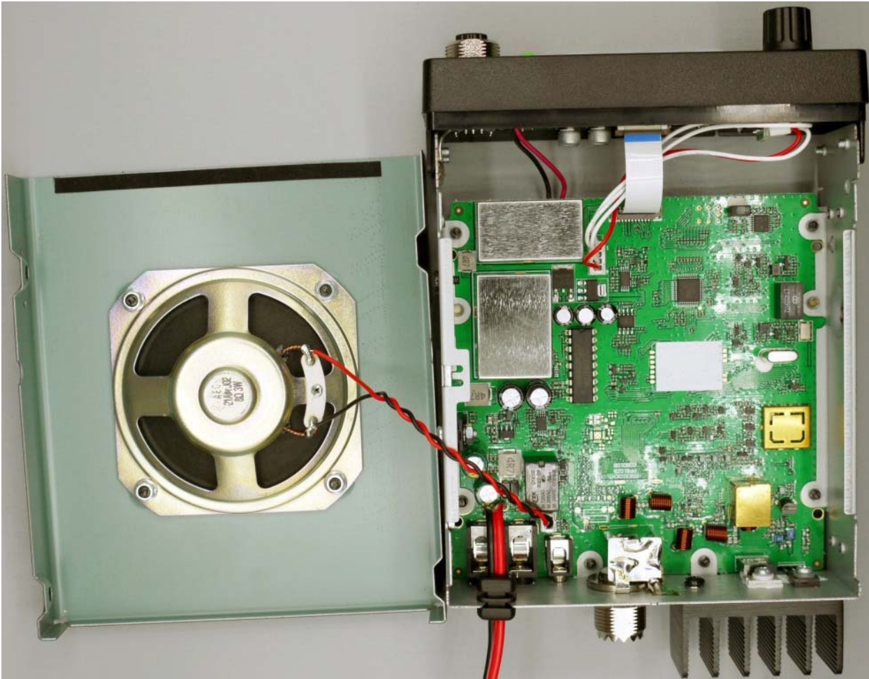
Figure E22.2 – Internal, Bottom Cover Removed
