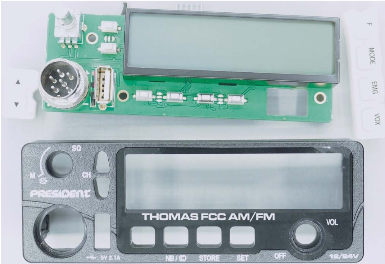
Figure E22.5 – Internal, Front Display Components, Front Side
