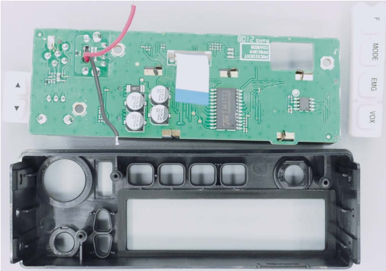
Figure E22.6 – Internal, Front Display Components, Back Side
