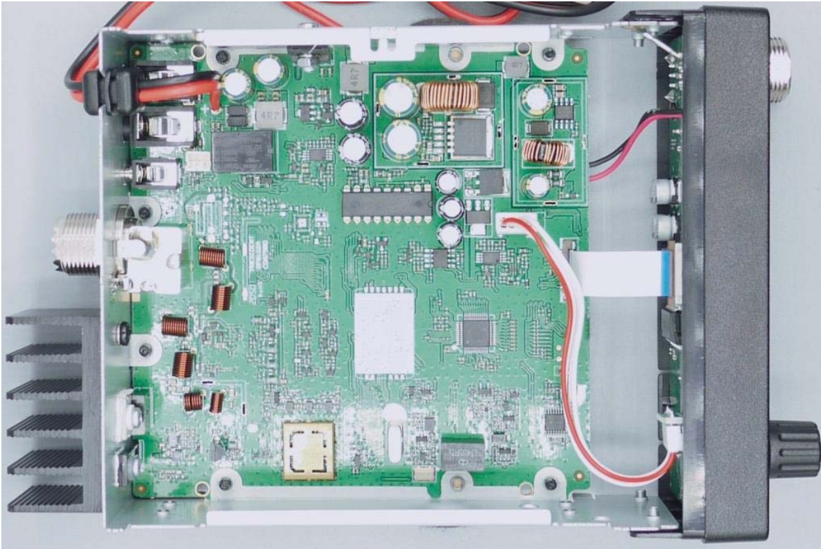
Figure E22.4 – Internal, PCB Bottom – Shields Removed
