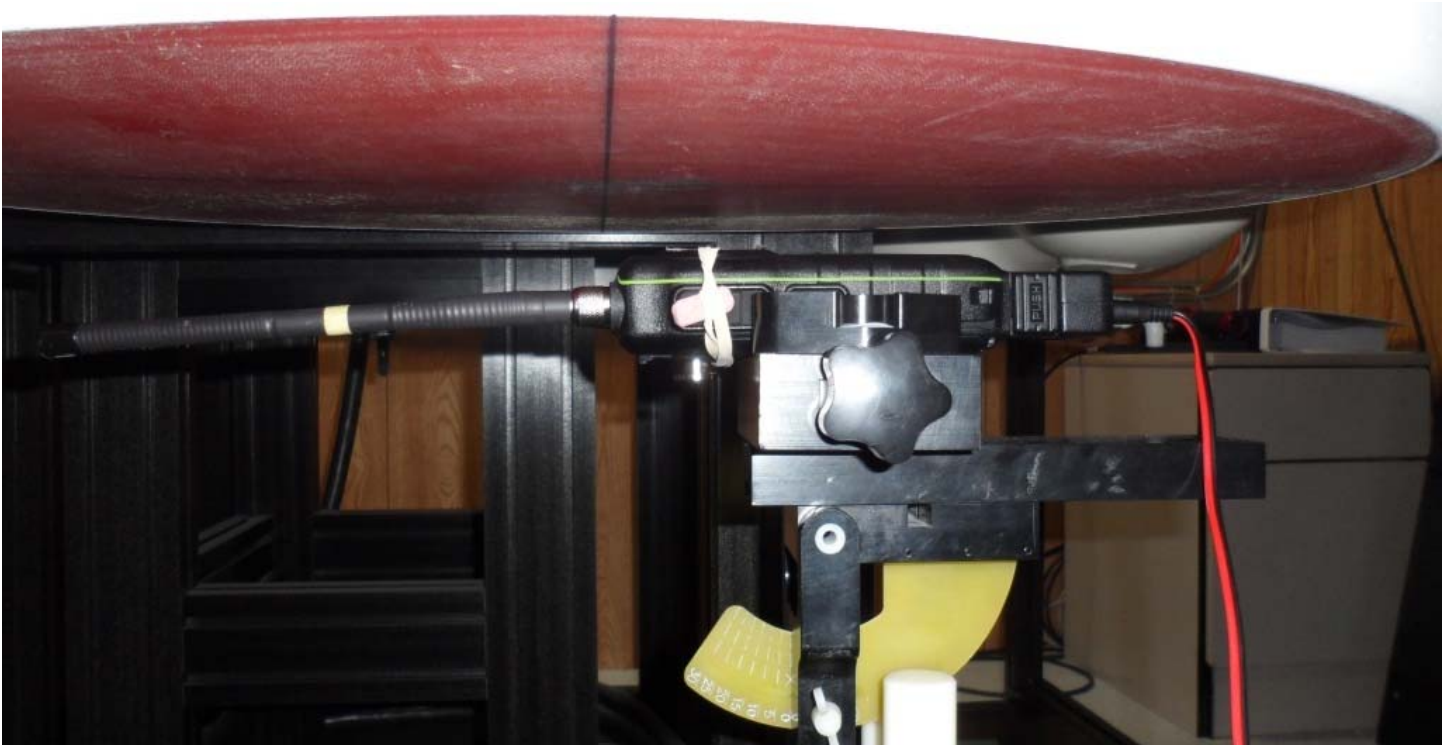
Figure E25.6 – Setup Photo – Face Configuration w/ Automotive Adapter, Enlarged
