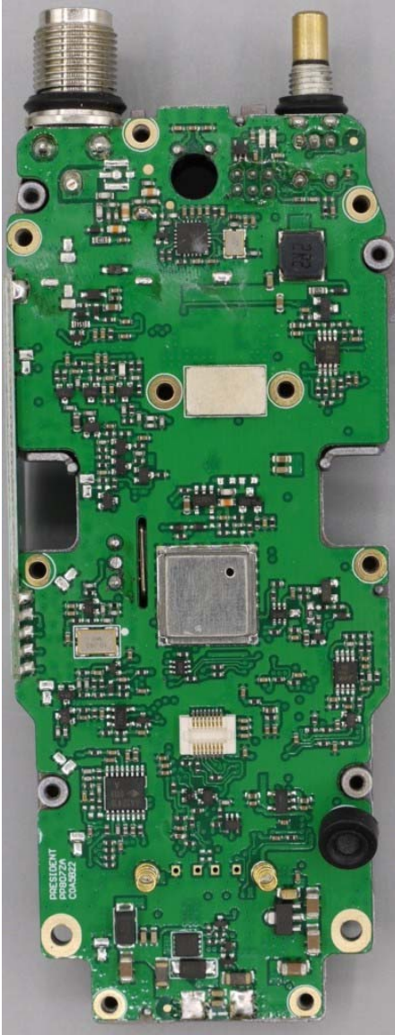
Figure E23.4 – Internal Photo – Main PCB Bottom
