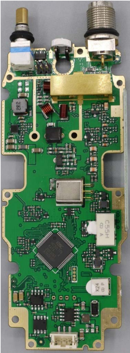
Figure E23.3 – Internal Photo – Main PCB Top
