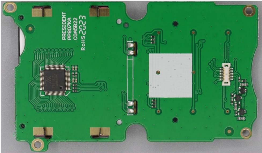
Figure E23.9 – Internal Photo – Battery Controller PCB
