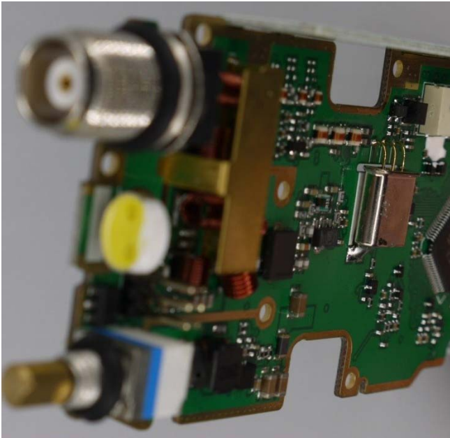
Figure E23.5 – Internal Photo – Main PCB Top End
