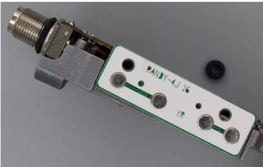
Figure E23.6 – Internal Photo – Side Pushbuttons
