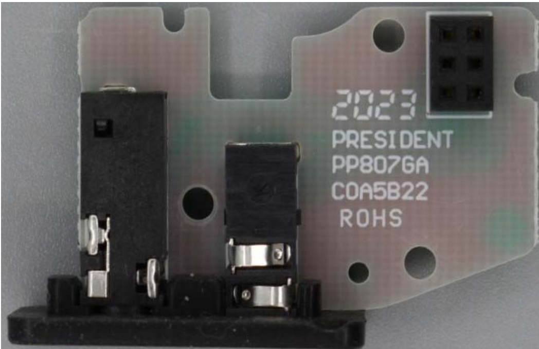
Figure E23.8 – Internal Photo – Accessory PCB Top
