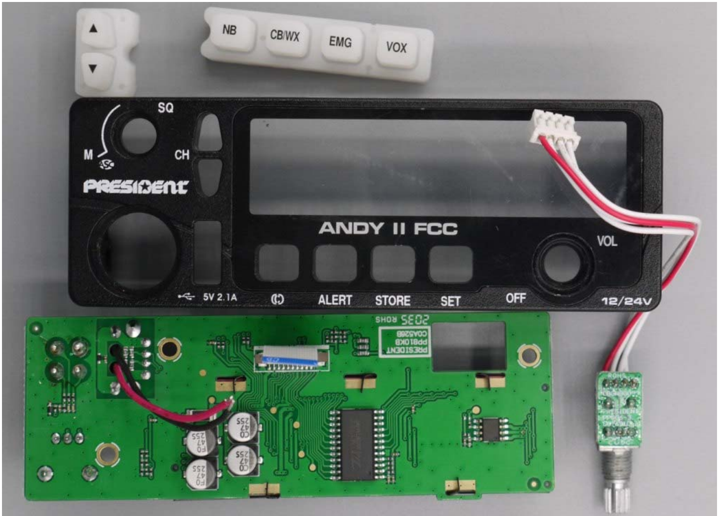
Figure E20.4 – Internal Photo – Front Assembly – Front View
