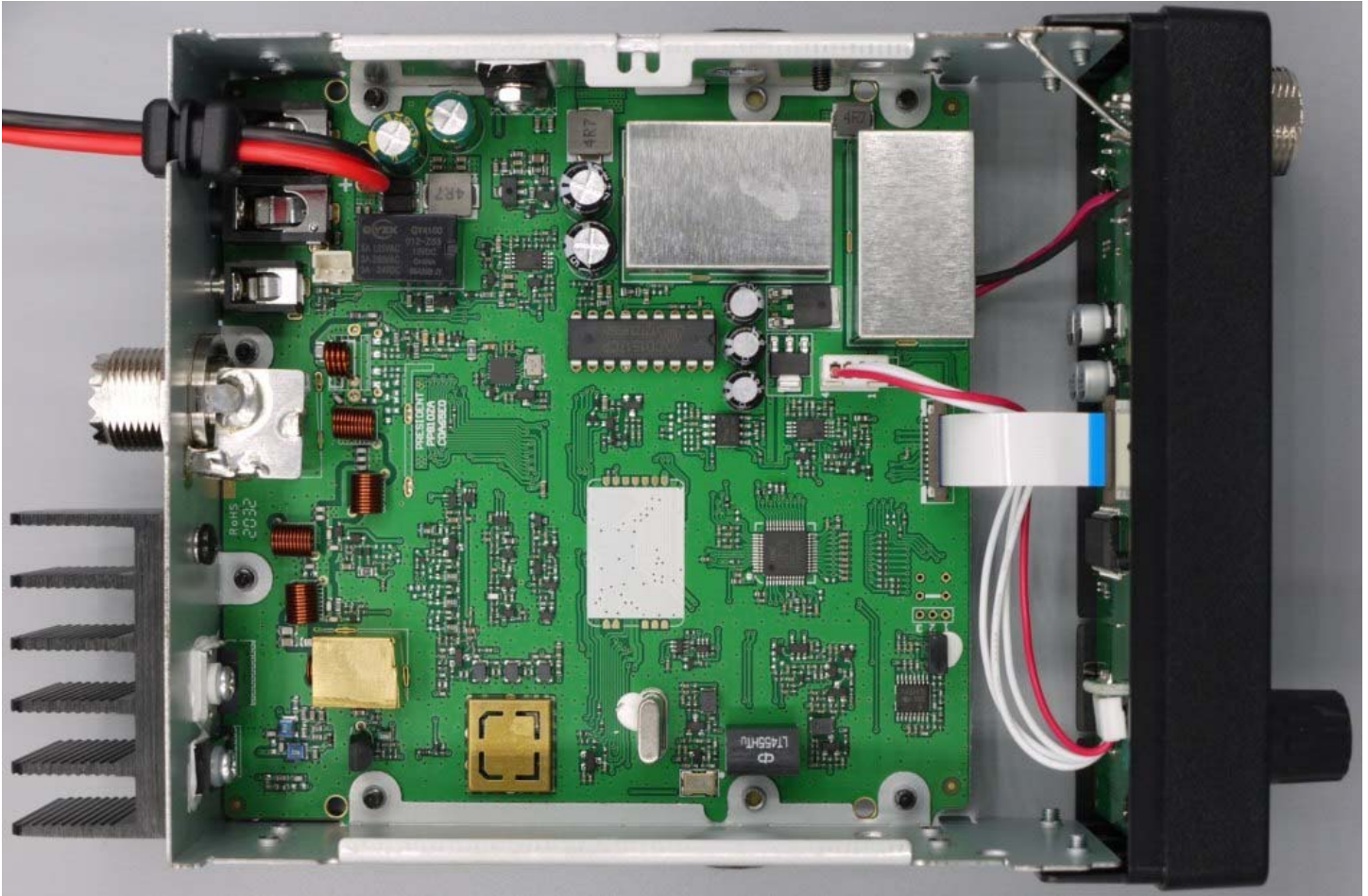
Figure E20.1 – Internal Photo – Bottom Cover Removed
