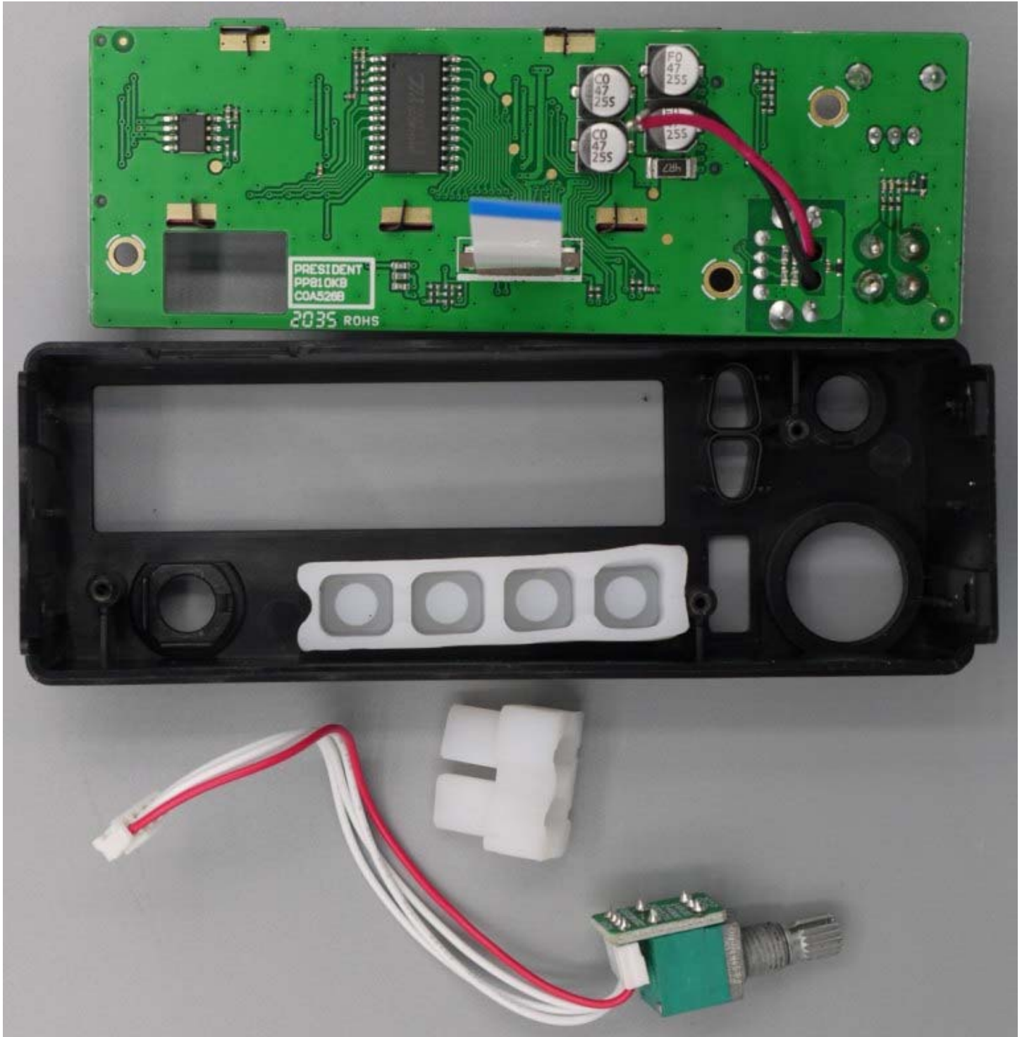
Figure E20.5 – Internal Photo – Front Assembly – Rear View
