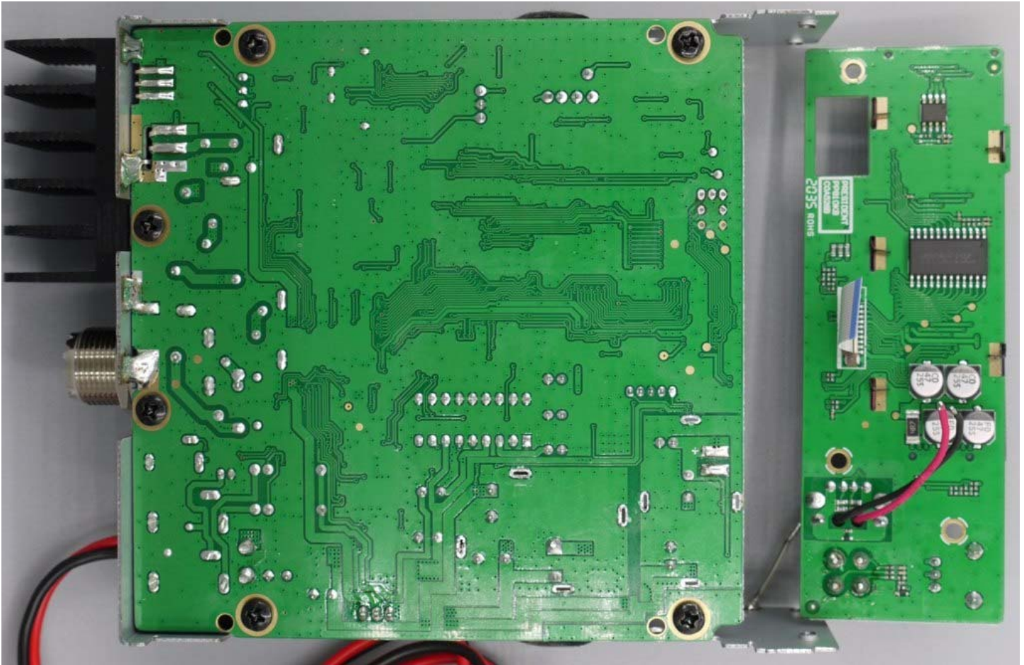
Figure E20.3 – Internal Photo – Top Cover & Front Removed
