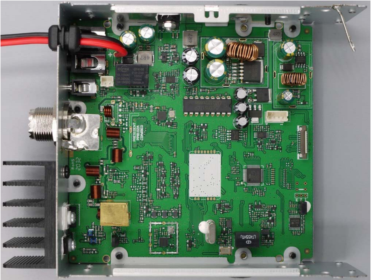
Figure E20.2 – Internal Photo – Bottom Cover/Front & Shields Removed
