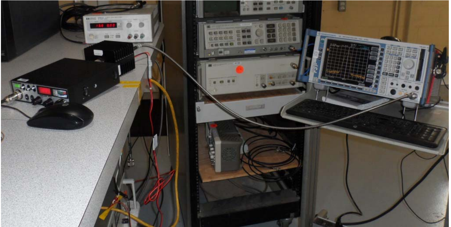
Figure E22.1 – Setup Photo – Conducted Measurements
