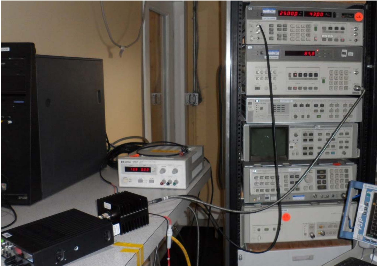
Figure E22.2 – Setup Photo – Audio Response Measurements
