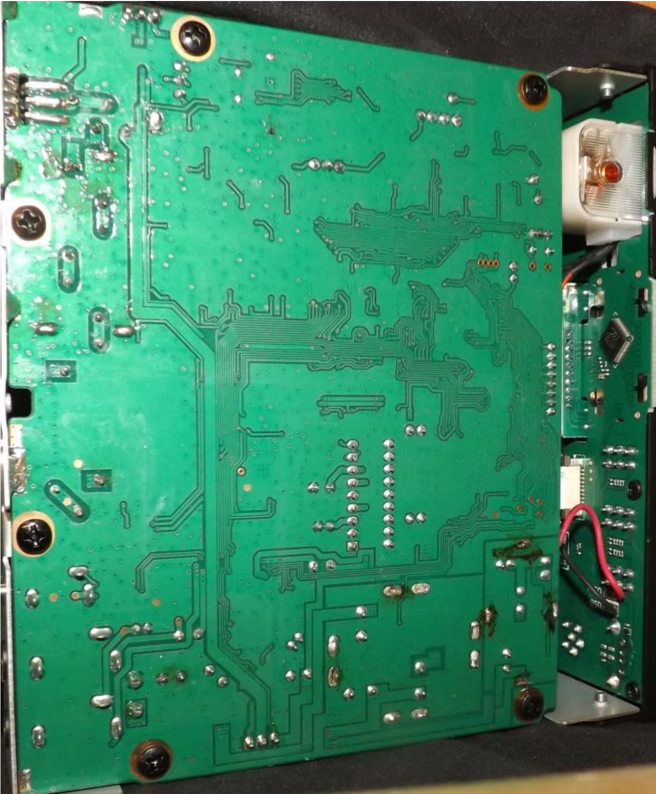
Figure E21.4 – Internal Photo – PCB Bottom Side
