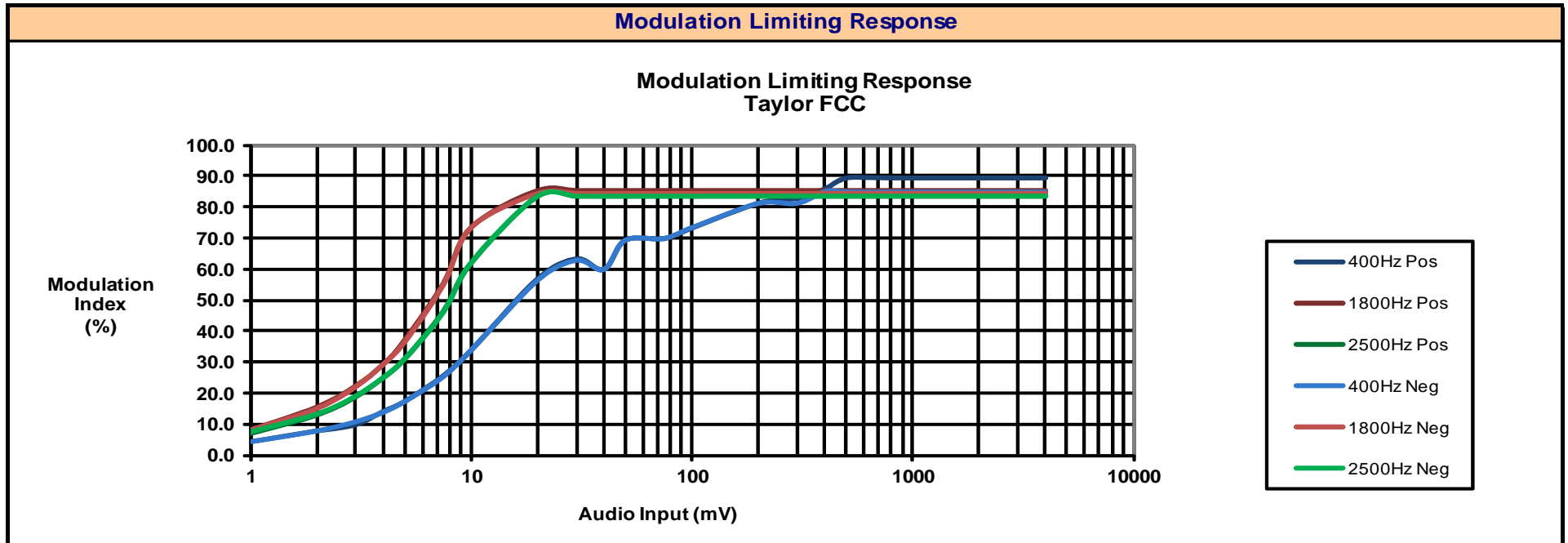
Plot 8.2 – Modulation Limiting Response
