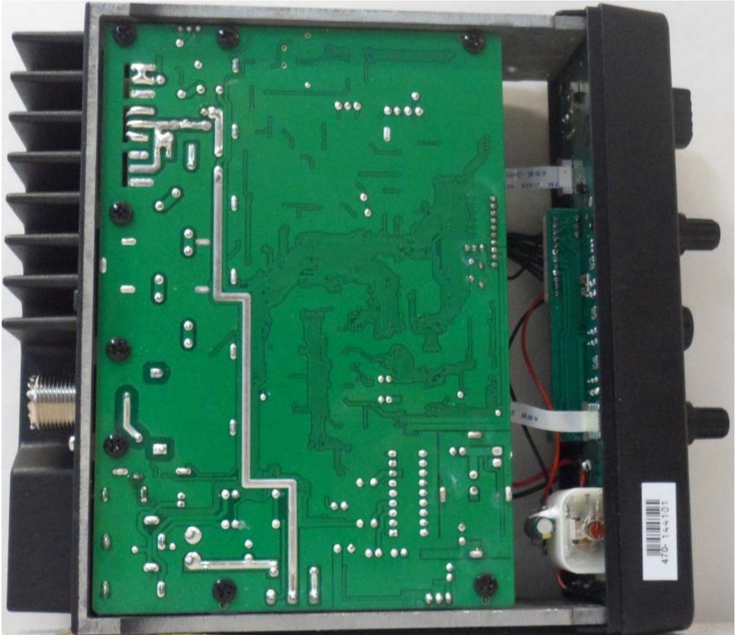
Figure E19.1 – Internal Photo – Main PCB - Bottom
