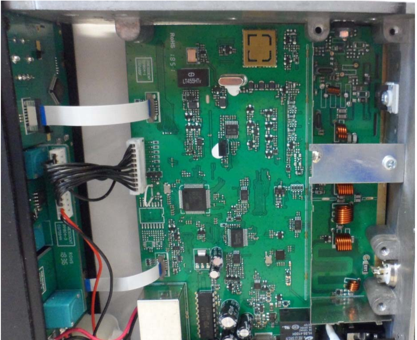
Figure E19.3 – Internal Photo – Main PCB – Top – Enlarged
