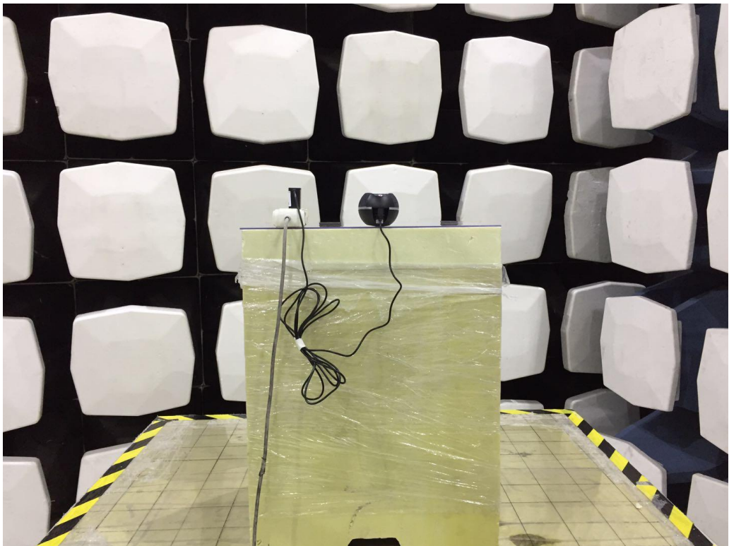
Back View of Radiated Emissions above 1GHz
