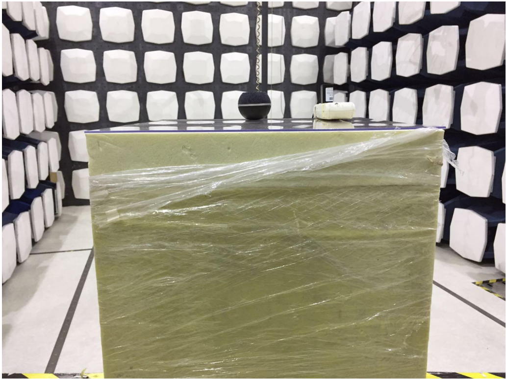
Front View of Radiated Emissions above 1GHz
