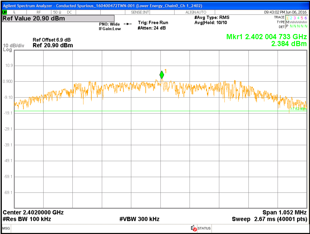
Chain0 : Conducted Spurious @ BT4.0 mode Ch low
