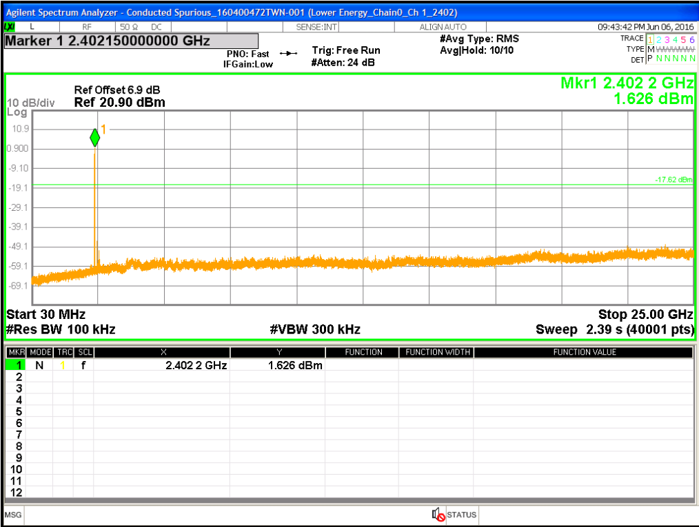
Chain0 : Conducted Spurious @ BT4.0 mode Ch low
