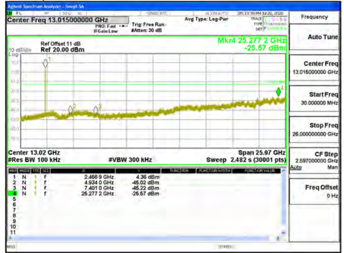
Spurious Emission_802.11b_20MHz_Chain0_2472MHz
