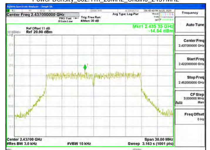
Power Density_802.11n_20MHz_Chain0_2437MHz
