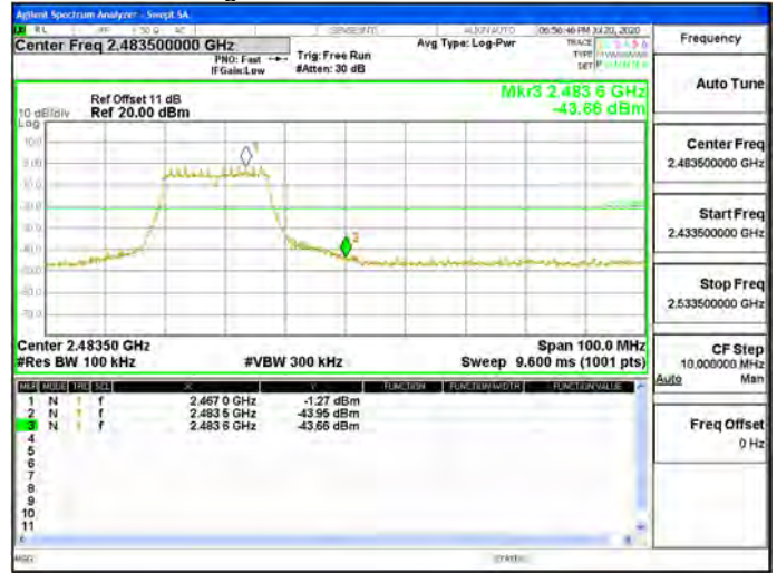
Band Edge_802.11n_20MHz_Chain0_2467MHz
