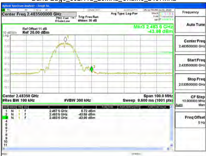
Band Edge_802.11b_20MHz_Chain0_2467MHz
