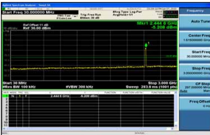
30M-3GHz Spurious Emission Test Data CH-Mid
