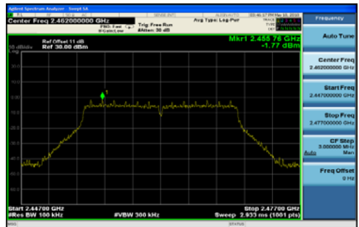
802.11g Band Edge Limit Test Data CH-High
