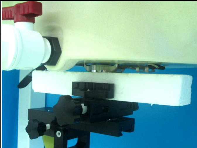
Rear Face of EUT with 0 cm Gap for Sample 2
