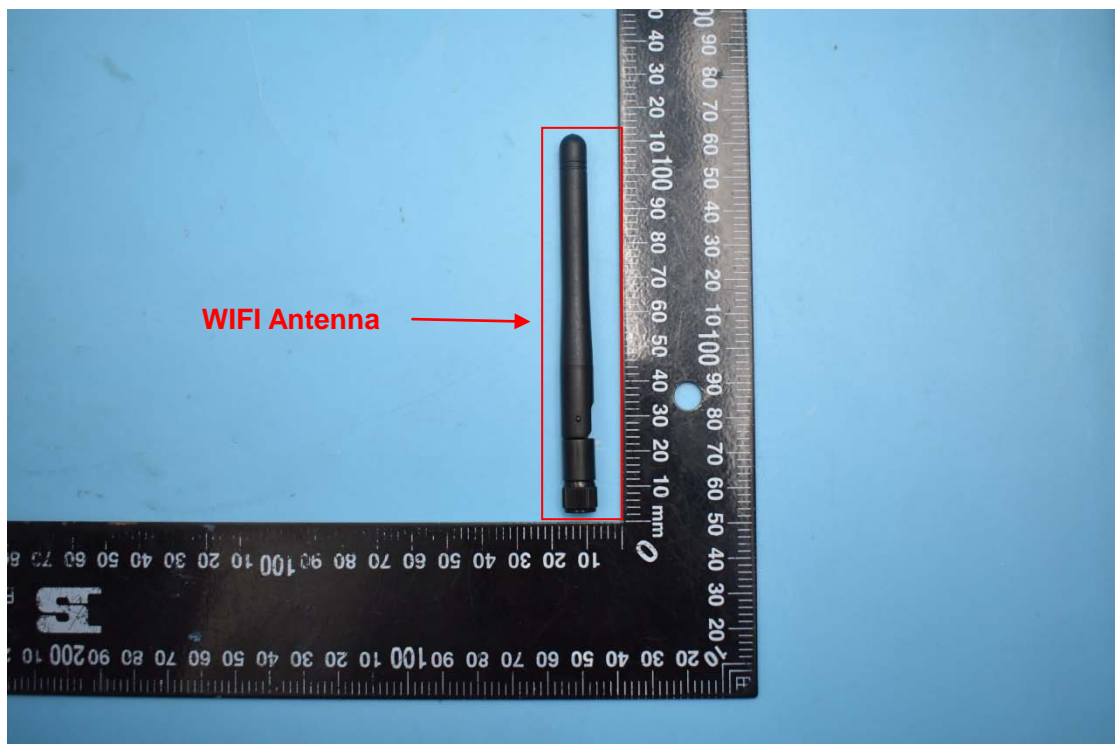
2. Antenna view
