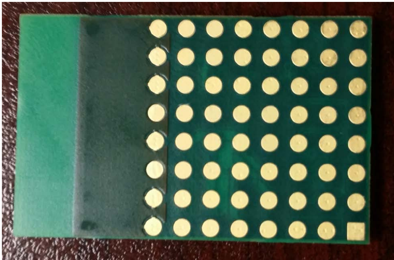
Figure 2: Bottom View
