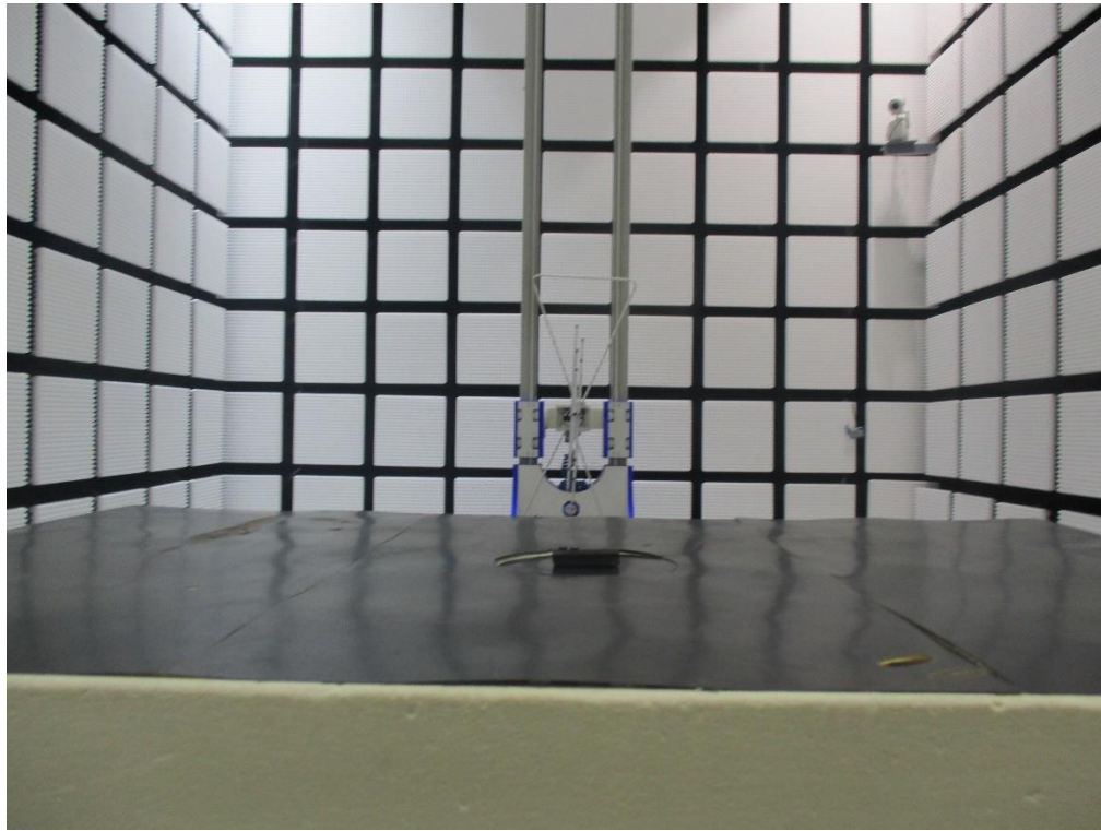
Setup photo_50126-R
